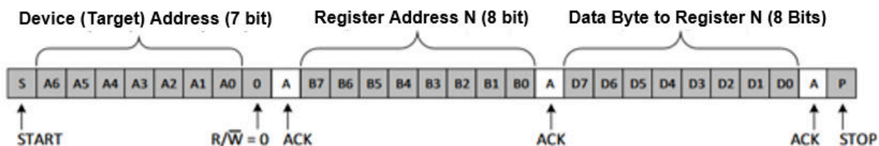
8-3. I 2 C Write Protocol
