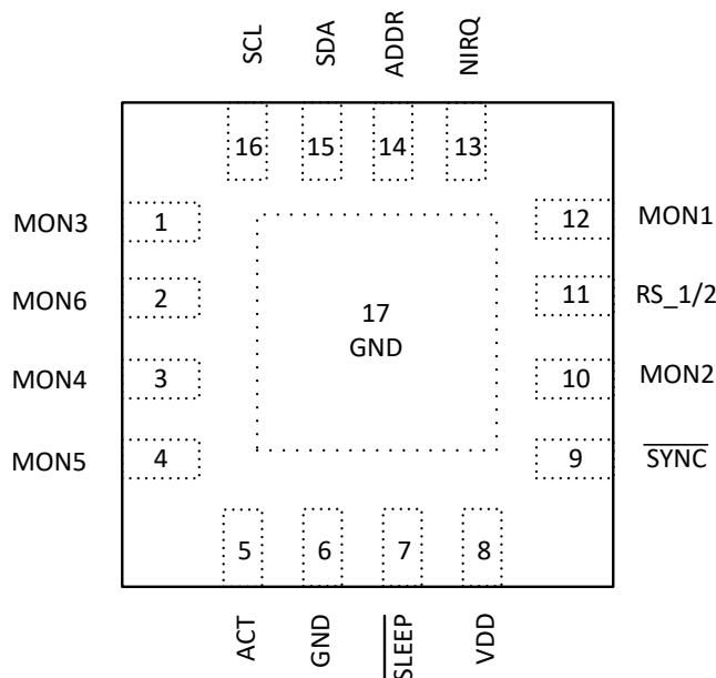
図 6-1. RTE Package 16-Pin WQFN TPS389006 Top View
