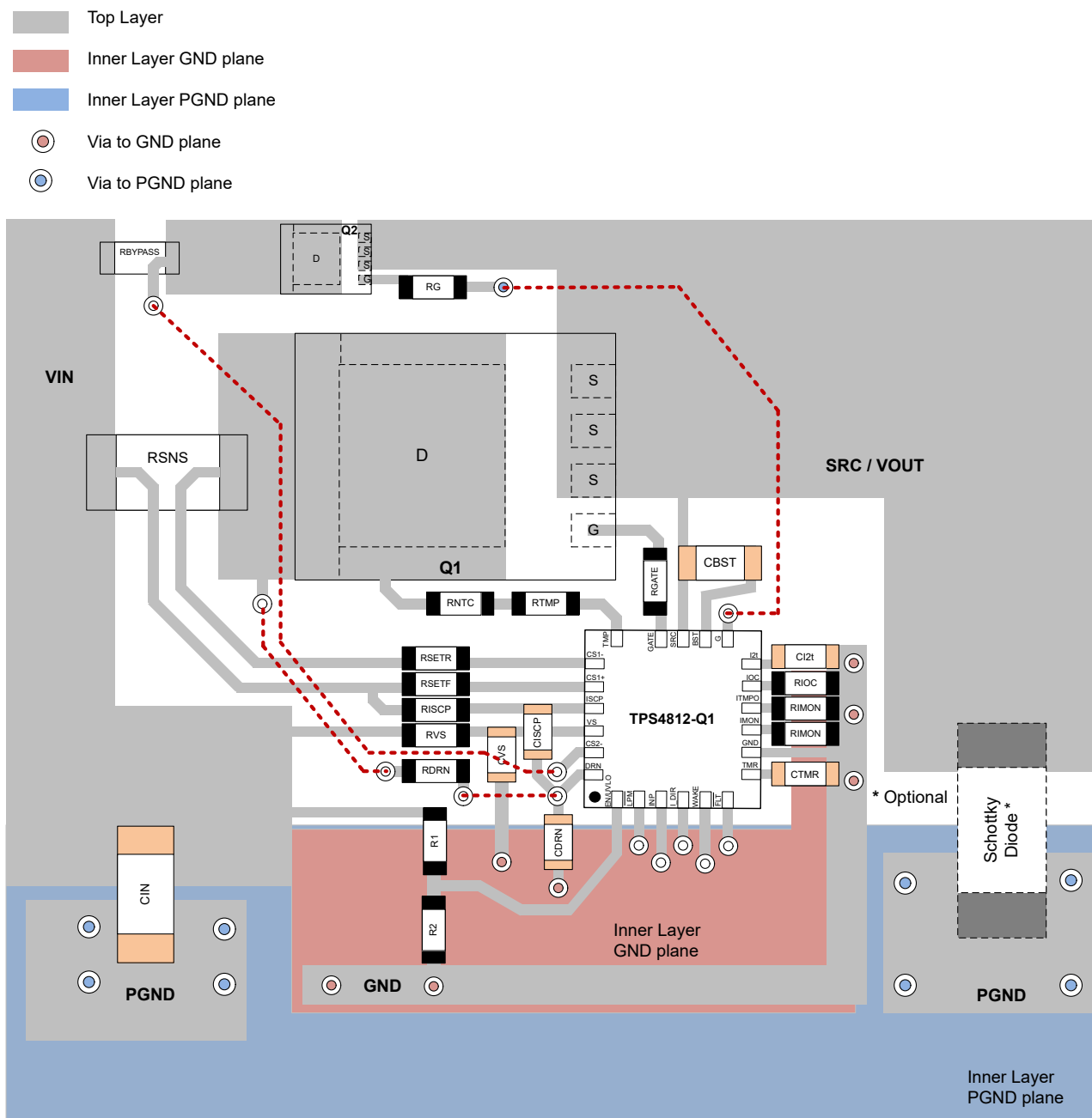
図 9-20. Typical PCB Layout Example of TPS4812-Q1
