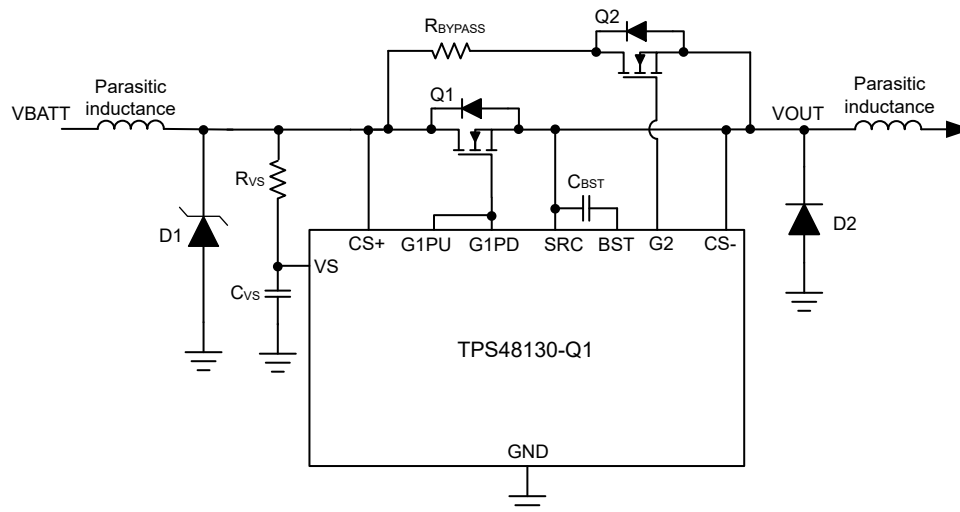
✎ 8-14. Circuit Implementation With Optional Protection Components For TPS48130-Q1
