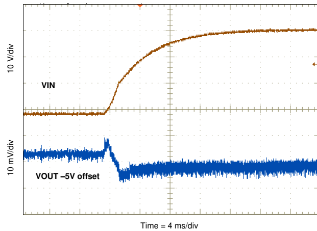
8-7. Line Transient (8 V to 40 V)
