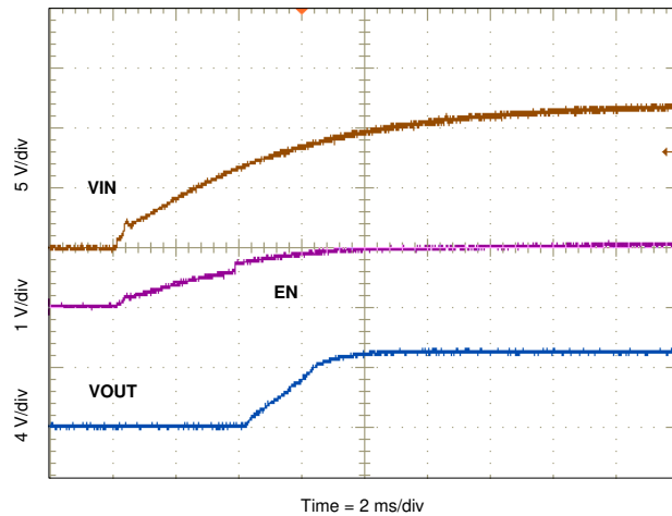
8-8. Start-up With VIN
