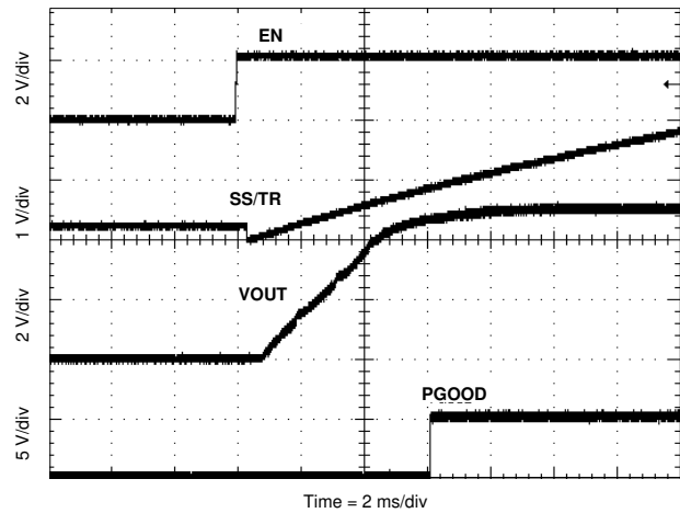
8-9. Start-up With EN
