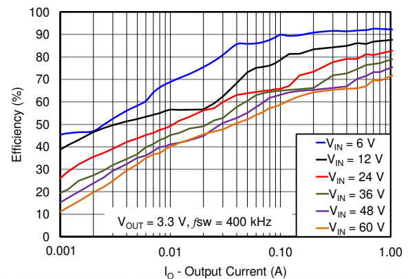
8-21. Light Load Efficiency
