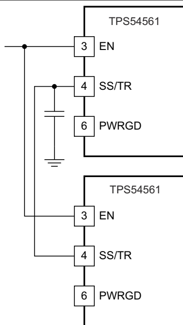
Figure 7-6. Schematic for Ratio-Metric Start-Up Sequence
