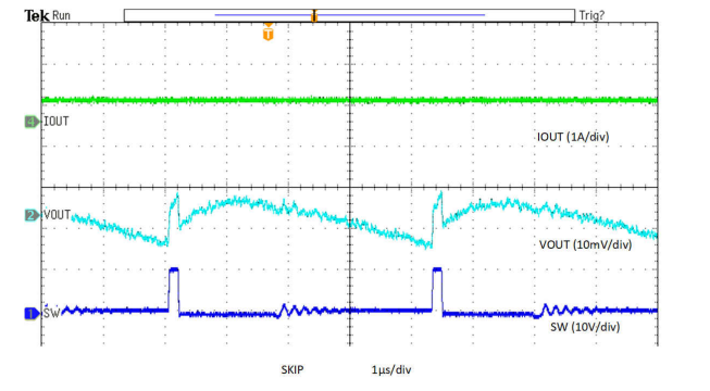
8-25. Output Voltage Ripple, Skip, 1-A Load
