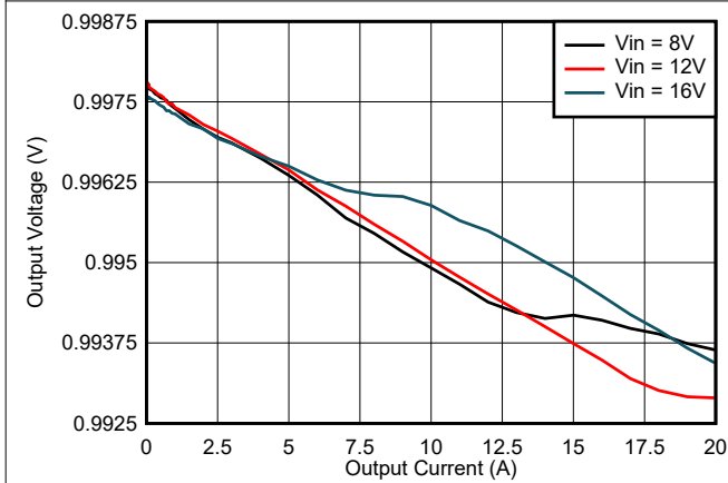
8-10. Output Voltage vs Output Current, VCC = 3.3-V External Bias, FCCM
