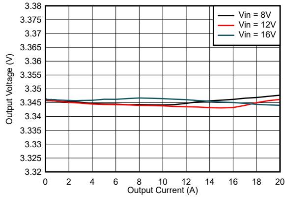
6-7. Output Voltage vs Output Current
