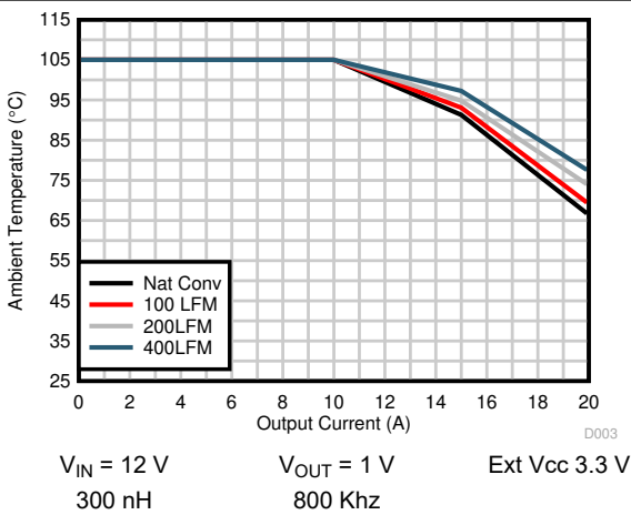
6-5. Safe Operating Area, V_{OUT} = 1 \text{ V}
