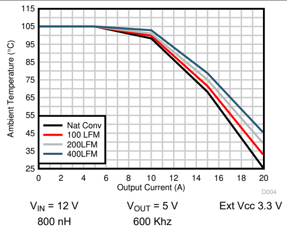
6-6. Safe Operating Area, V_{OUT} = 5 \text{ V}
