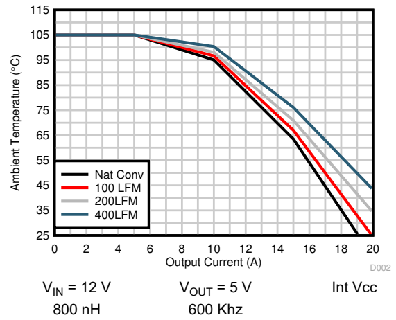
6-4. Safe Operating Area, V_{OUT} = 5 \text{ V}
