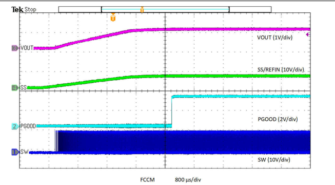
8-27. Exiting Overtemperature Protection in FCCM
