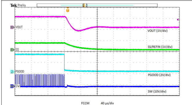
8-26. Overtemperature Protection in FCCM
