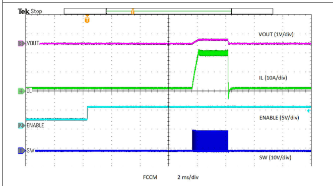
8-28. Enabled into Overcurrent
