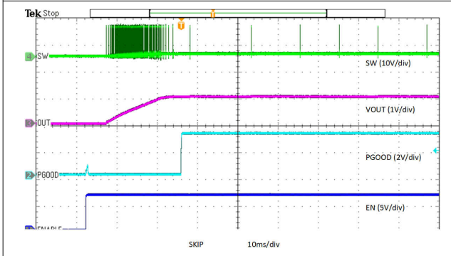
8-16. Enable Power Up, Skip
