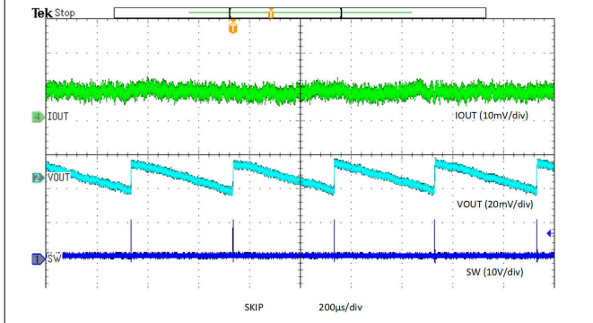
8-24. Output Voltage Ripple, Skip, 0.01-A Load
