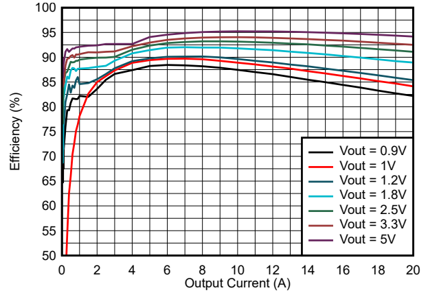
6-2. Efficiency vs Output Current, 12 V_{IN} , 800 KHz, DCM, V_{CC} = \text{EXT } 3.3 \text{ V}
