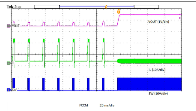
8-29. Hiccup Overcurrent
