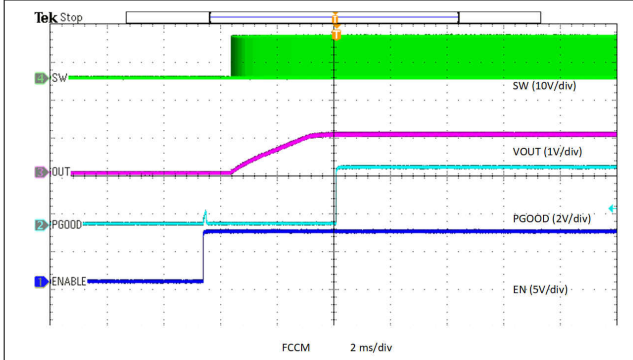
8-14. Enable Start-Up, Prebias
