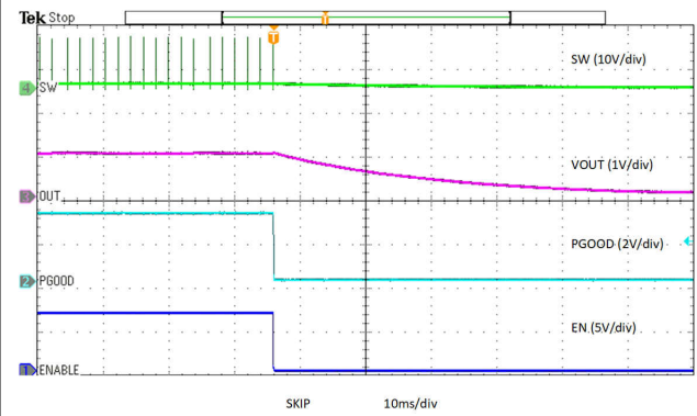
6-14. Enable Power Down, Skip
