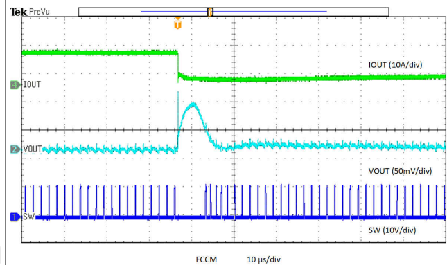
6-12. Unload Transient
