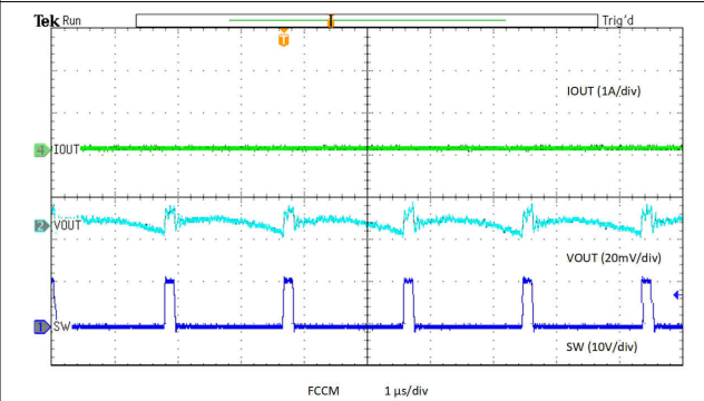
8-21. Output Voltage Ripple, FCCM, 0-A Load
