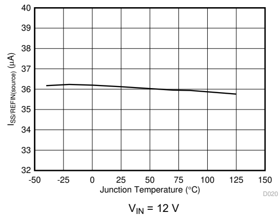
6-10. I_{SS}(\text{source}) vs Junction Temperature
