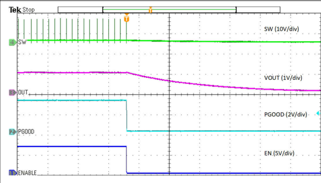
8-15. Prebias Power Down
