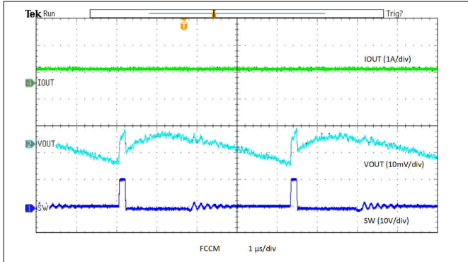
8-22. Output Voltage Ripple, FCCM, 0.5-A Load
