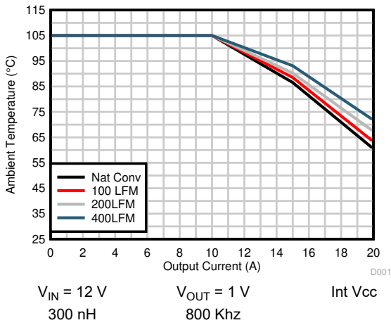
6-3. Safe Operating Area, V_{OUT} = 1.0 \text{ V}
