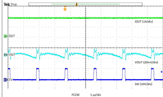
6-16. V_{OUT} Ripple, FCCM, 20-A Load
