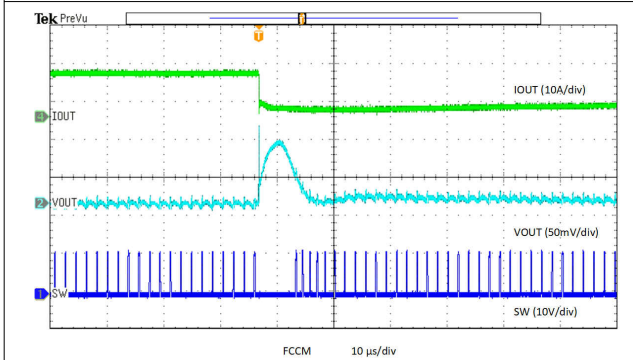
8-20. Unload Transient
