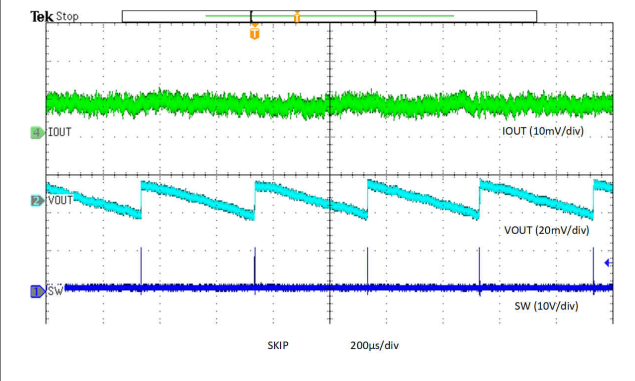
6-18. V_{OUT} Ripple, Skip Mode, 10-mA Load
