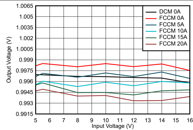
8-11. Output Voltage vs Input Voltage, Internal VCC Bias
