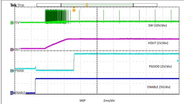
8-18. Enable Power Up into Pre-bias, Skip
