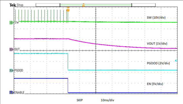
8-19. Enable Power Down with Pre-bias, Skip
