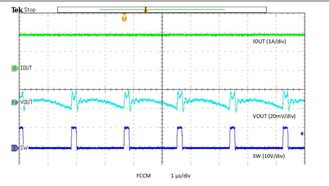
8-23. Output Voltage Ripple, FCCM, 20-A Load
