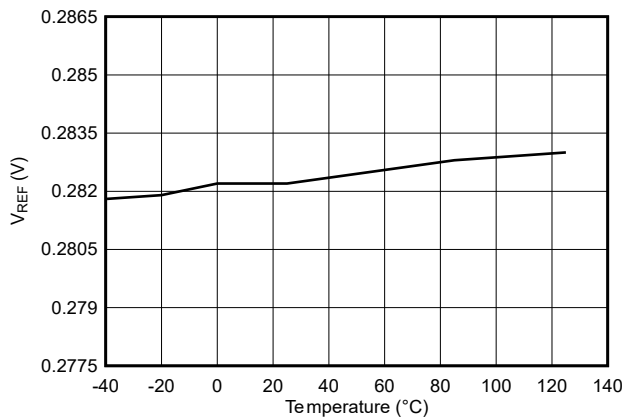
5-17. Reference Voltage vs Temperature ( V_{REF} = 0.282\text{ V} )
