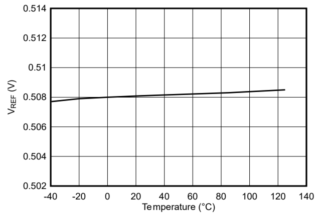
5-18. Reference Voltage vs Temperature ( V_{REF} = 0.508\text{ V} )
