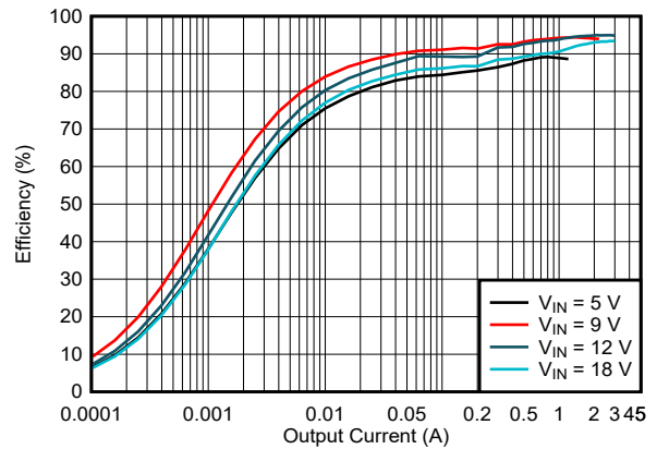
5-14. Efficiency vs Output Current, V_{OUT} = 12\text{ V} , f_{SW} = 2\text{ MHz} , PFM
