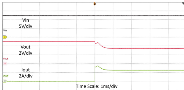
図 7-12. Output Current Limit Waveforms in V_{IN} = 12\text{ V} , V_{OUT} = 5\text{ V} , R_{LOAD} = 1.5\ \Omega , R_{SNS} = 20\text{ m}\Omega FPWM
