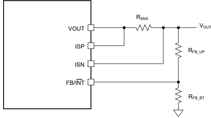
☒ 6-5. Output Voltage Setting by External Resistor Divider
