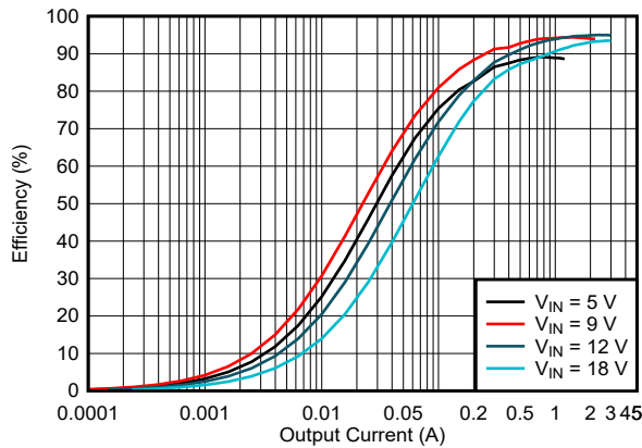
5-13. Efficiency vs Output Current, V_{OUT} = 12\text{ V} , f_{SW} = 2\text{ MHz} , FPWM
