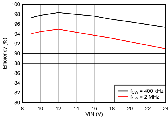
5-15. Efficiency vs Input Voltage, V_{OUT} = 12\text{ V} , I_{OUT} = 2\text{ A} , FPWM
