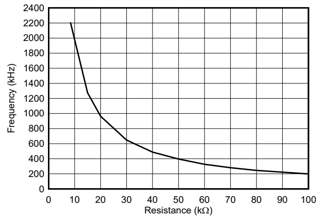
5-16. Switching Frequency vs Setting Resistance
