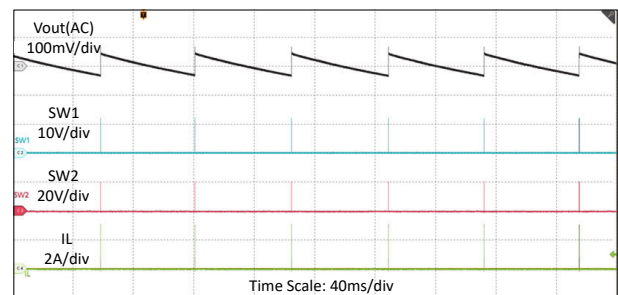
8-7. Switching Waveforms in V_{IN} = 12V , V_{OUT} = 20V , I_O = 0A , PFM
