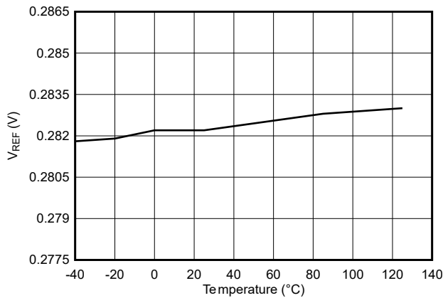
图 5-17. Reference Voltage vs Temperature ( V_{REF} = 0.282\text{ V} )
