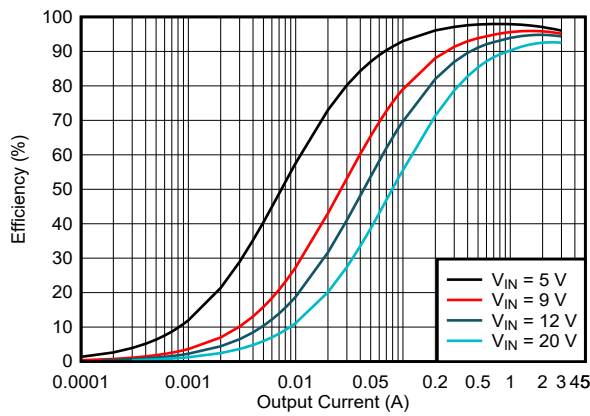
5-1. Efficiency vs Output Current, V_{OUT} = 5V , f_{SW} = 400\text{ kHz} , FPWM
