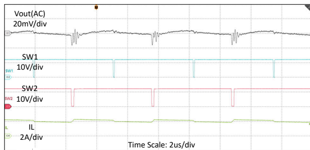
8-4. Switching Waveforms in V_{IN} = 12V , V_{OUT} = 12V , I_O = 2A , FPWM
