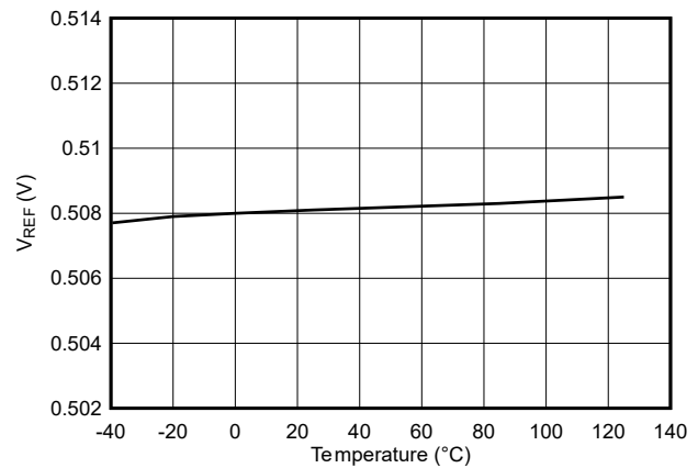
图 5-18. Reference Voltage vs Temperature ( V_{REF} = 0.508\text{ V} )
