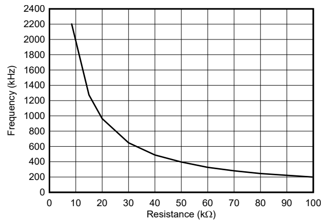
图 5-16. Switching Frequency vs Setting Resistance
