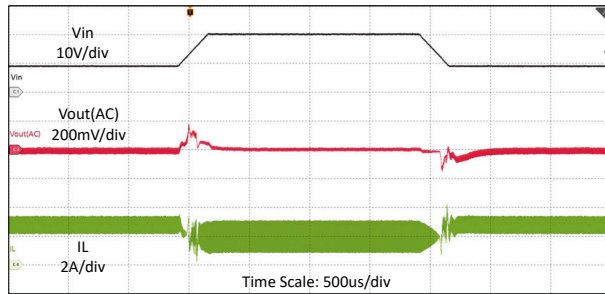
8-10. Line Transient Waveforms in V_{IN} = 9V to 20V , V_{OUT} = 12V , I_O = 2A with 200\mu s Slew Rate, FPWM
