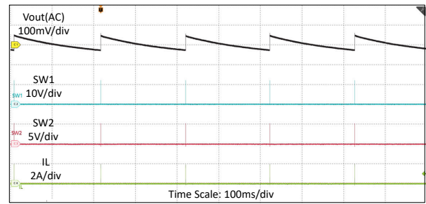
8-3. Switching Waveforms in V_{IN} = 12V , V_{OUT} = 5V , I_O = 0A , PFM
