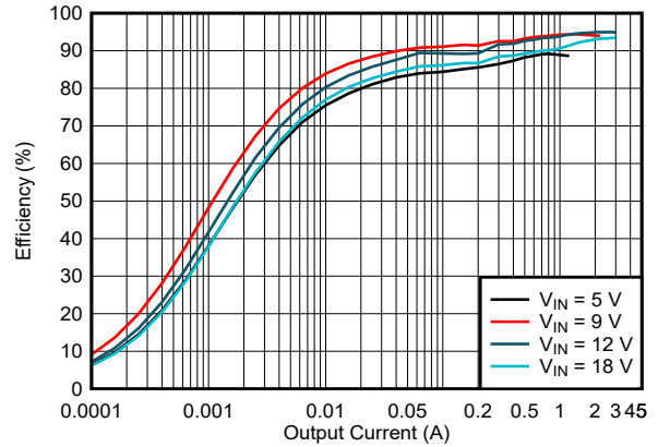
图 5-14. Efficiency vs Output Current, V_{OUT} = 12\text{ V} , f_{SW} = 2\text{ MHz} , PFM
