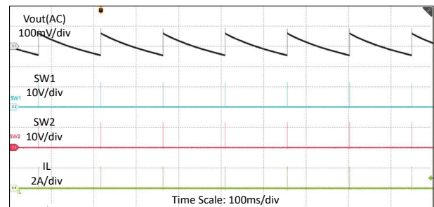
8-5. Switching Waveforms in V_{IN} = 12V , V_{OUT} = 12V , I_O = 0A , PFM
