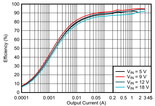
図 5-12. Efficiency vs Output Current, V_{OUT} = 9V , f_{SW} = 2\text{ MHz} , PFM
