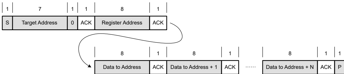
Figure 6-13. Multi-byte Write
