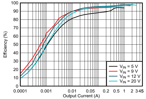
図 5-8. Efficiency vs Output Current, V_{OUT} = 15V , f_{SW} = 400\text{ kHz} , PFM
