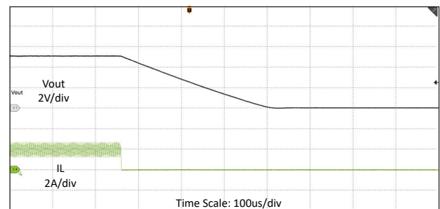
8-9. Shutdown Waveforms in V_{IN} = 12V , V_{OUT} = 5V , R_{LOAD} = 2.5\Omega , FPWM
