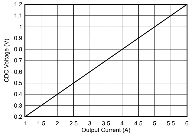
図 5-25. CDC Voltage vs Output Current with R_{SENSE} = 10m\Omega
