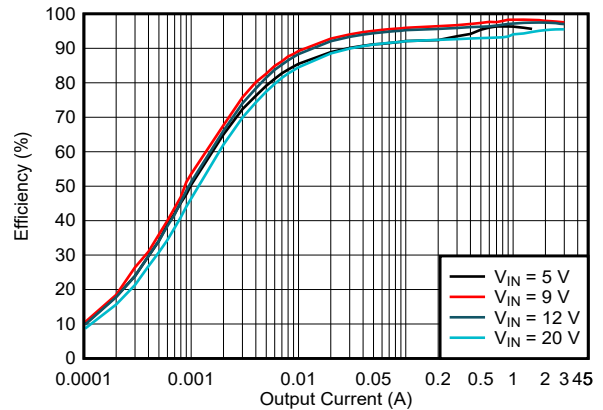
5-4. Efficiency vs Output Current, V_{OUT} = 9V , f_{SW} = 400\text{ kHz} , PFM
