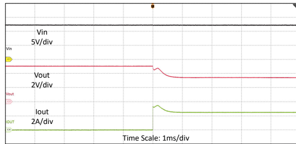
8-12. Output Current Limit Waveforms in V_{IN} = 12V , V_{OUT} = 5V , R_{LOAD} = 1.5\Omega , R_{SNS} = 20m\Omega FPWM
