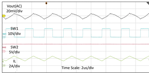
8-2. Switching Waveforms in V_{IN} = 12V , V_{OUT} = 5V , I_O = 2A , FPWM
