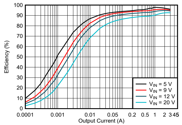
5-2. Efficiency vs Output Current, V_{OUT} = 5V , f_{SW} = 400\text{ kHz} , PFM
