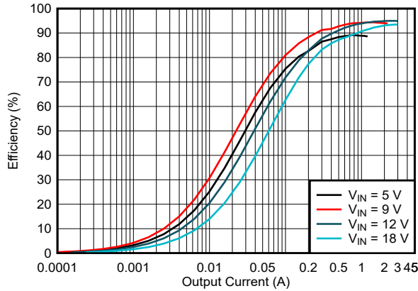
图 5-13. Efficiency vs Output Current, V_{OUT} = 12\text{ V} , f_{SW} = 2\text{ MHz} , FPWM
