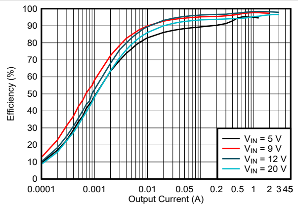
5-6. Efficiency vs Output Current, V_{OUT} = 12V , f_{SW} = 400\text{ kHz} , PFM
