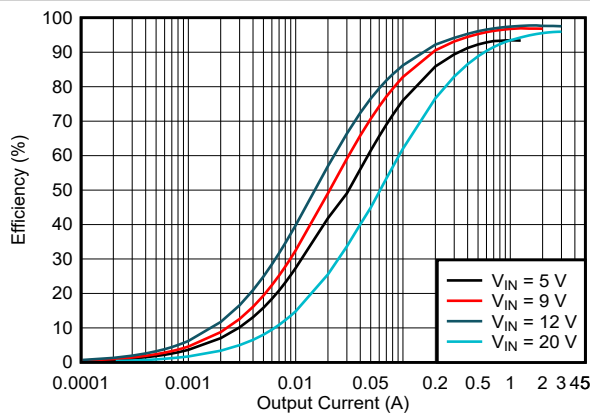
5-5. Efficiency vs Output Current, V_{OUT} = 12V , f_{SW} = 400\text{ kHz} , FPWM
