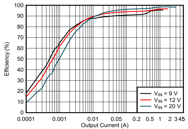
図 5-10. Efficiency vs Output Current, V_{OUT} = 20V , f_{SW} = 400\text{ kHz} , PFM
