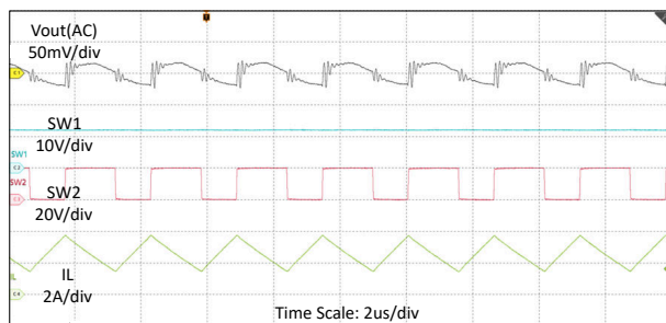
8-6. Switching Waveforms in V_{IN} = 12V , V_{OUT} = 20V , I_O = 1.5A , FPWM
