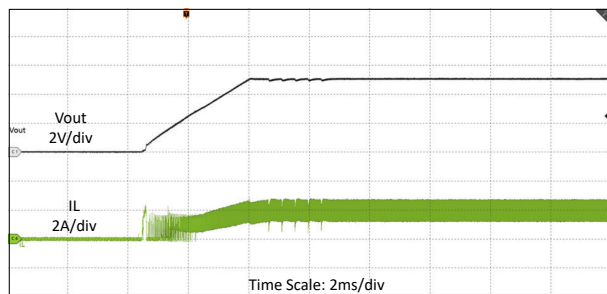
8-8. Start-up Waveforms in V_{IN} = 12V , V_{OUT} = 5V , R_{LOAD} = 2.5\Omega , FPWM
