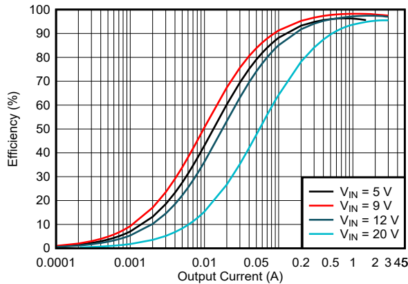
5-3. Efficiency vs Output Current, V_{OUT} = 9V , f_{SW} = 400\text{ kHz} , FPWM
