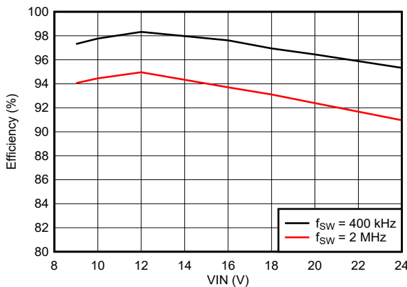
图 5-15. Efficiency vs Input Voltage, V_{OUT} = 12\text{ V} , I_{OUT} = 2\text{ A} , FPWM
