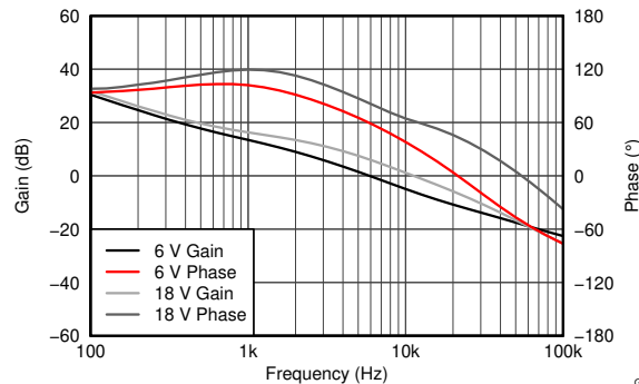
9-16. Closed Loop Gain and Phase of the SEPIC Converter
