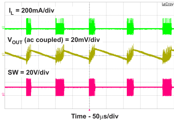
9-7. Pulse Skipping
