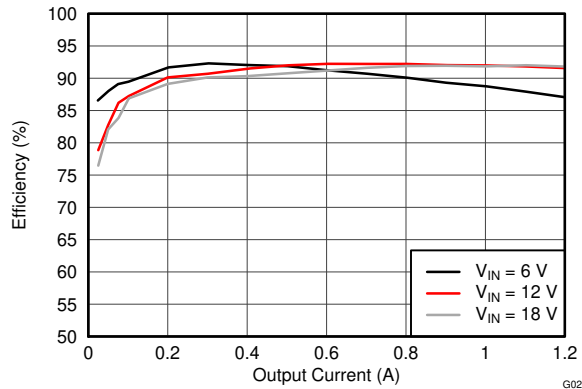
9-12. Efficiency vs Output Current
