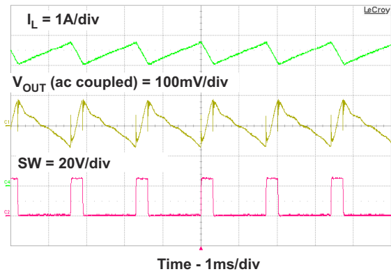
9-5. CCM PWM Operation
