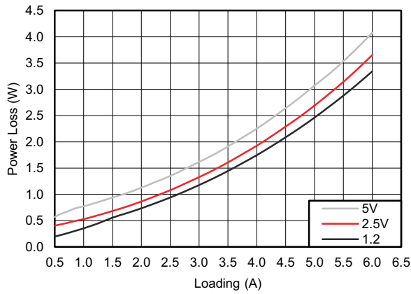
10-1. Power Dissipation of TPS55340-EP
