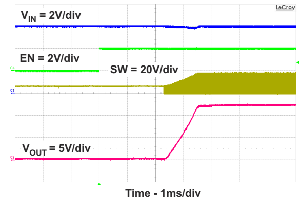
9-15. Output Voltage Soft-Start
