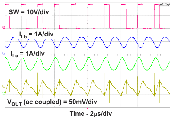
9-14. CCM PWM Operation
