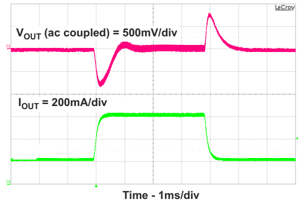
9-4. Load Transient Response
