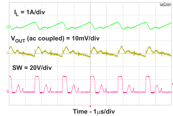
9-6. DCM PWM Operation
