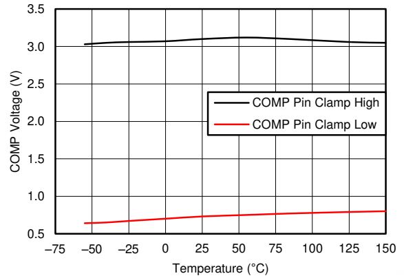
7-8. COMP Clamp Voltage vs Temperature
