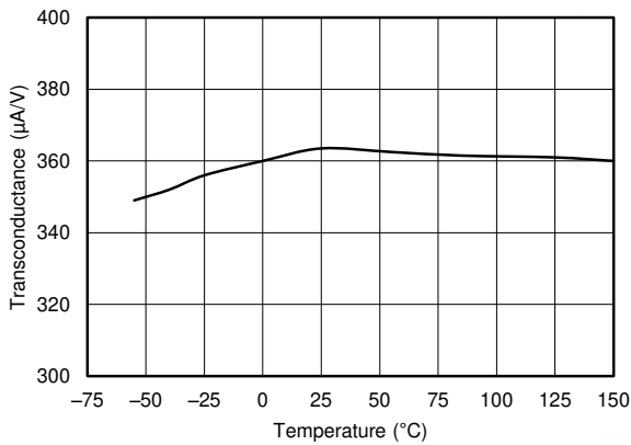
7-1. Error Amplifier Transconductance vs Temperature
