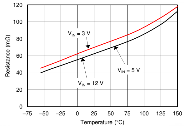
7-4. R DS(ON) vs Temperature
