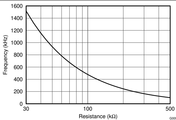
7-5. Frequency vs FREQ Resistance
