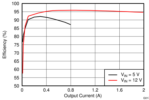
9-3. Efficiency vs Output Current
