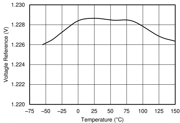
7-3. Feedback Voltage Reference vs Temperature
