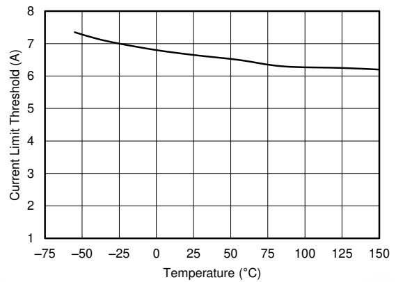
7-2. Switch Current Limit vs Temperature
