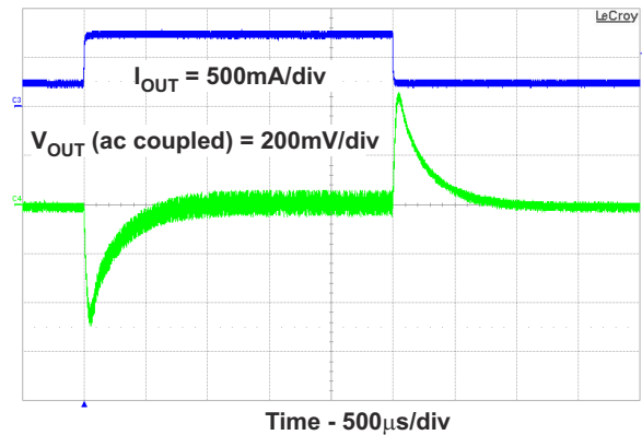
9-13. Load Transient Response
