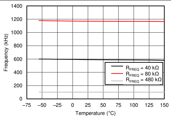
7-6. Frequency vs Temperature
