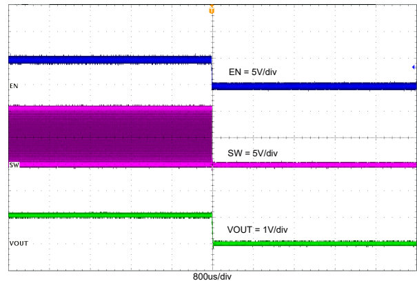
7-7. TPS561243 Enable Off With 1A Loading
