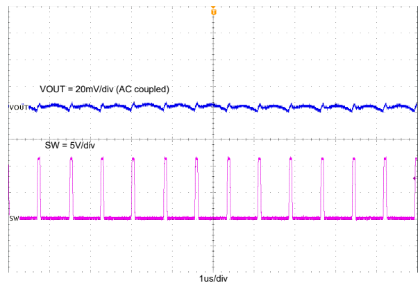
7-5. TPS561246 Output Voltage Ripple With 1A Loading
