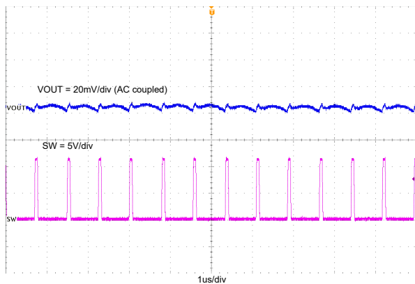
7-4. TPS561243 Output Voltage Ripple With 1A Loading
