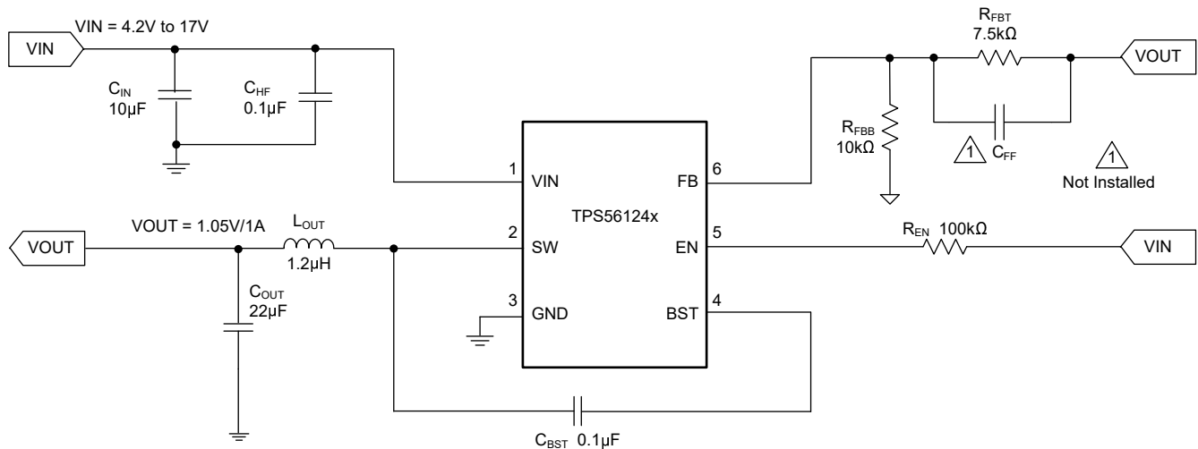
図 7-1. TPS56124x 1.05V/1A Reference Design
