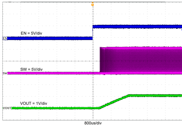
7-6. TPS561243 Enable On With 1A Loading
