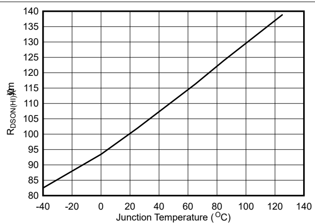
Figure 5-6. High-Side R_{dson}
