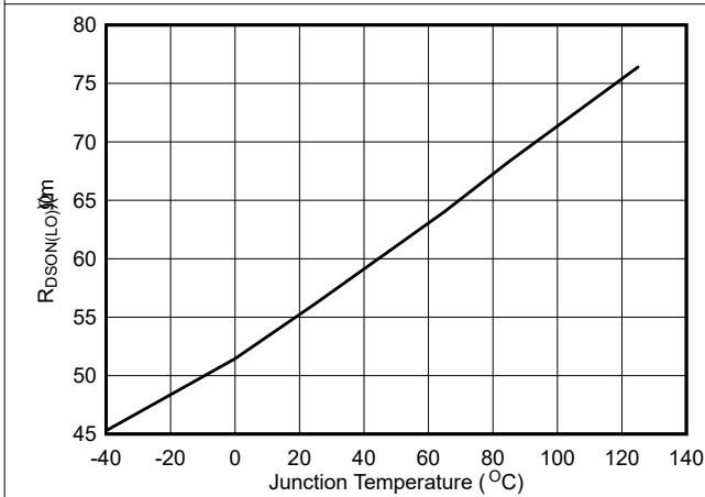
Figure 5-5. Low-Side R_{dson}
