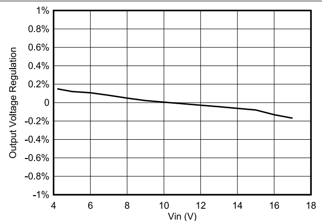
7-7. TPS562206 Line Regulation vs Vin at 1A Loading
