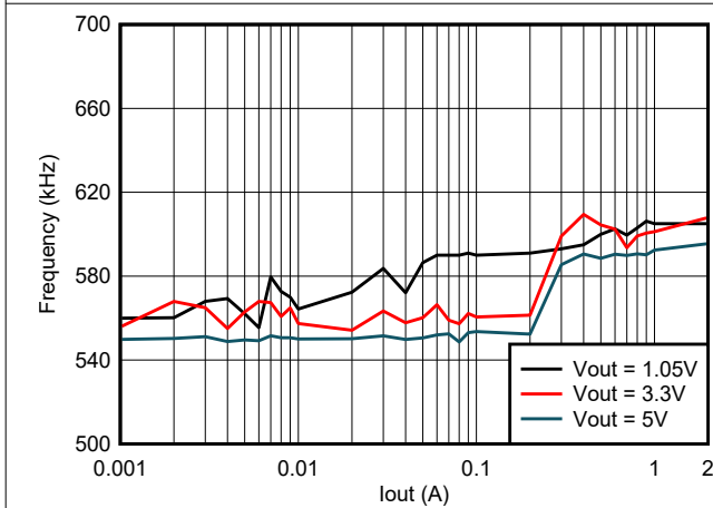
5-9. TPS562206 Frequency vs Loading
