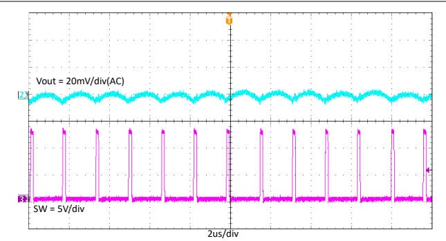
7-9. TPS562206 Output Voltage Ripple With 0.1A Loading
