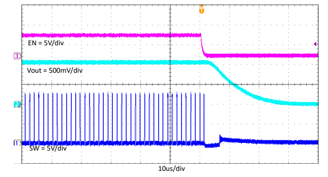
7-13. TPS562203 Enable Off With 2A Loading
