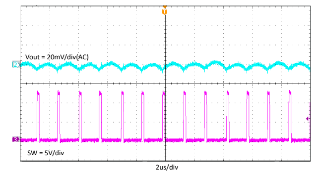
7-11. TPS562206 Output Voltage Ripple With 2A Loading
