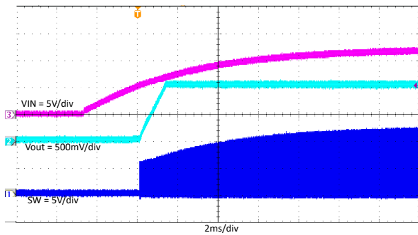
7-16. TPS562203 Power On With 2A Loading
