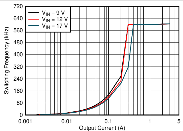
6-12. Switching Frequency vs Output Current, V OUT = 3.3 V, L = 3.3 μH
