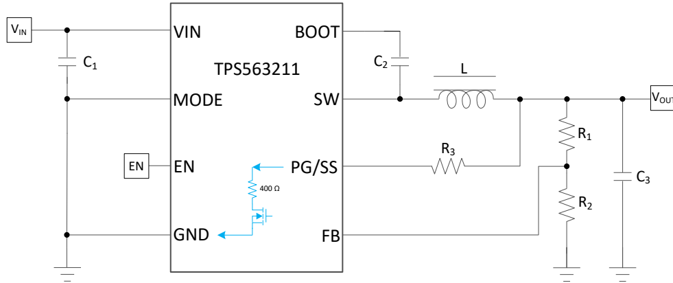
7-2. Discharge VOUT through PG/SS Pin with TPS563211
