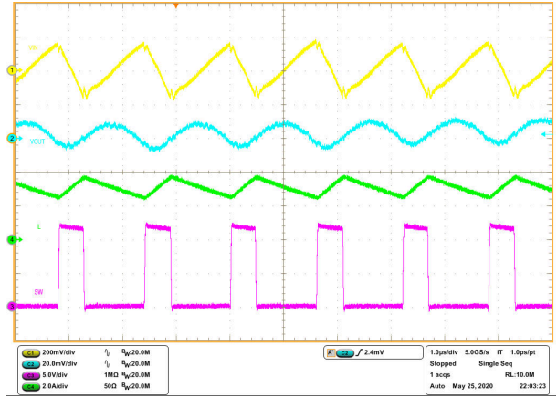
Fig 8-9. Steady State Waveforms, I_{OUT} = 3 \text{ A}
