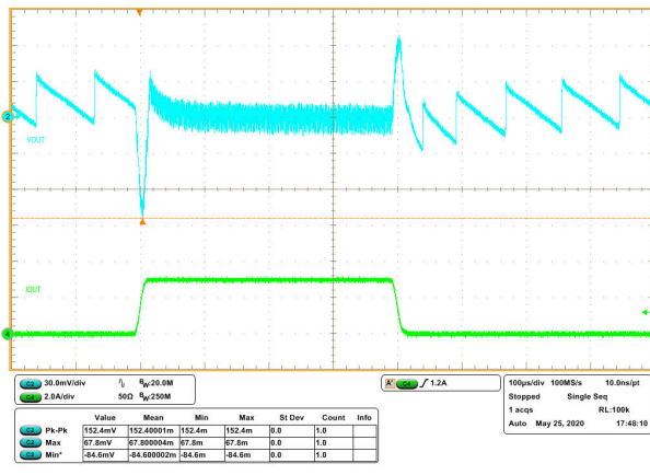
Fig 8-10. Transient Response 0 to 3 A with Slew Rate of 0.25 \text{ A}/\mu\text{s} (Eco-Mode)
