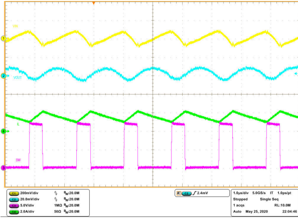
Fig 8-8. Steady State Waveforms, I_{OUT} = 1.5 \text{ A}
