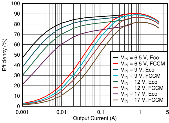
6-13. V_{OUT} = 1.05\text{-V} Efficiency, L = 1.5\ \mu\text{H}
