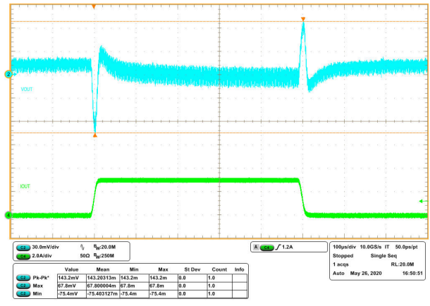
Fig 8-11. Transient Response 0 to 3 A with Slew Rate of 0.25 \text{ A}/\mu\text{s} (FCCM)
