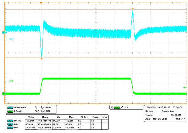
Fig 8-13. Transient Response 0.03 to 3 A with Slew Rate of 0.25 \text{ A}/\mu\text{s} (FCCM)
