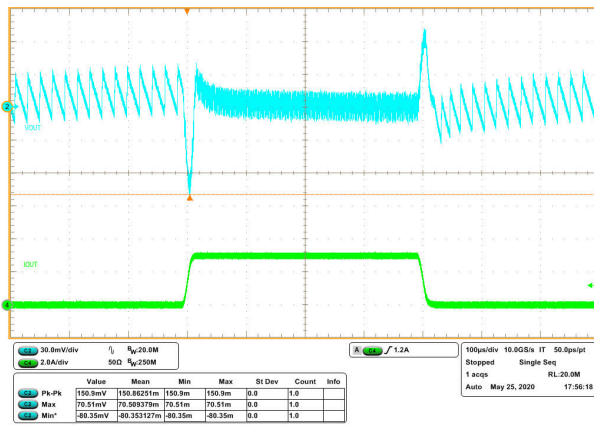
Fig 8-12. Transient Response 0.03 to 3 A with Slew Rate of 0.25 \text{ A}/\mu\text{s} (Eco-Mode)
