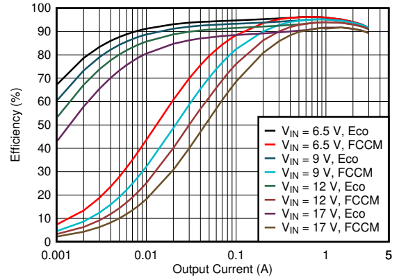
6-14. V_{OUT} = 3.3\text{-V} Efficiency, L = 3.3\ \mu\text{H}
