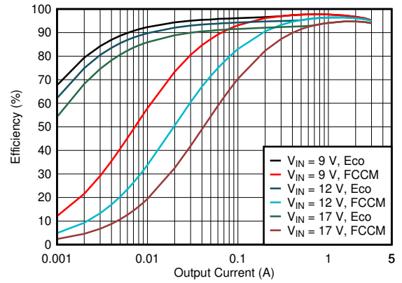
6-16. V_{OUT} = 7\text{-V} Efficiency, L = 4.7\ \mu\text{H}
