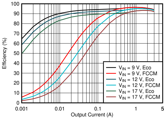
6-15. V_{OUT} = 5\text{-V} Efficiency, L = 4.7\ \mu\text{H}
