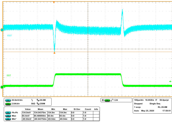
8-14. Transient Response 0.3 to 2.7 A with Slew Rate of 0.25 A/ \mu s
