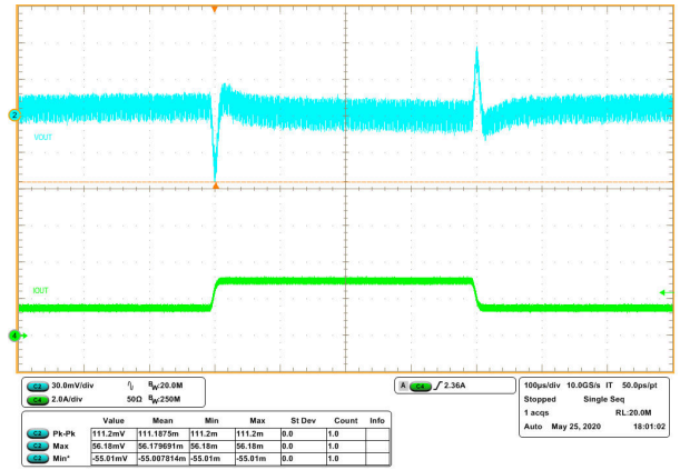
8-15. Transient Response 1.5 to 3 A with Slew Rate of 0.25 A/ \mu s
