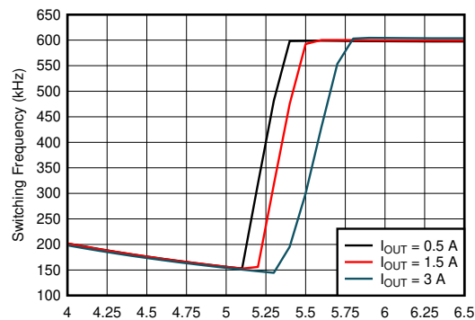
图 7-4. Frequency Foldback at Dropout ( V_{OUT} = 5 V)
