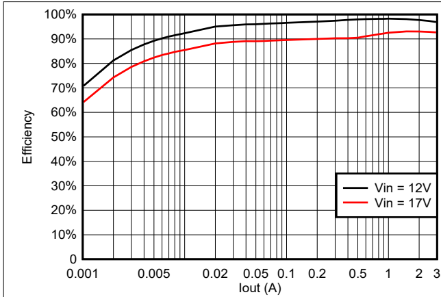
6-19. TPS563252 Efficiency at 10 V_{OUT} with a 4.7- \mu\text{H} Inductor
