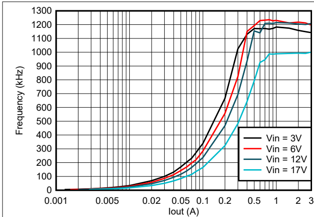
8-2. TPS563252 Frequency vs Loading
