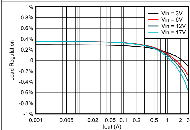
8-4. TPS563252 Load Regulation vs Loading
