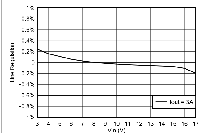
8-6. TPS563252 Line Regulation vs V_{IN}
