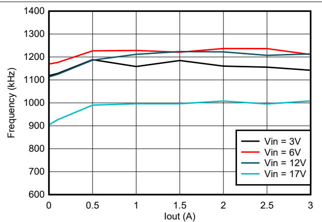
8-3. TPS563257 Frequency vs Loading
