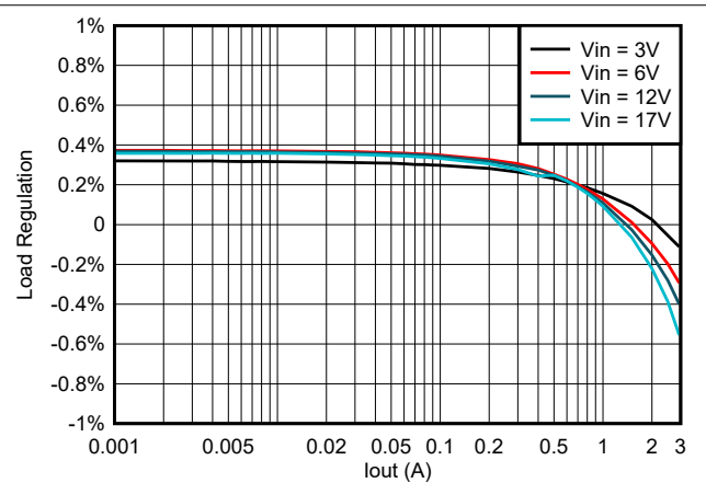
8-5. TPS563257 Load Regulation vs Loading
