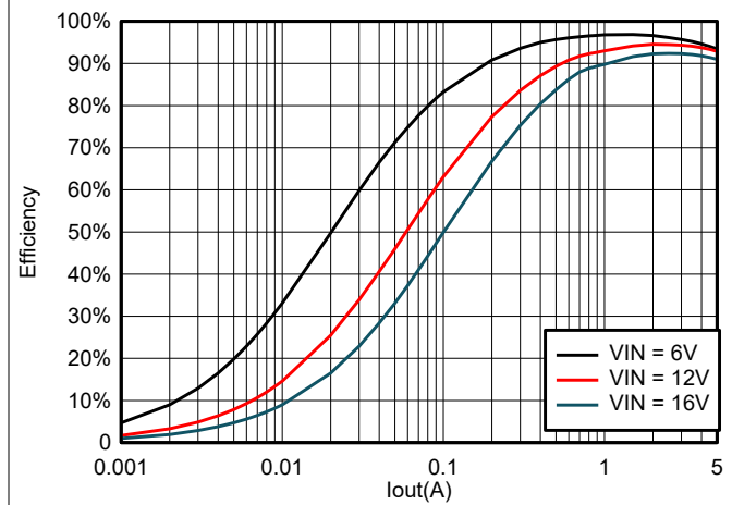
6-16. TPS565247 Efficiency at 3.3 V_{OUT} with a 2.2- \mu\text{H} Inductor
