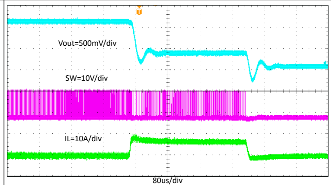
8-19. TPS565242 Normal Operation to Output Hard Short
