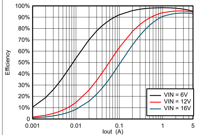
6-18. TPS565247 Efficiency at 5 V_{OUT} with a 2.2- \mu\text{H} Inductor
