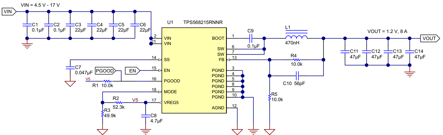
図 8-1. Application Schematic
