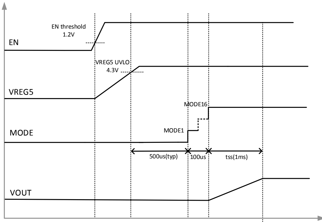
☒ 7-1. Power-Up Sequence
