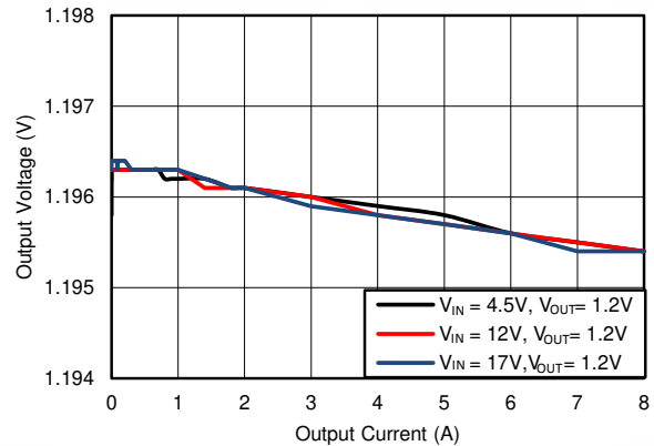
6-16. Load Regulation, F_{SW} = 400\text{kHz}
