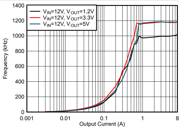
6-36. f_{SW} Load Regulation, Mode = DCM, f_{SW} = 1200\text{ kHz}
