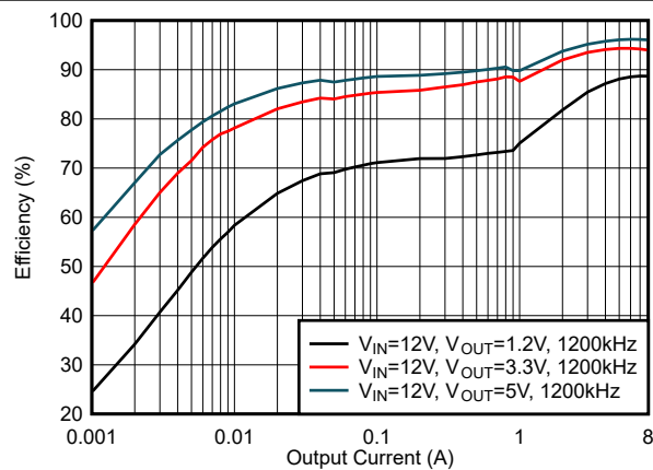
6-21. Efficiency, Mode = DCM, f_{SW} = 1200\text{ kHz}
