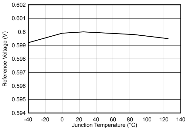
6-3. Reference Voltage vs Temperature
