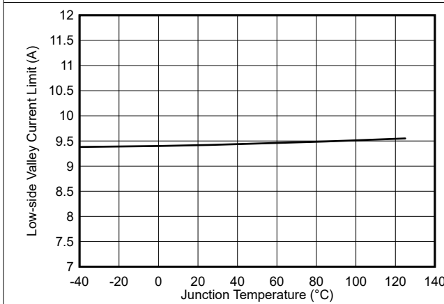
6-9. TPS568231 Current Limit (ILIM) vs Temperature
