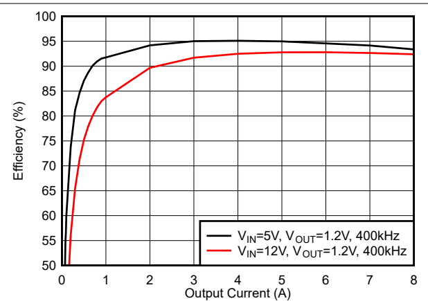
6-12. Efficiency, Mode = FCCM, f_{SW} = 400\text{ kHz}
