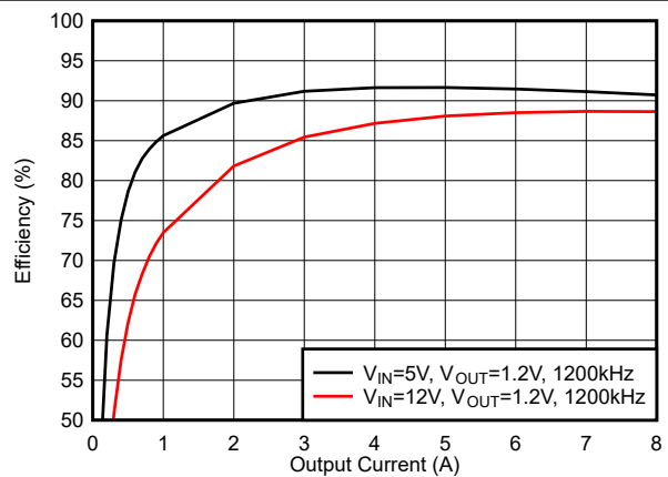
6-22. Efficiency, Mode = FCCM, f_{SW} = 1200\text{ kHz}
