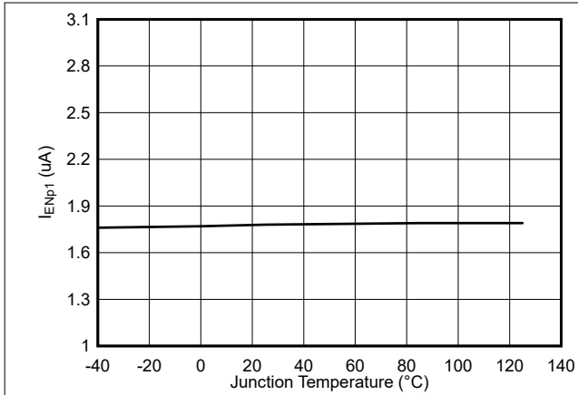
6-7. Enable Pullup Current, V_{EN} = 1\text{ V}
