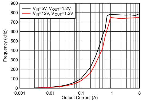
6-26. f_{SW} Load Regulation, Mode = DCM, f_{SW} = 800\text{ kHz}
