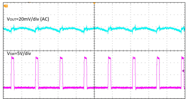
8-5. Output Voltage Ripple, I_{OUT} = 8\text{ A} , Time = 1\ \mu\text{S/div}
