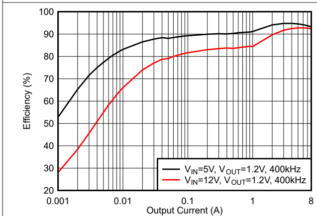
6-11. Efficiency, Mode = DCM, f_{SW} = 400\text{ kHz}
