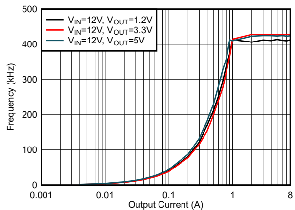
6-34. f_{SW} Load Regulation, Mode = DCM, f_{SW} = 400\text{ kHz}
