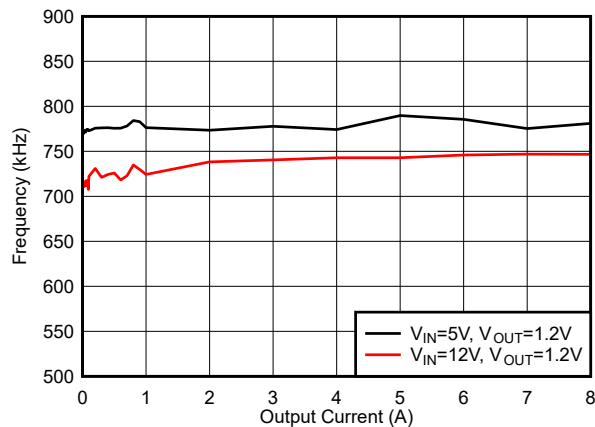
6-29. f_{SW} Load Regulation, Mode = FCCM, f_{SW} = 800\text{ kHz}
