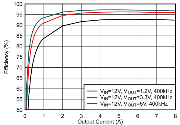
6-18. Efficiency, Mode = FCCM, f_{SW} = 400\text{ kHz}
