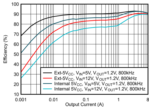
6-23. Efficiency, Ext-VCC vs Internal-VCC, Mode = DCM, f_{SW} = 800\text{ kHz}
