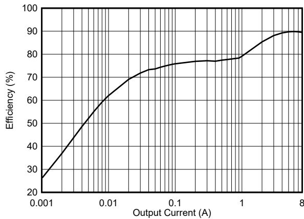
8-2. Efficiency
