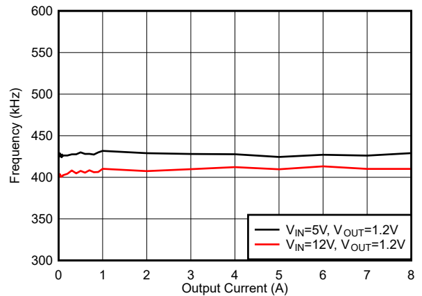
6-28. f_{SW} Load Regulation, Mode = FCCM, f_{SW} = 400\text{ kHz}
