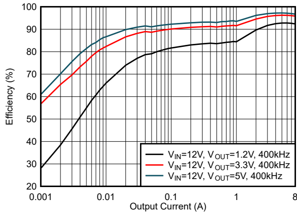
6-17. Efficiency, Mode = DCM, f_{SW} = 400\text{ kHz}
