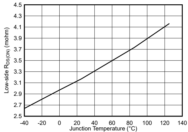
6-5. Low-Side R_{DS(on)} vs Temperature
