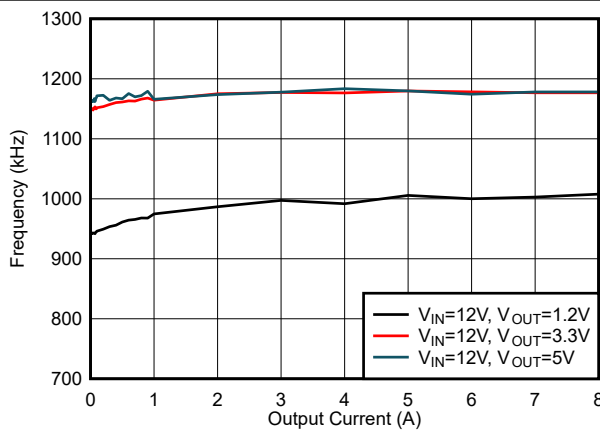
6-33. f_{SW} Load Regulation, Mode = FCCM, f_{SW} = 1200\text{ kHz}
