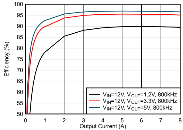
6-20. Efficiency, Mode = FCCM, f_{SW} = 800\text{ kHz}
