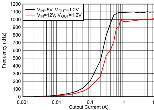
6-27. f_{SW} Load Regulation, Mode = DCM, f_{SW} = 1200\text{ kHz}
