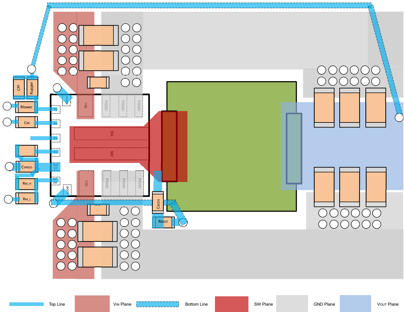
8-8. Layout Example
