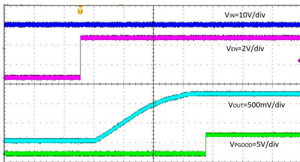
8-6. Start-Up Relative to EN Rising, Time = 2\ \text{ms/div}
