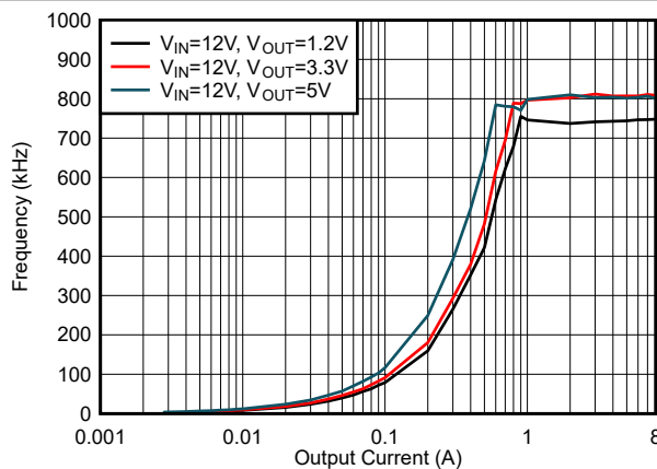
6-35. f_{SW} Load Regulation, Mode = DCM, f_{SW} = 800\text{ kHz}
