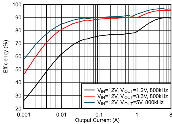
6-19. Efficiency, Mode = DCM, f_{SW} = 800\text{ kHz}
