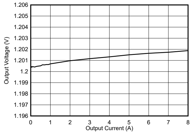
8-3. Load Regulation
