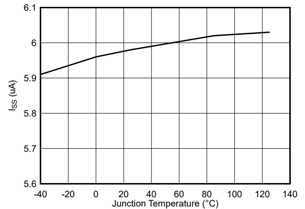
6-6. Soft-Start Charge Current vs Temperature
