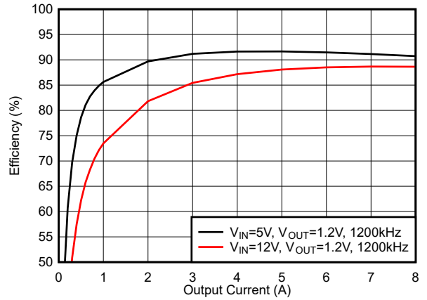
6-16. Efficiency, Mode = FCCM, f_{SW} = 1200\text{ kHz}
