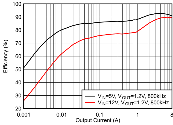
6-13. Efficiency, Mode = DCM, f_{SW} = 800\text{ kHz}
