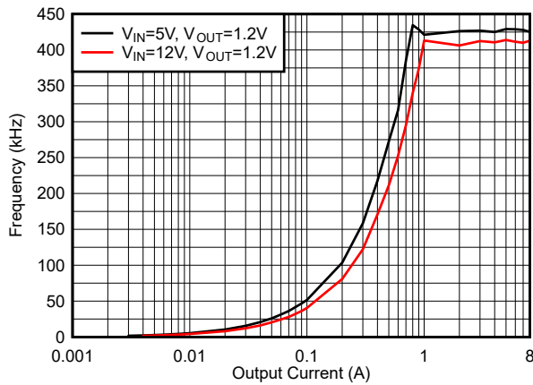
6-25. f_{SW} Load Regulation, Mode = DCM, f_{SW} = 400\text{ kHz}
