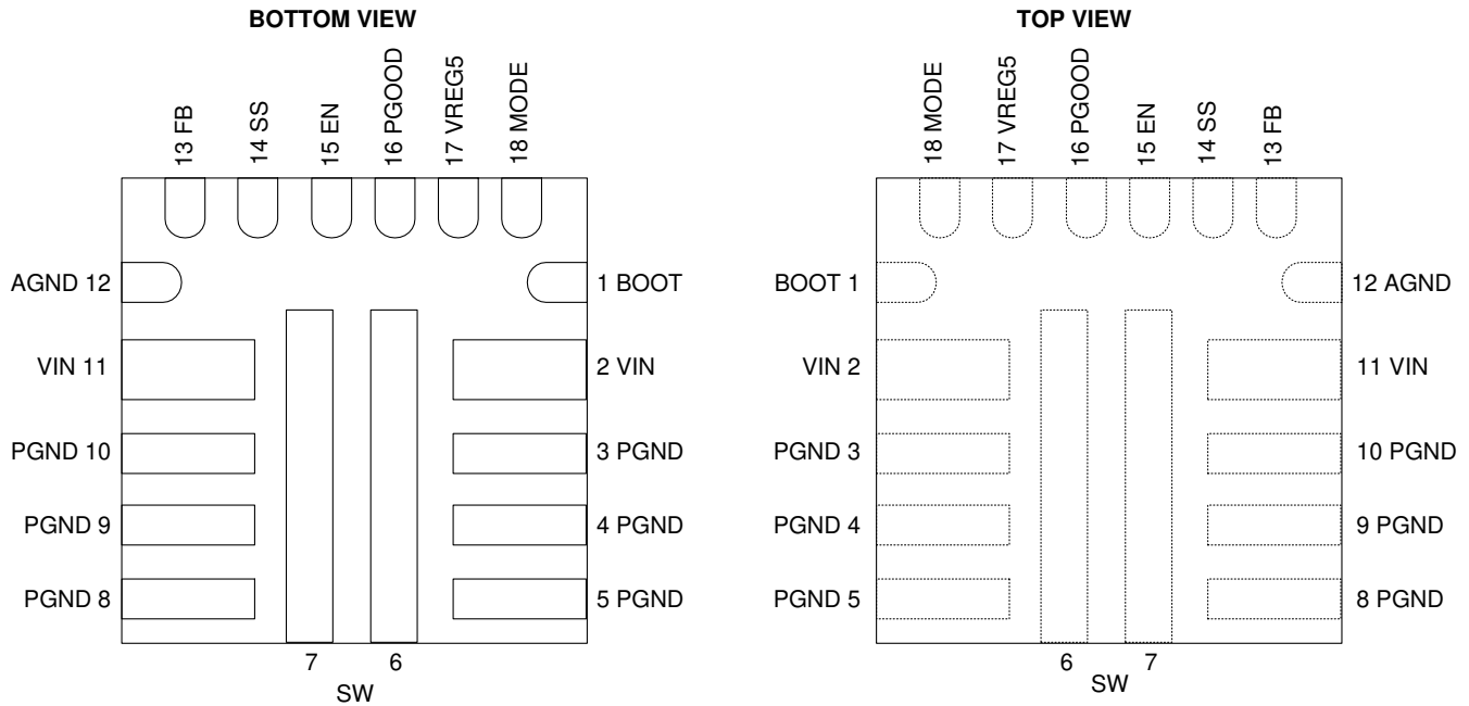
图 5-1. 18-Pin VQFN RNN Package (Bottom View Left, Top View Right)
