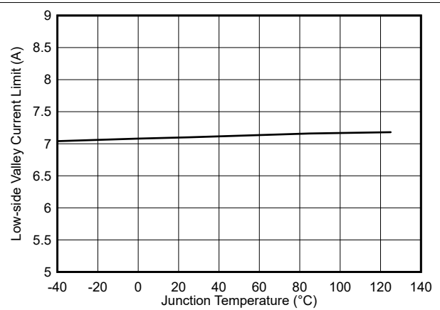
6-10. TPS568231 Current Limit (ILIM-1) vs Temperature
