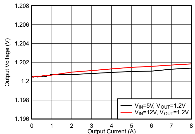
6-24. Load Regulation, f_{SW} = 800\text{ kHz}
