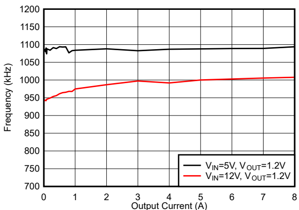
6-30. f_{SW} Load Regulation, Mode = FCCM, f_{SW} = 1200\text{ kHz}
