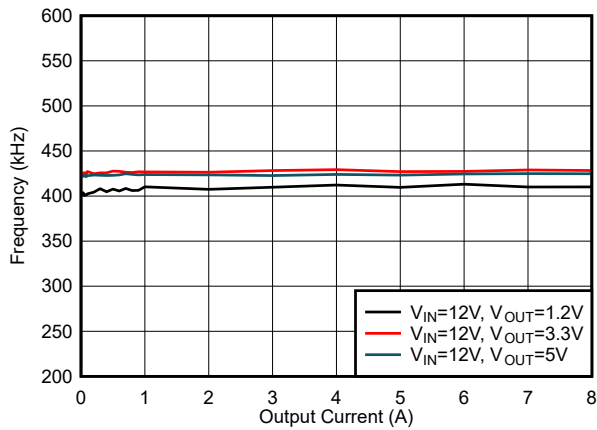
6-31. f_{SW} Load Regulation, Mode = FCCM, f_{SW} = 400\text{ kHz}
