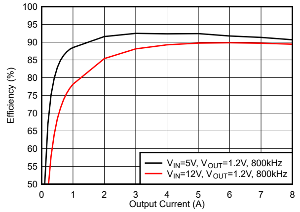
6-14. Efficiency, Mode = FCCM, f_{SW} = 800\text{ kHz}
