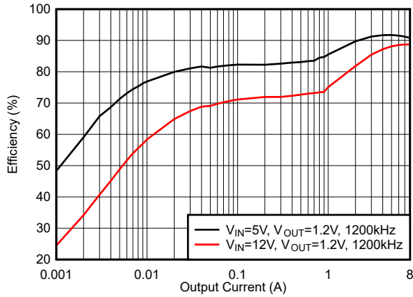
6-15. Efficiency, Mode = DCM, f_{SW} = 1200\text{ kHz}
