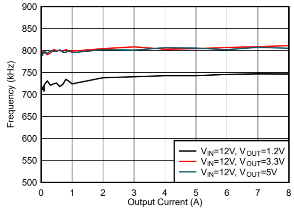
6-32. f_{SW} Load Regulation, Mode = FCCM, f_{SW} = 800\text{ kHz}
