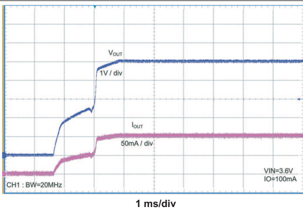
Figure 22. Power On V_{IN} = 3.6 \text{ V} , I_O = 100 \text{ mA}
