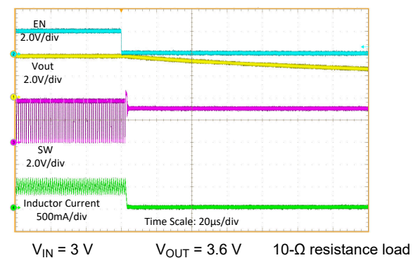
8-7. Shutdown Waveform
