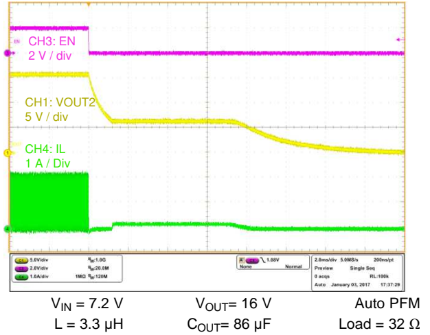
29. Shutdown by EN
