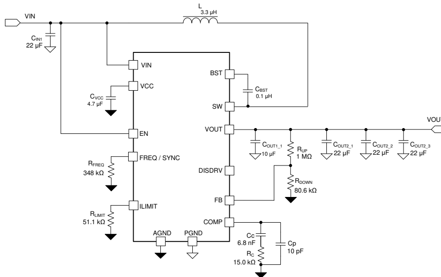
34. 16-V Output Voltage Without Load Disconnect Function
