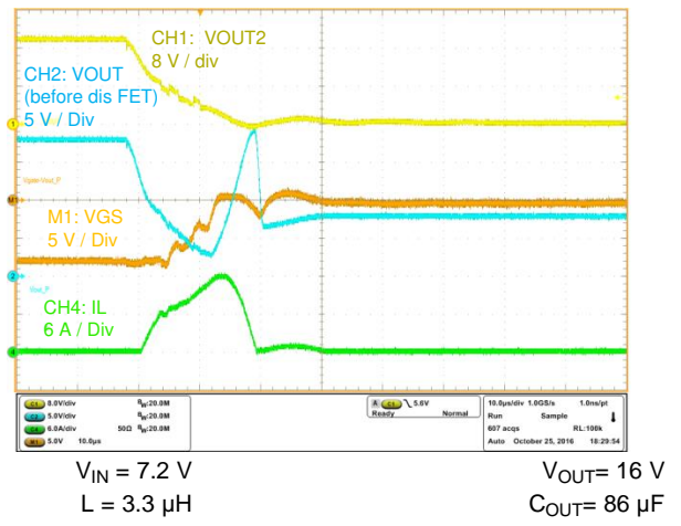
31. Output Short (with Disconnect FET)
