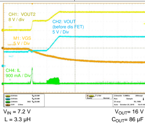
32. Output Short Release (with Disconnect FET)
