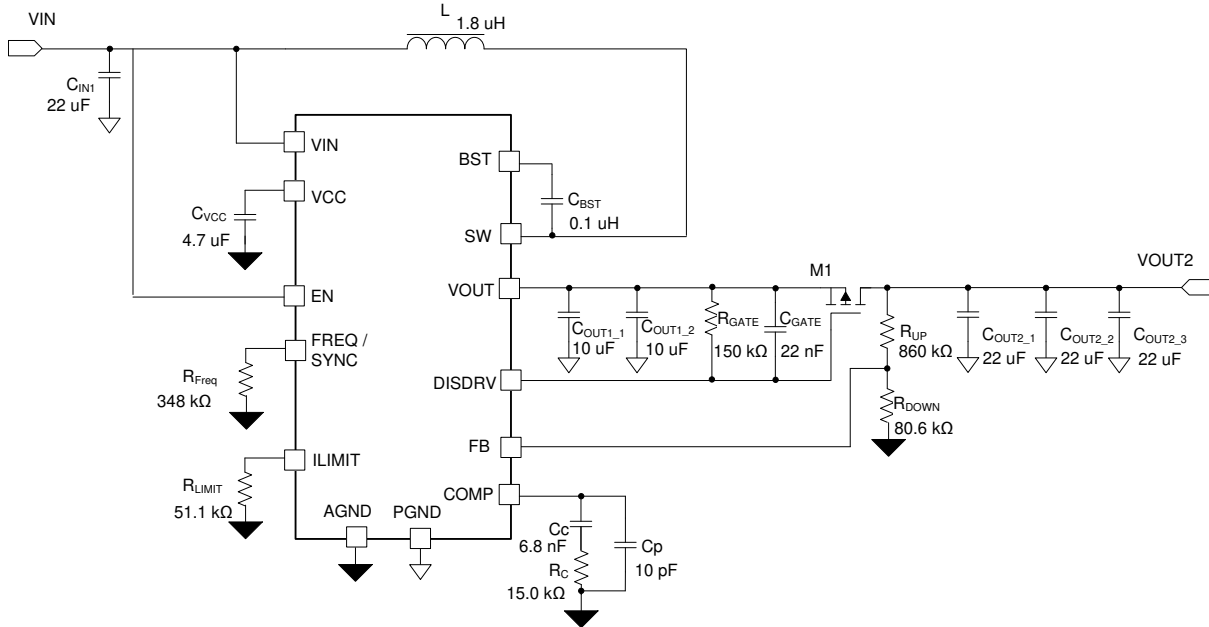
33. 14-V Output Voltage from 2.7-V to 4.4-V Input Voltage
