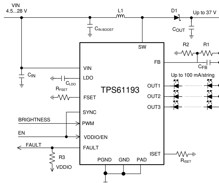
図 8-1. Three Strings 100-mA/String Configuration
