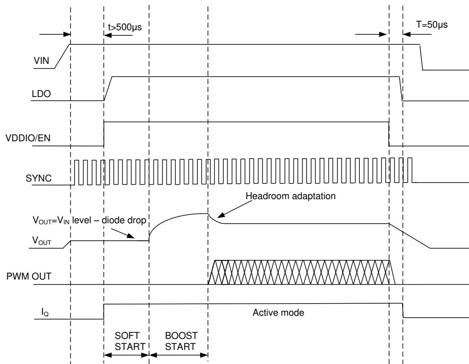
FIG 7-11. Timing Diagram for the Typical Start-Up and Shutdown
