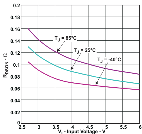
Figure 7-5. R_{DS(on)} High-Side Switch
