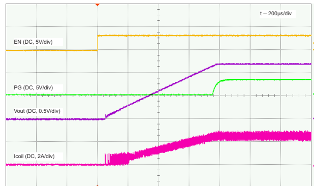
9-11. Start-Up, Load = 0.47 Ω
