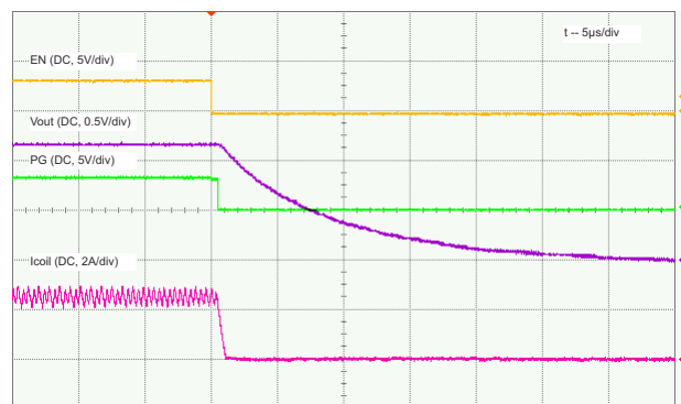
9-13. Shutdown, Load = 0.47 Ω
