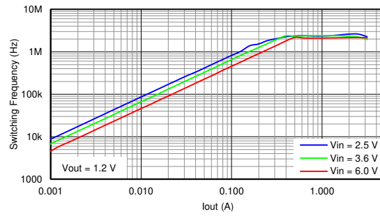
7-1. Switching Frequency
