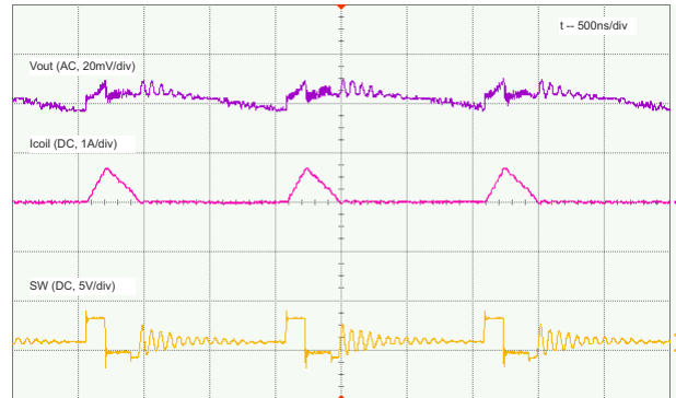
9-9. PSM Operation, Load = 100 mA
