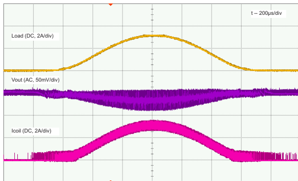
9-10. Load Sweep, Load = Open to 3 A
