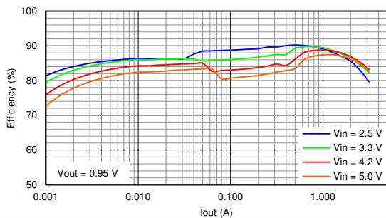
9-2. Efficiency
