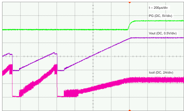
9-18. Output Short-Circuit Protection, Load = 0.47 Ω, Recovery
