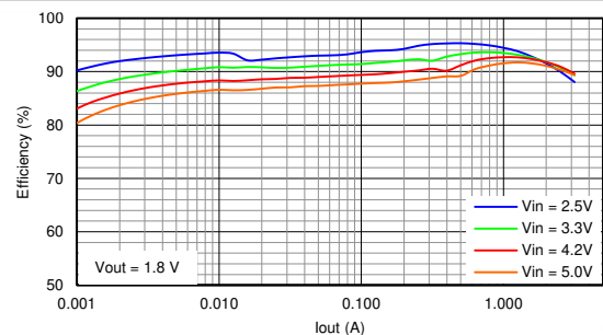
9-5. Efficiency
