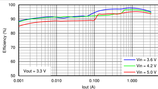
9-4. Efficiency
