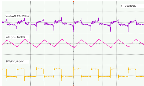
9-8. PWM Operation, Load = 3 A
