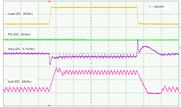
9-15. Load Transient, Load = 0.5 A to 3 A
