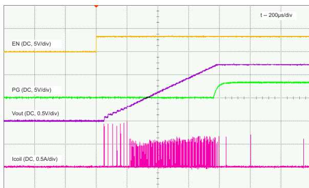
9-12. Start-Up, Load = Open
