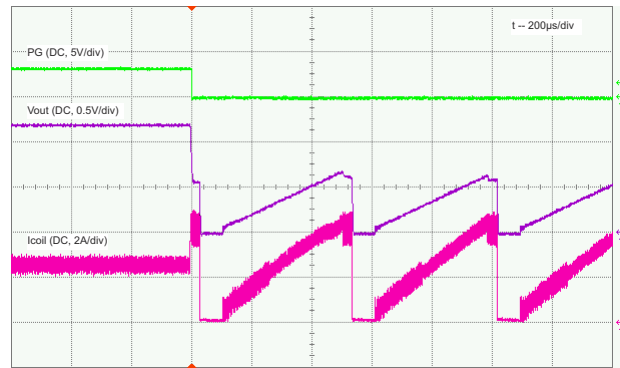
9-17. Output Short-Circuit Protection, Load = 0.47 Ω, Entry
