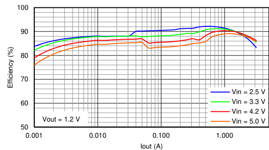
9-3. Efficiency
