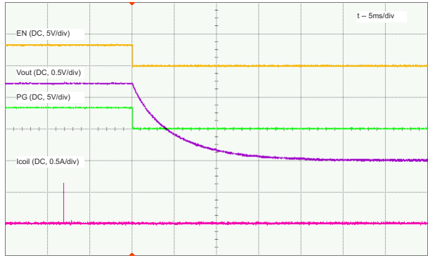
9-14. Shutdown, Load = Open
