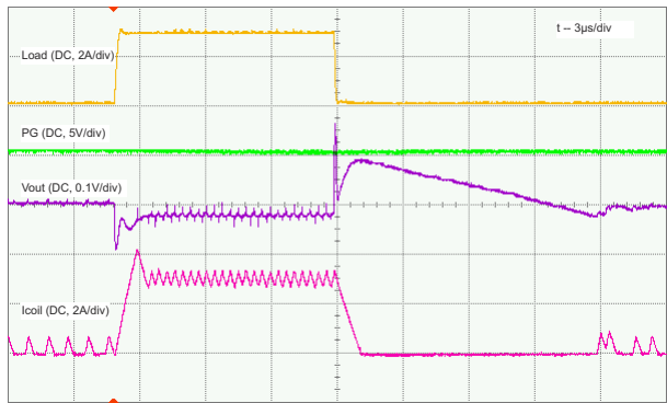
9-16. Load Transient, Load = 50 mA to 3 A
