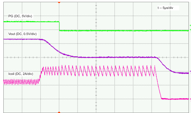
9-19. Output Short-Circuit Protection, Load = 0.47 Ω, HICCUP Zoom In
