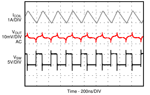
8-27. PWM Operation
