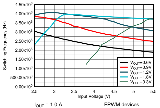
8-26. Switching Frequency
