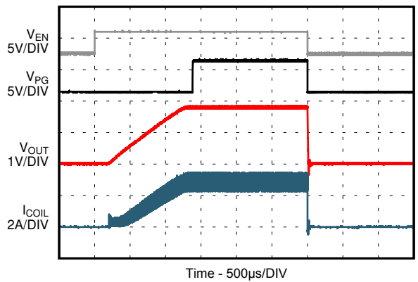
8-30. Start-Up With No Load
