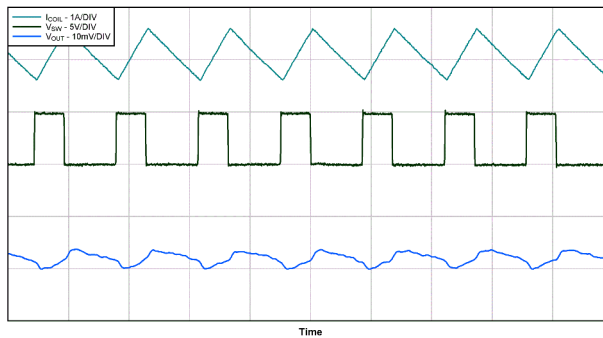
8-27. PWM Operation
