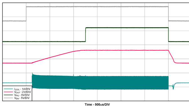
8-31. Start-Up With No Load
