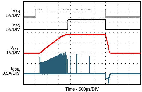
8-28. PSM Operation
