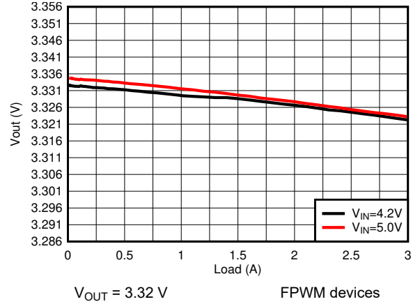
8-22. Load Regulation
