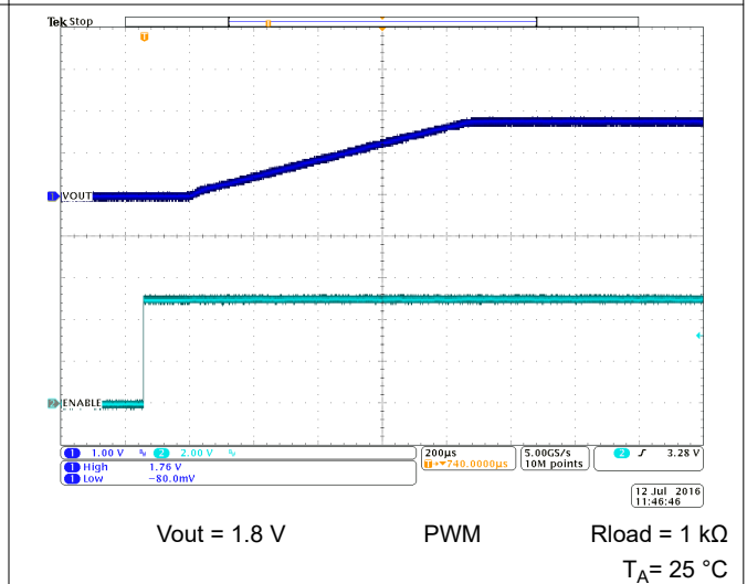
图 10-44. Start-Up Timing
