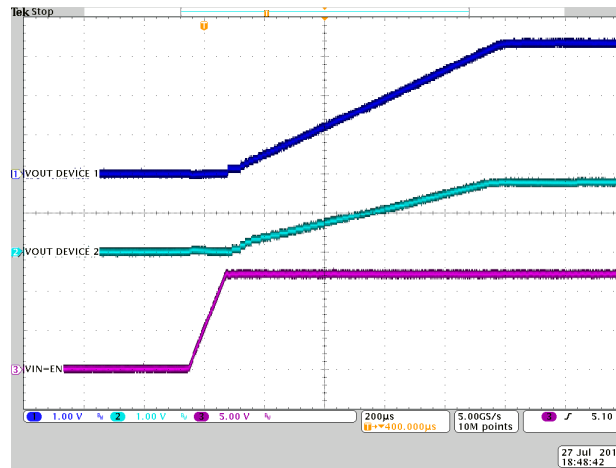
Figure 10-86. Tracking
