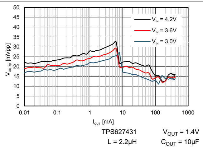
9-14. Typical Output Ripple Voltage V_{OUT} = 1.4\text{ V}
