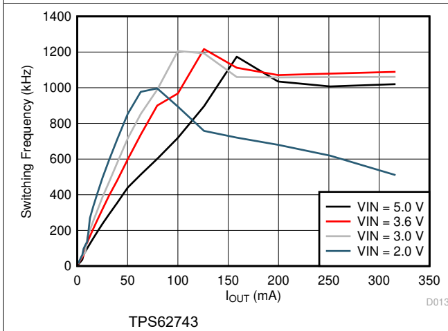
9-13. Switching Frequency vs Load Current V_{OUT} = 1.2\text{ V}
