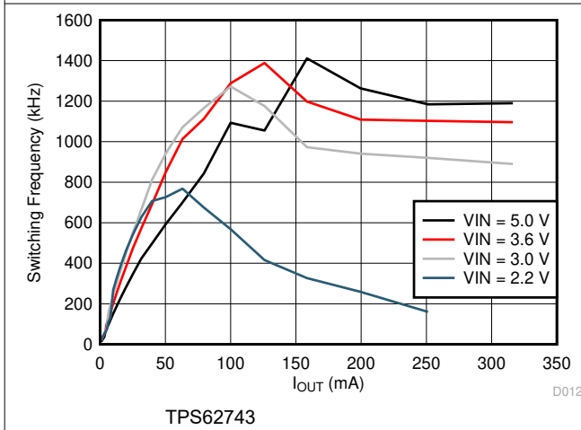
9-11. Switching Frequency vs Load Current V_{OUT} = 1.8\text{ V}
