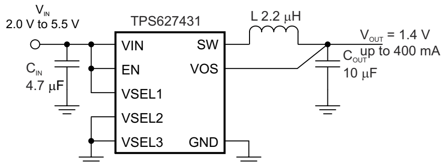
図 9-2. TPS627431 Typical Application Circuit
