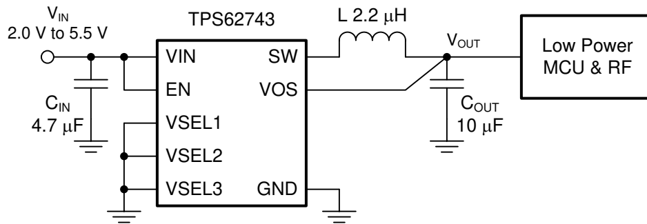
図 9-1. TPS62743 Typical Application Circuit
