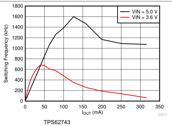
9-10. Switching Frequency vs Load Current V_{OUT} = 3.3\text{ V}
