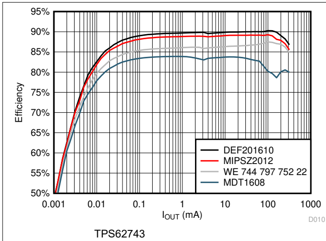
9-9. Efficiency vs Load Current; V_{OUT} = 1.8\text{ V}
