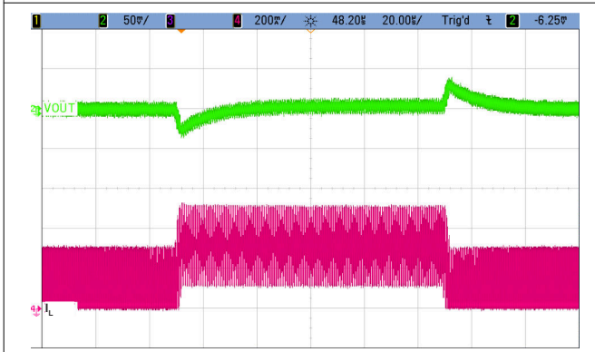
图 9-19. Load Transient Response; 100 mA to 290 mA
