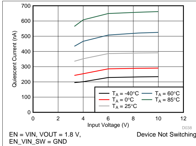
Figure 1. Quiescent Current
