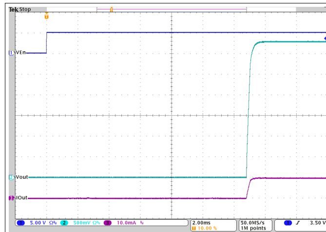
Figure 35. TPS62745 with V_{OUT} = 3.3 V Startup
