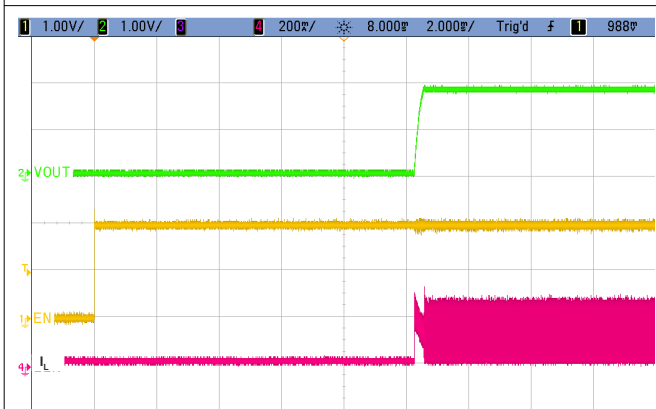
图 9-16. Startup Into 100 mA Electronic Load EN Delay + Soft-Start Delay
