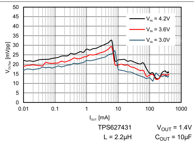
9-13. Typical Output Ripple Voltage V_{OUT} = 1.4\text{ V}
