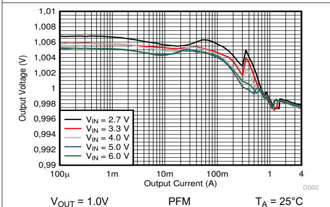
9-18. Output Voltage versus Output Current
