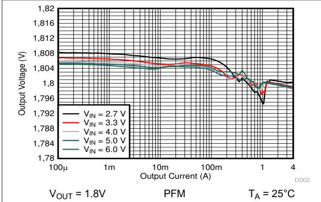
9-14. Output Voltage versus Output Current
