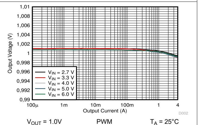
9-19. Output Voltage versus Output Current
