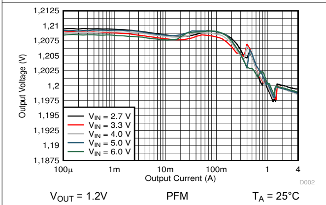
9-16. Output Voltage versus Output Current
