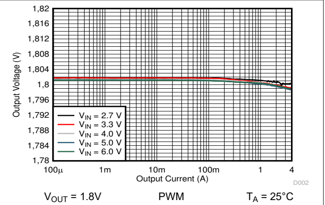
9-15. Output Voltage versus Output Current
