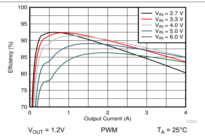
9-7. Efficiency versus Output Current
