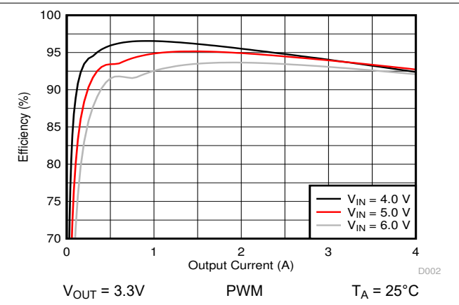
9-3. Efficiency versus Output Current
