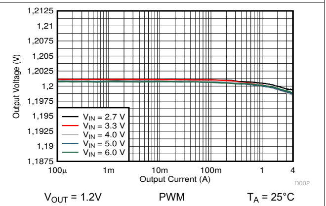
9-17. Output Voltage versus Output Current
