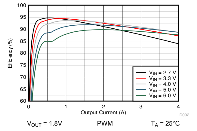
9-5. Efficiency versus Output Current
