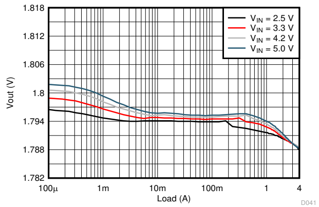
8-10. Load Regulation
