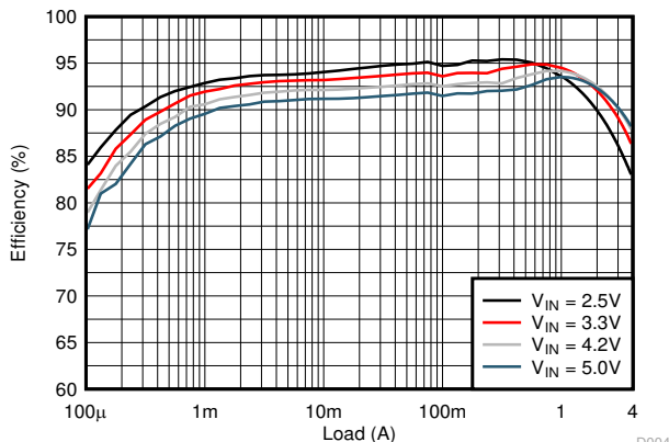
8-9. PWM Efficiency
