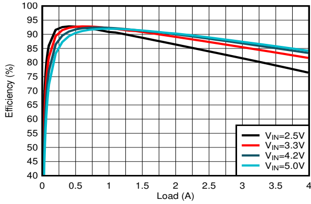
8-9. PWM Efficiency
