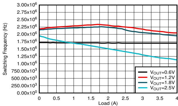
8-23. Switching Frequency
