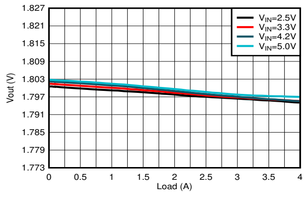
8-14. Load Regulation
