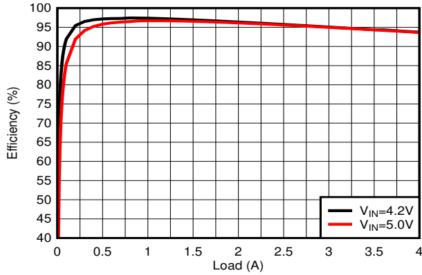
8-21. PWM Efficiency
