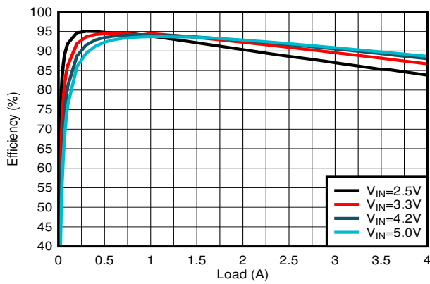
8-11. Efficiency
