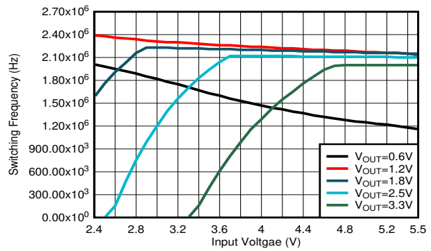
8-24. Switching Frequency
