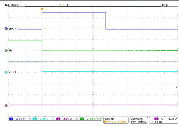
PFM or PWM TPS628303BDRL T_A = 25\text{ }^\circ\text{C}
