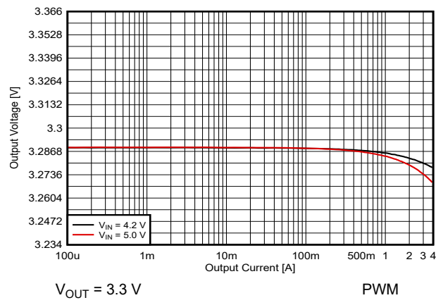
8-26. Output Voltage versus Output Current
