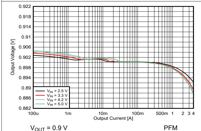
8-17. Output Voltage versus Output Current
