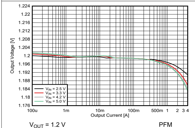
8-19. Output Voltage versus Output Current
