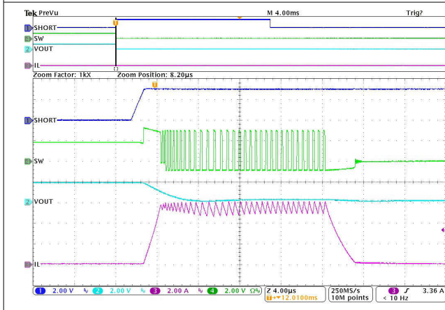
PFM or PWM TPS628303BDRL T_A = 25\text{ }^\circ\text{C}
