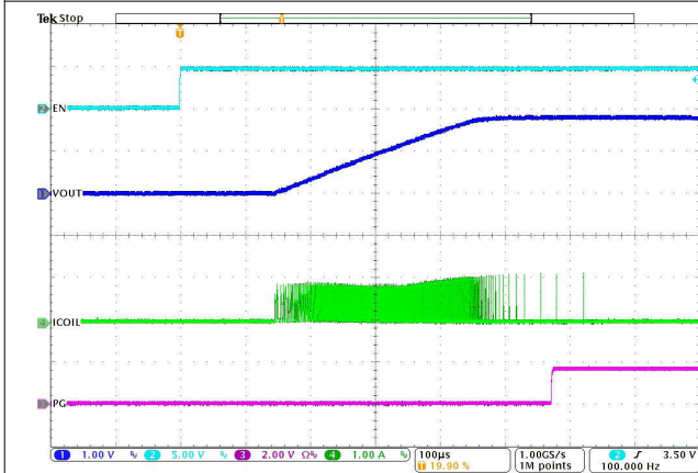
I_{OUT} = 0\text{ mA} PFM or PWM T_A = 25\text{ }^\circ\text{C} 'A' and 'B' versions
