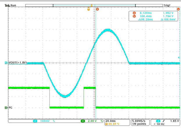
PFM or PWM TPS628303BDRLR T_A = 25\text{ }^\circ\text{C}
