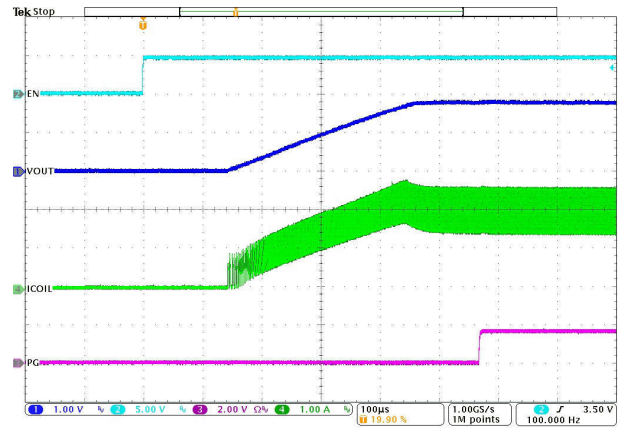
I_{OUT} = 2.0\text{ A} PFM or PWM T_A = 25\text{ }^\circ\text{C} 'A' and 'B' versions
