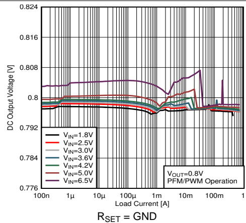
25. Output Voltage versus Load Current V_{OUT} = 0.8\text{ V}
