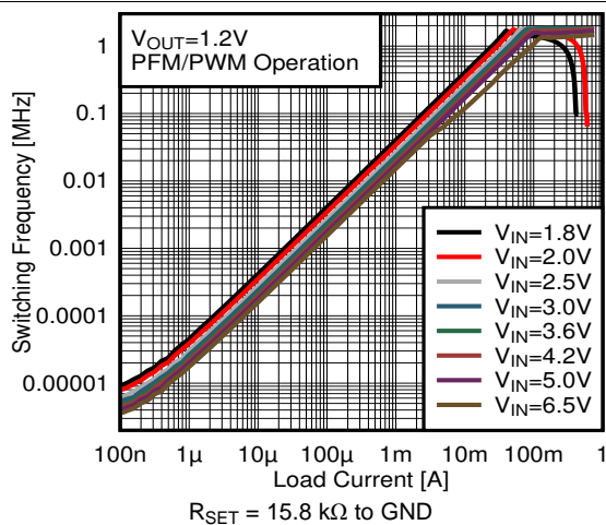
36. Switching Frequency versus Load Current V_{OUT} = 1.2 V
