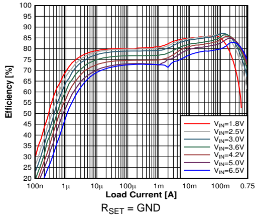
20. Efficiency Power Save Mode V_{OUT} = 0.8\text{ V} for the DGR device
