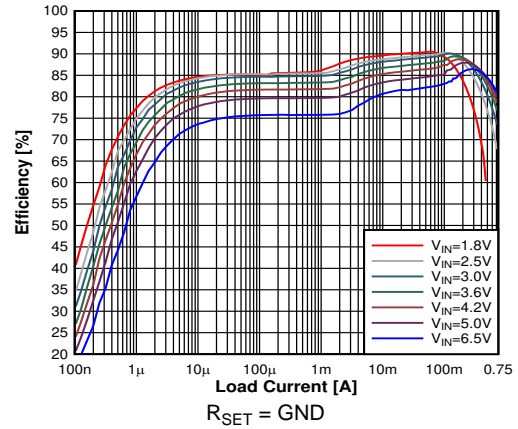
21. Efficiency Power Save Mode V_{OUT} = 1.2\text{ V} for the DGR device
