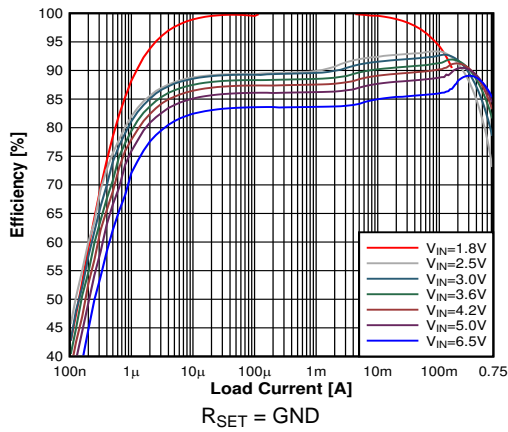
22. Efficiency Power Save Mode V_{OUT} = 1.8\text{ V} for the DGR device
