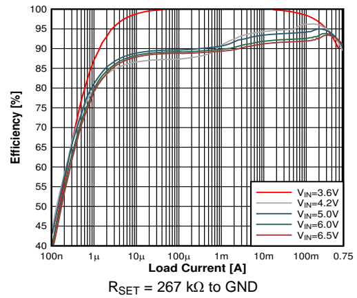
23. Efficiency Power Save Mode V_{OUT} = 3.6\text{ V} for the DGR device
