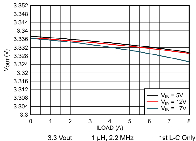
図 7-9. Output Voltage vs Load Current
