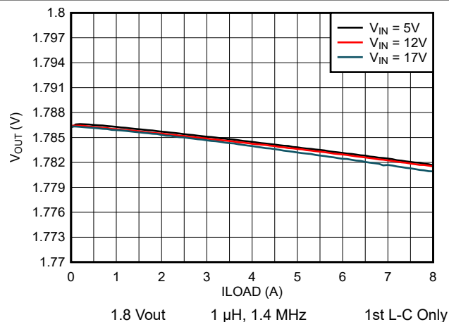
図 7-8. Output Voltage vs Load Current
