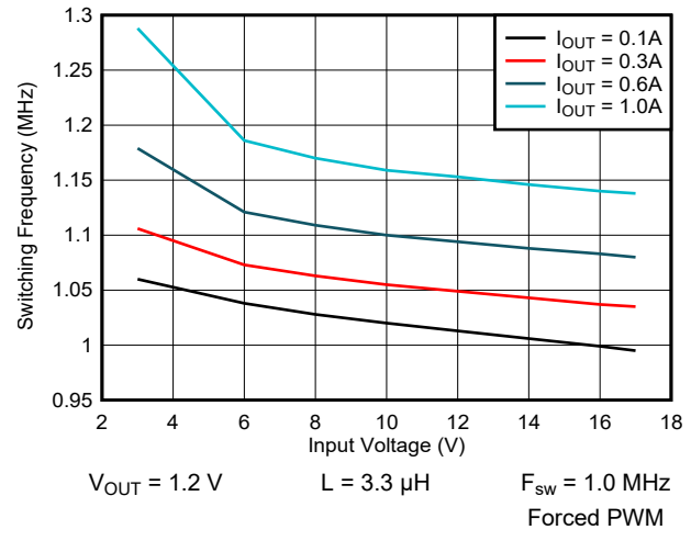
9-47. Switching Frequency vs Input Voltage
