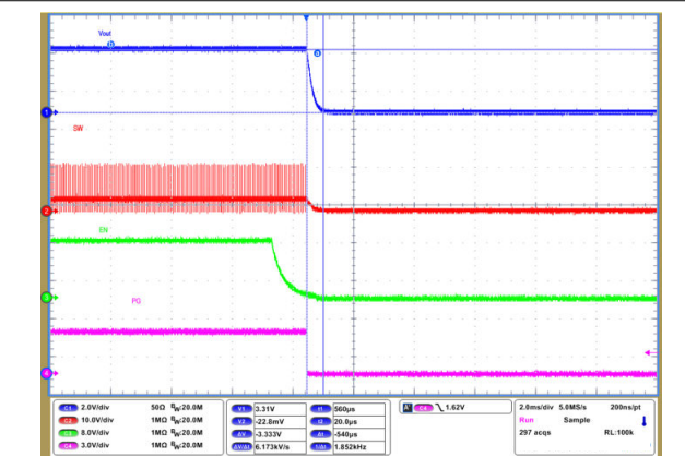
9-65. Shutdown Timing with Output Discharge Enabled
