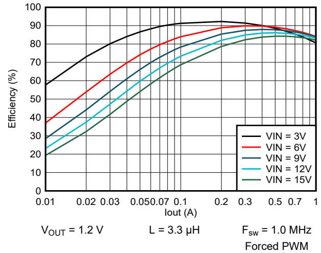
9-45. Efficiency vs Output Current
