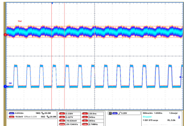
FIG 9-75. Output Voltage Ripple
