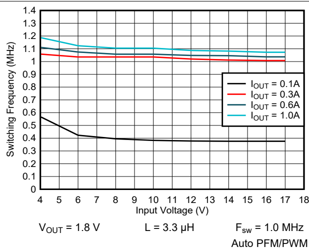
Figure 9-34. Switching Frequency vs Input Voltage
