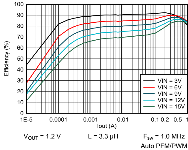
9-44. Efficiency vs Output Current
