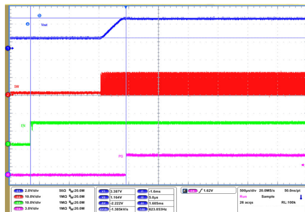
9-62. Start-Up Timing
