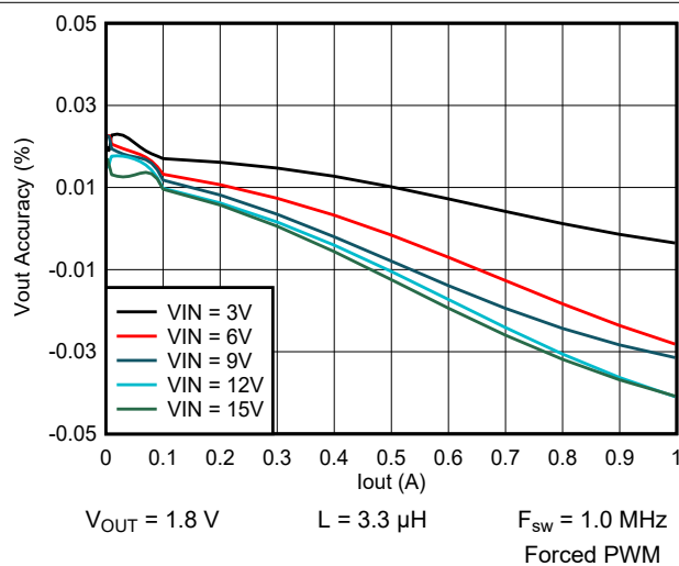
9-37. Output Voltage vs Output Current
