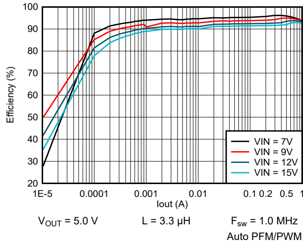
Figure 9-8. Efficiency vs Output Current
