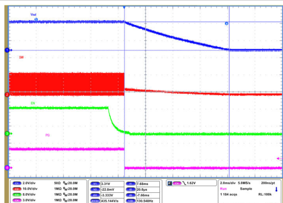
Figure 9-68. Shutdown Timing with Output Discharge Disabled
