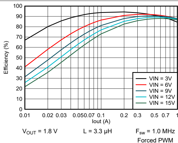
FIG 9-33. Efficiency vs Output Current
