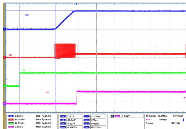
9-62. Start-Up Timing
