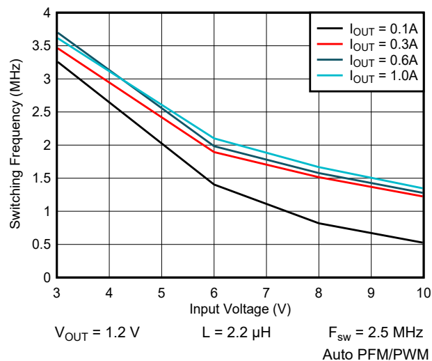
9-40. Switching Frequency vs Input Voltage
