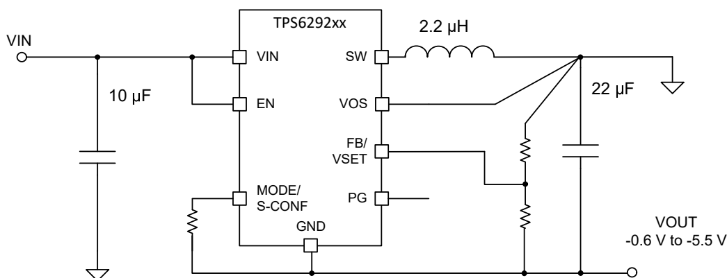
FIG 9-77. IBB Example with Adjustable Feedback
