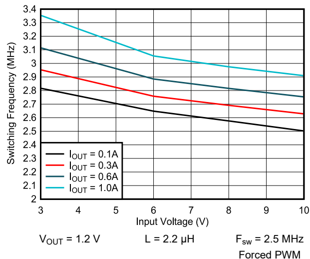
9-41. Switching Frequency vs Input Voltage
