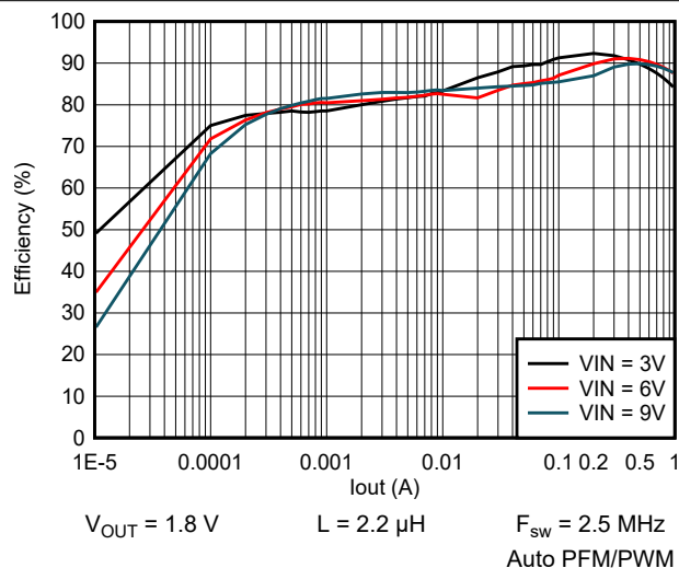
Figure 9-26. Efficiency vs Output Current
