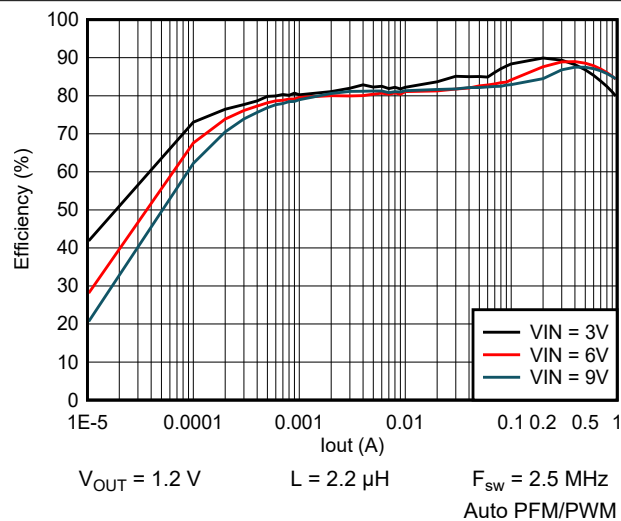
9-38. Efficiency vs Output Current
