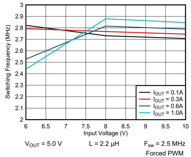
Figure 9-5. Switching Frequency vs Input Voltage
