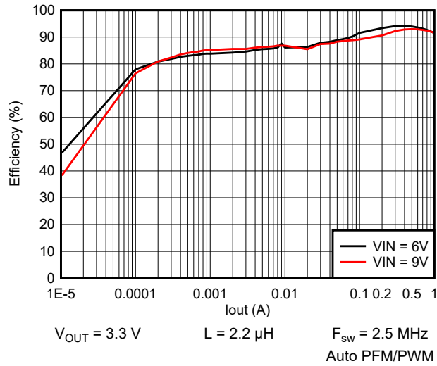
Figure 9-14. Efficiency vs Output Current
