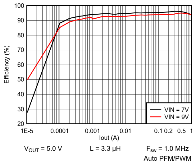
9-8. Efficiency vs Output Current
