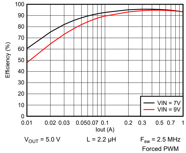
Figure 9-3. Efficiency vs Output Current
