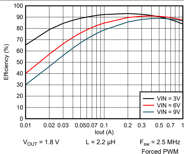
Figure 9-27. Efficiency vs Output Current
