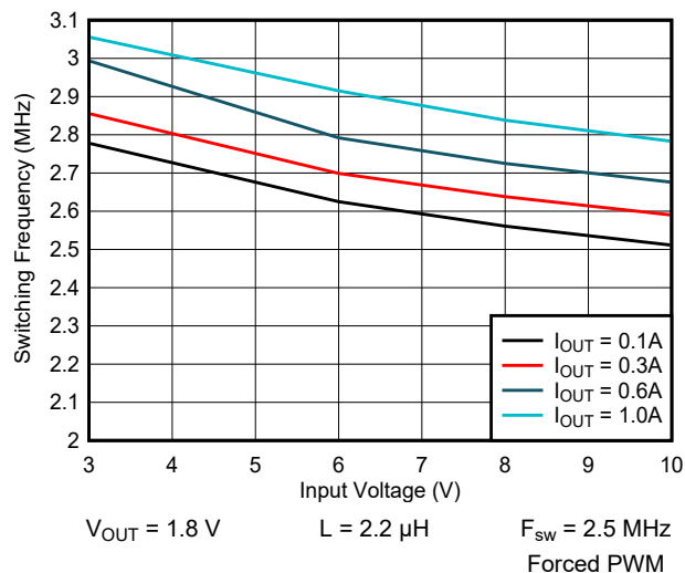
Figure 9-29. Switching Frequency vs Input Voltage
