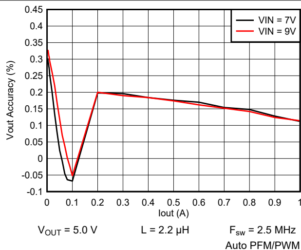
9-6. Output Voltage vs Output Current
