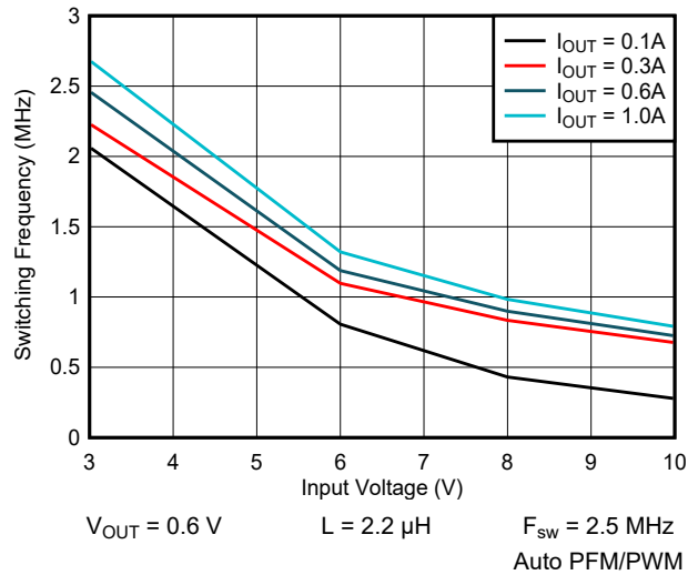
9-52. Switching Frequency vs Input Voltage
