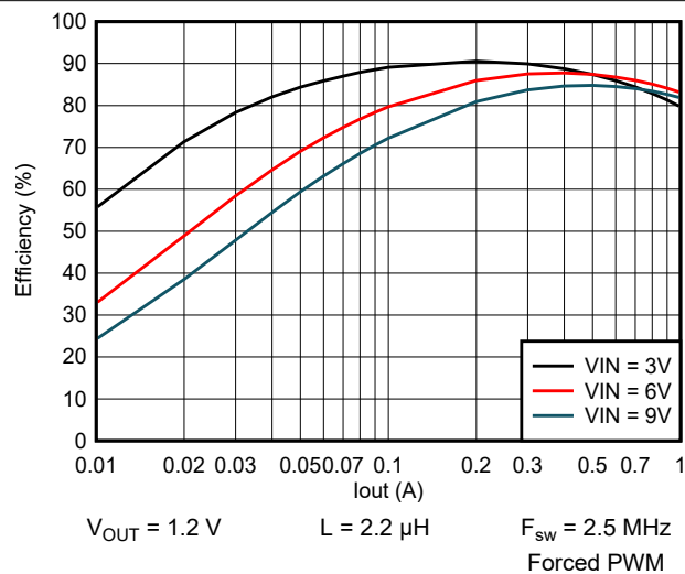
9-39. Efficiency vs Output Current
