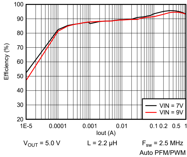
Figure 9-2. Efficiency vs Output Current
