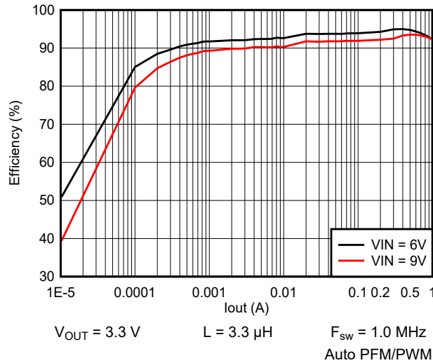
9-20. Efficiency vs Output Current
