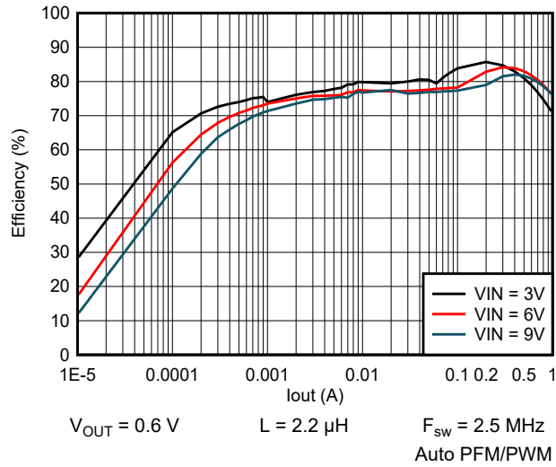
9-50. Efficiency vs Output Current
