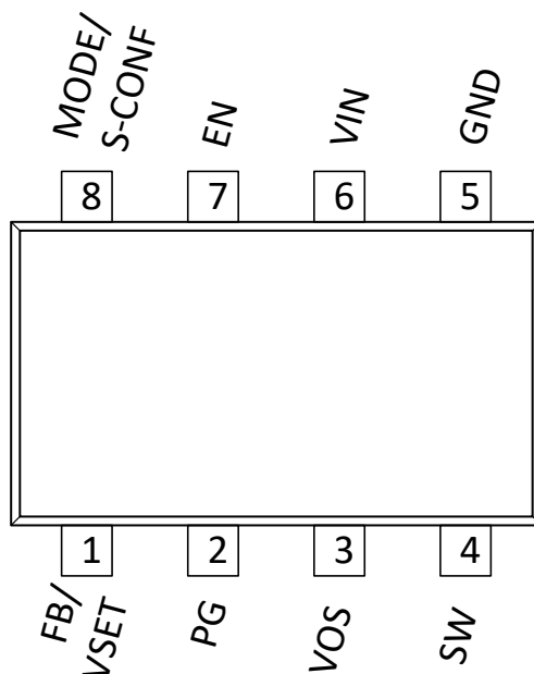
6-1. TPS629211-Q1 8-Pin DRL SOT-5X3 Pinout (TOP)
