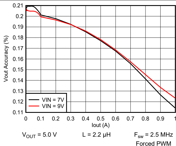
9-7. Output Voltage vs Output Current
