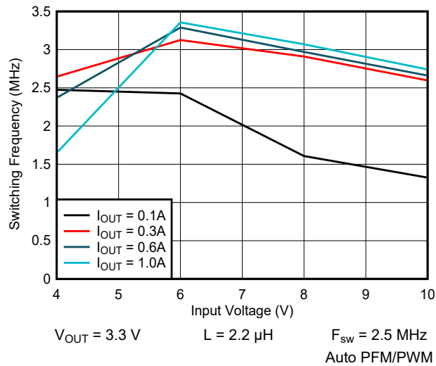
Figure 9-16. Switching Frequency vs Input Voltage
