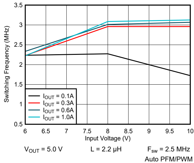
Figure 9-4. Switching Frequency vs Input Voltage
