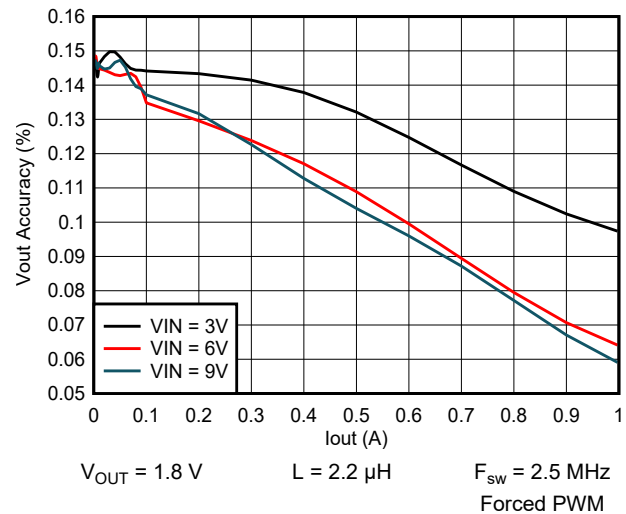
9-31. Output Voltage vs Output Current
