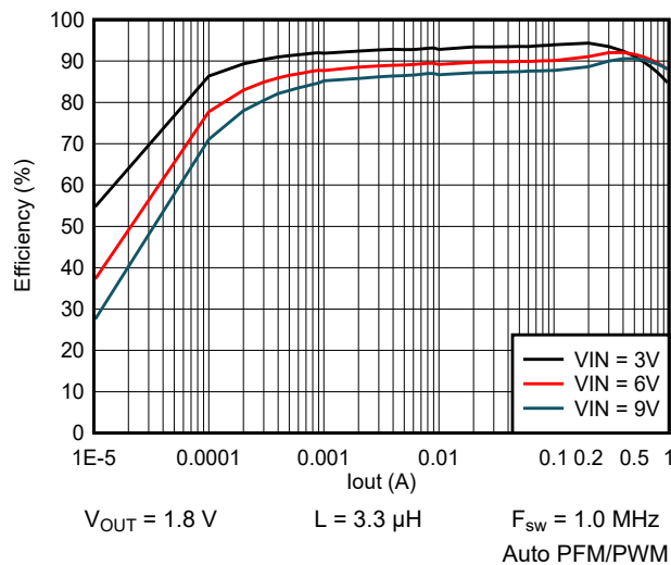
9-32. Efficiency vs Output Current
