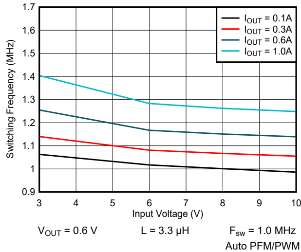
Figure 9-58. Switching Frequency vs Input Voltage
