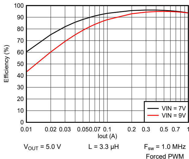
9-9. Efficiency vs Output Current
