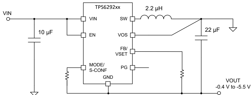
FIG 9-78. IBB Example with Internal Feedback
