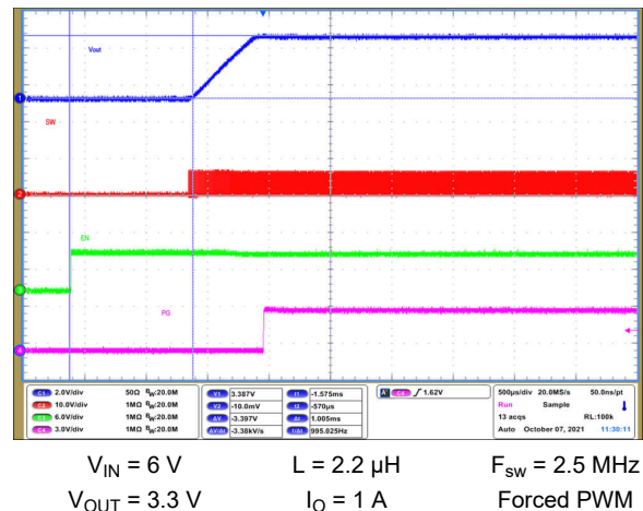
Figure 9-63. Start-Up Timing
