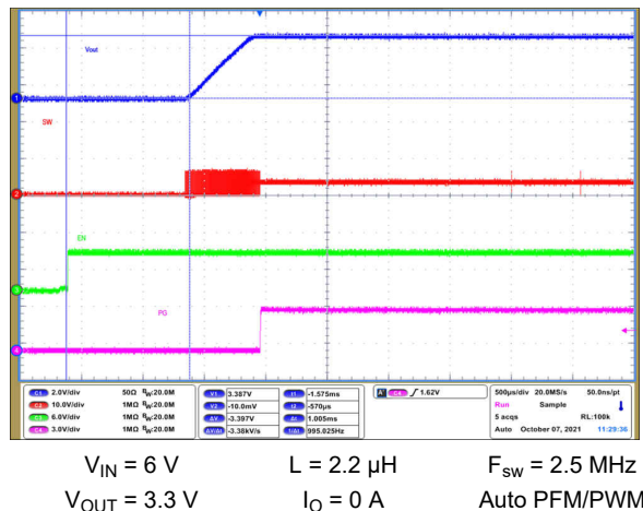
Figure 9-62. Start-Up Timing
