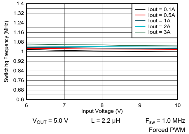
9-49. Switching Frequency vs Input Voltage
