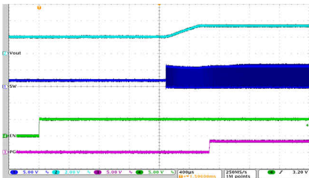
9-66. Start-Up Timing
