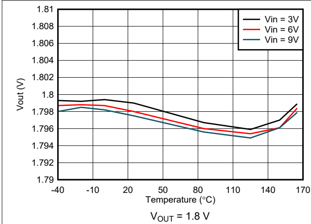
7-7. Output Voltage Accuracy - VSET Selected
