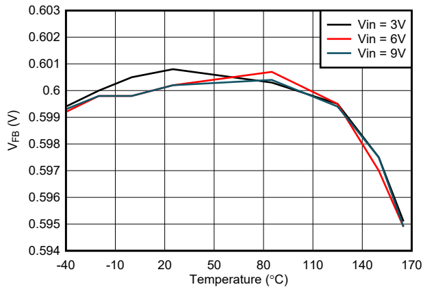
7-3. Feedback Voltage Accuracy - External Feedback Selected
