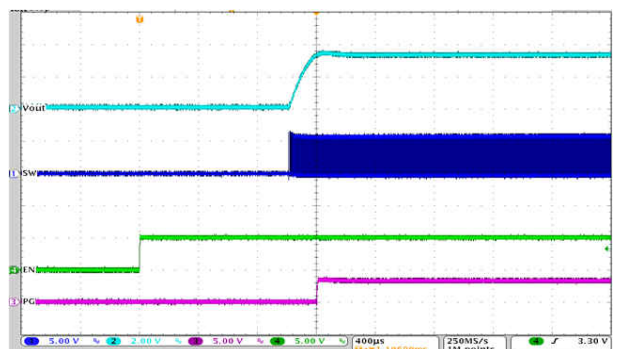
9-65. Start-Up Timing
