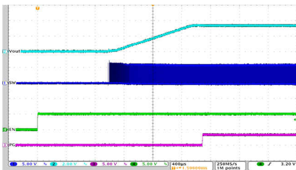
9-64. Start-Up Timing
