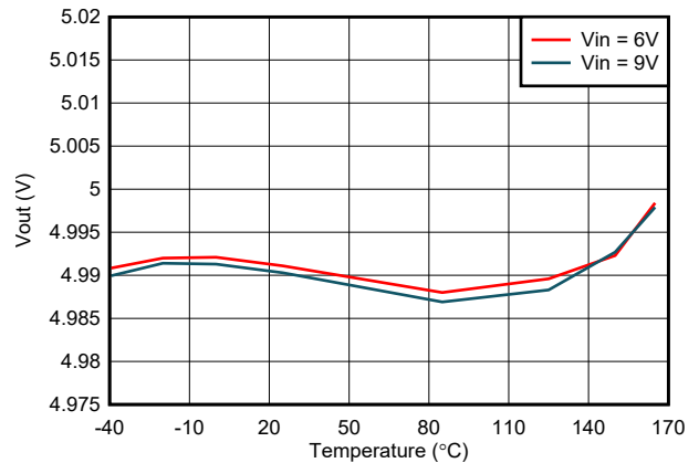
7-4. Output Voltage Accuracy - VSET Selected
