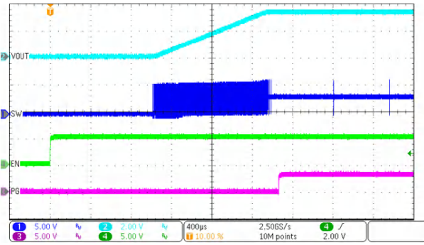
9-64. Start-Up Timing
