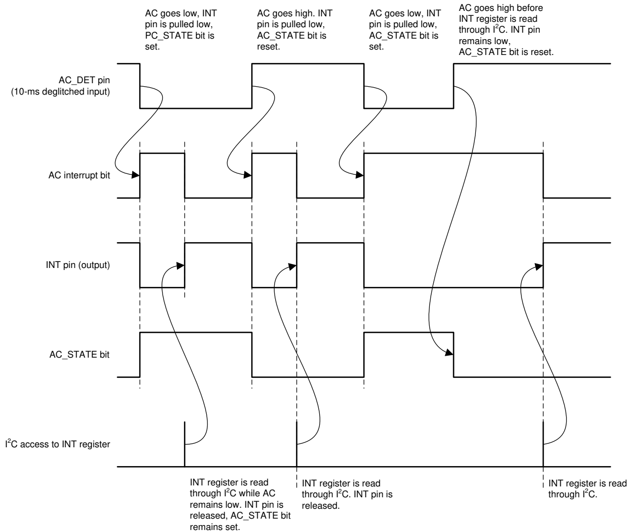
8-29. AC_STATE Pin
