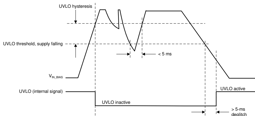
FIG 8-15. Definition of UVLO and Hysteresis
