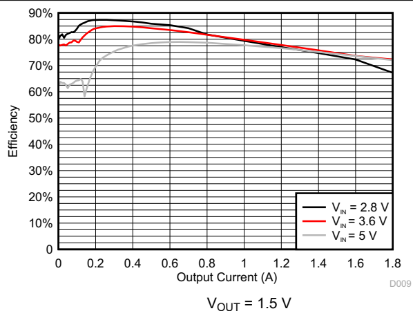
9-6. DCDC3 Efficiency
