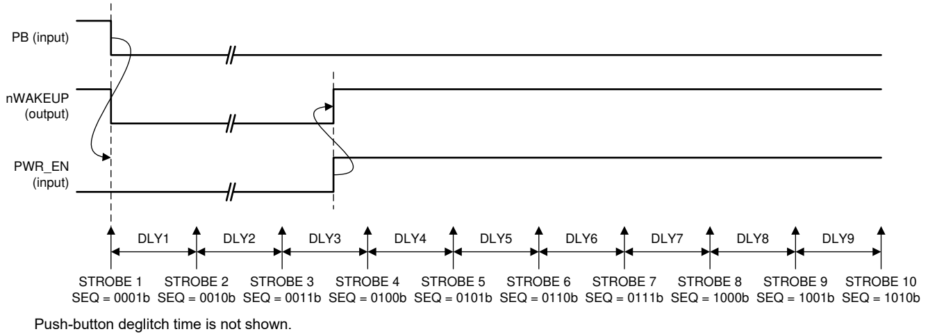
8-1. Power-Up Sequences from OFF or SUSPEND State; PB is Power-Up Event
