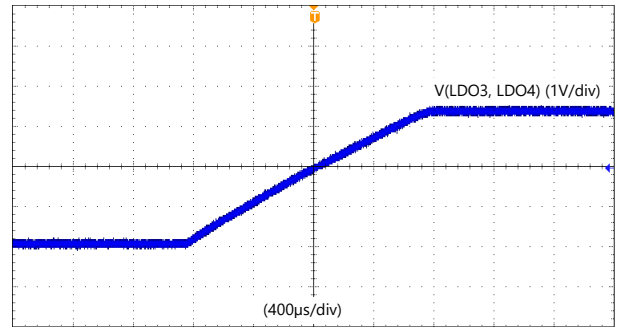
V_{IN} = 5.0V V_{OUT} = 3.3V T_A = 25^\circ C LDO モード/低速ラ ンプ I_{out} = 300mA C_{OUT\_total} = 10\mu F
