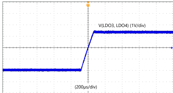
V_{IN} = 5.0V V_{OUT} = 3.3V T_A = 25^\circ C LDO モード/高速ラ ンプ I_{out} = 300mA C_{OUT\_total} = 10\mu F
