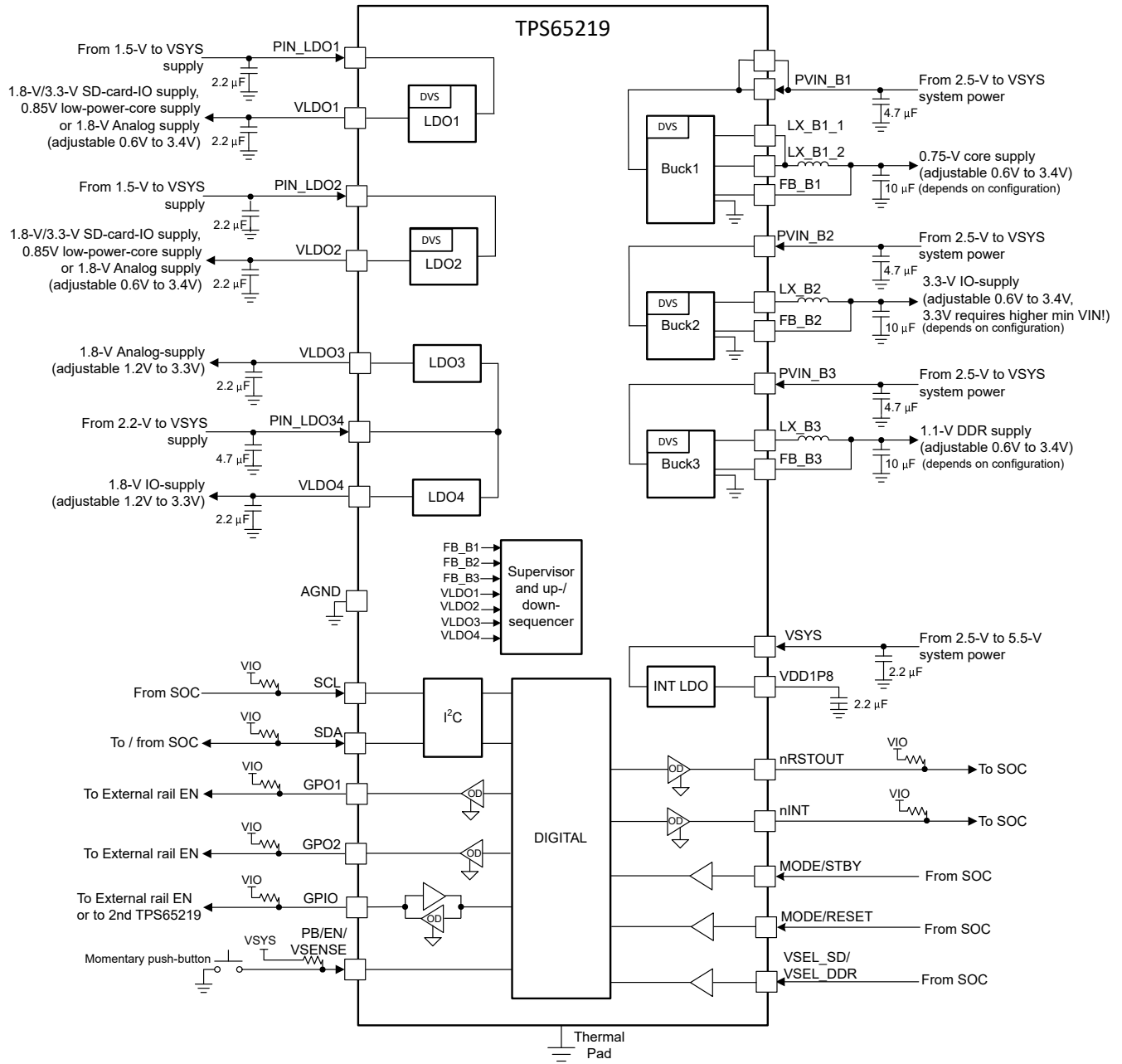
図 7-1. Functional Block Diagram
