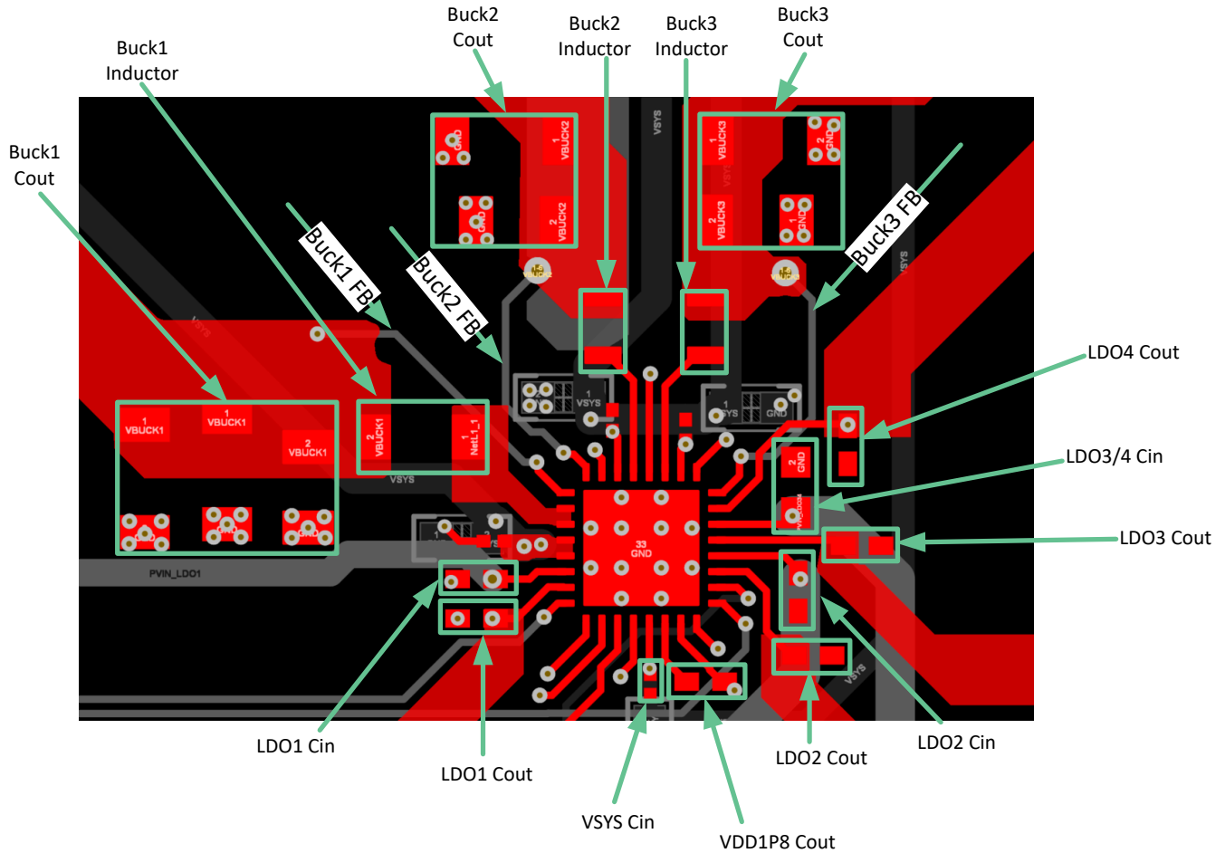
8-12. Example PMIC Layout
