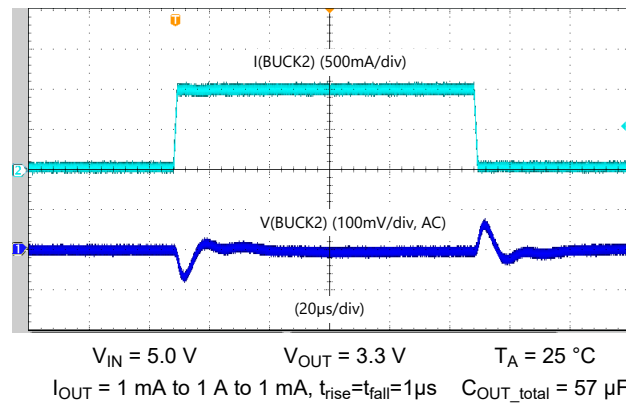
図 6-4. BUCK2 Load-step response - Low Bandwidth, forced PWM
