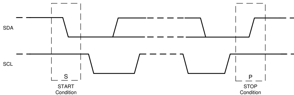
図 7-5. Start and Stop Sequences
