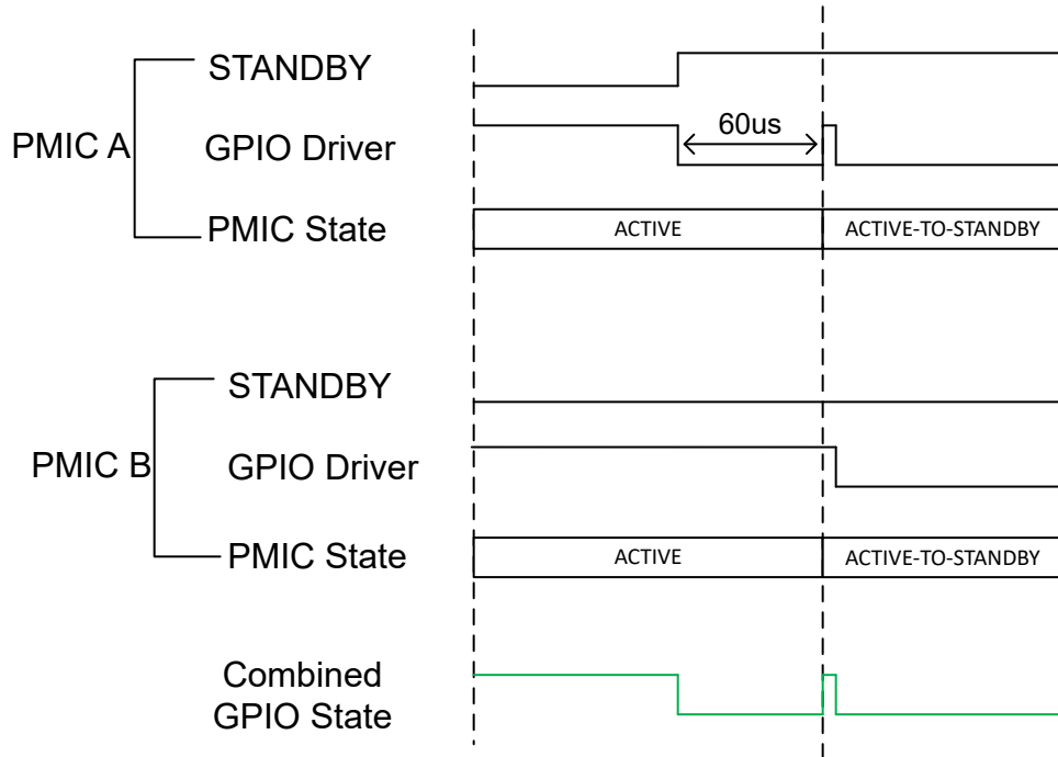
图 7-14. Synchronization before transitioning to Standby/OFF request/COLD RESET
