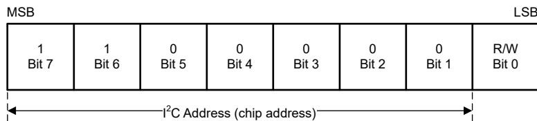
图 7-7. Example Device Address
