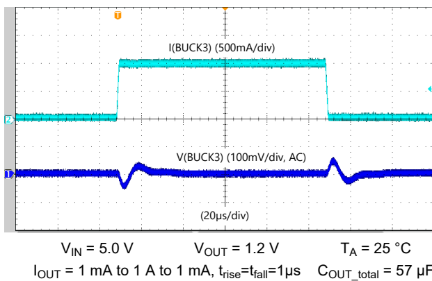
図 6-5. BUCK3 Load-step response - Low Bandwidth, forced PWM
