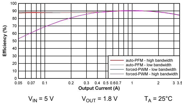
図 6-1. Efficiency BUCK1
