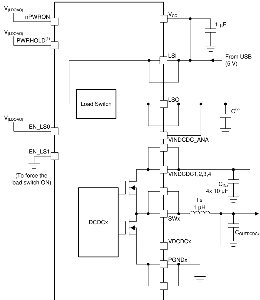
8-13. Load Switch Connected as USB Input Current Limited Switch
