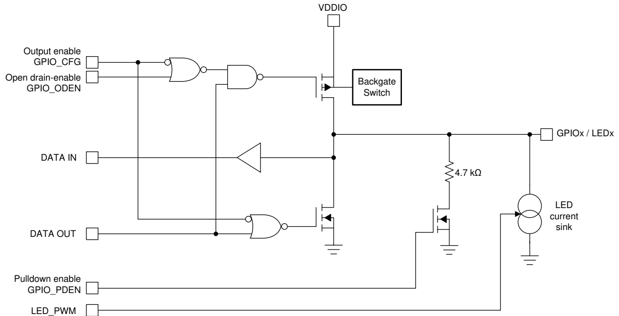
FIG 8-2. GPIO Block for GPIO3, GPIO4, and GPIO5
