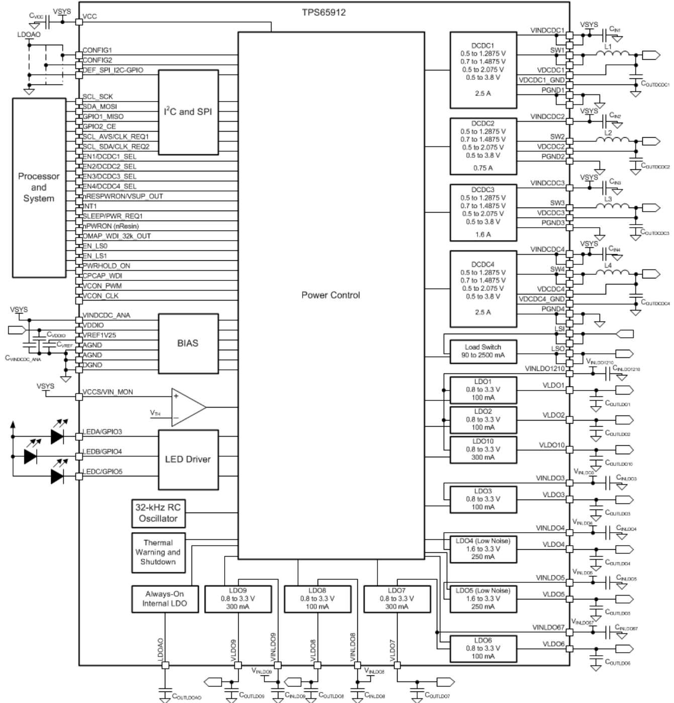
9-1. Typical Application Schematic
