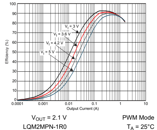
6-16. DCDC3 Efficiency vs Output Current
