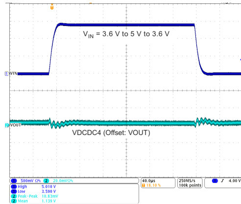
9-9. DCDC4 Line Transient Response
