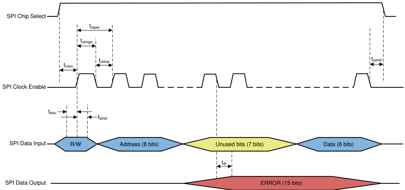
7-3. SPI Timing
