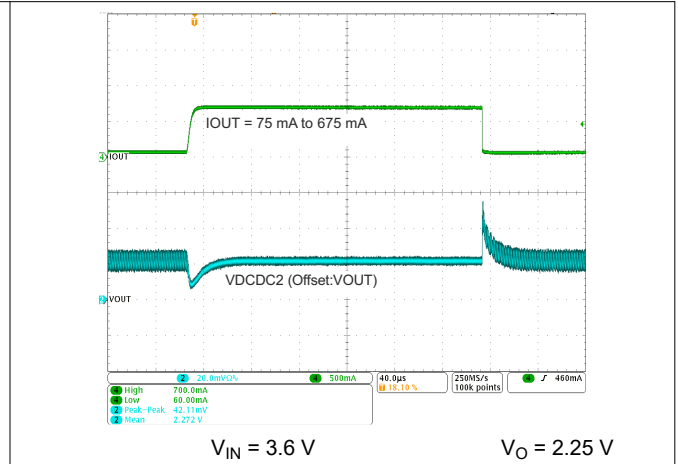
9-3. DCDC2 Load Transient Response
