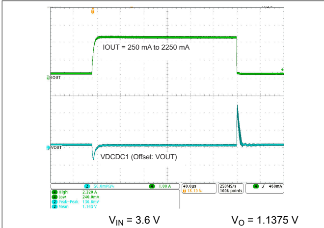
9-2. DCDC1 Load Transient Response
