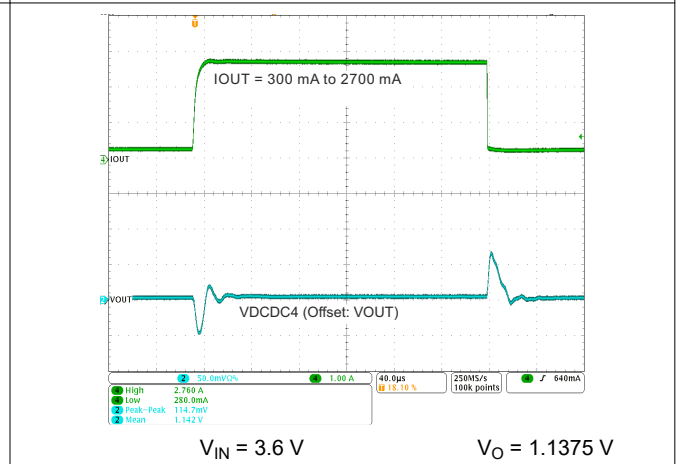
9-5. DCDC4 Load Transient Response
