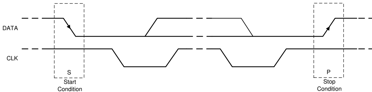
8-19. START and STOP Conditions
