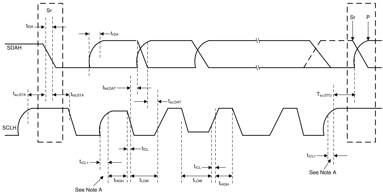
7-1. Serial Interface Timing Diagram for FS-Mode
