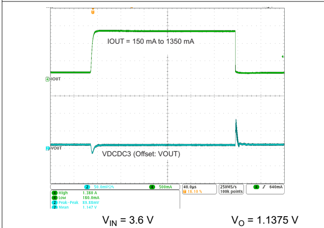
9-4. DCDC3 Load Transient Response
