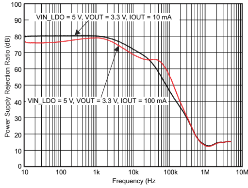
6-25. LDO4 PSRR vs Frequency
