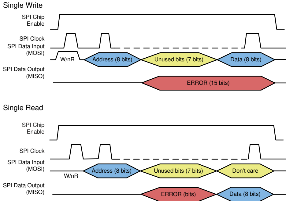
8-17. SPI READ and WRITE Protocol
