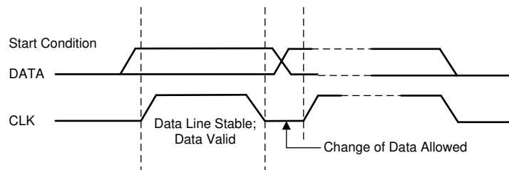
8-20. Bit Transfer on the Serial Interface
