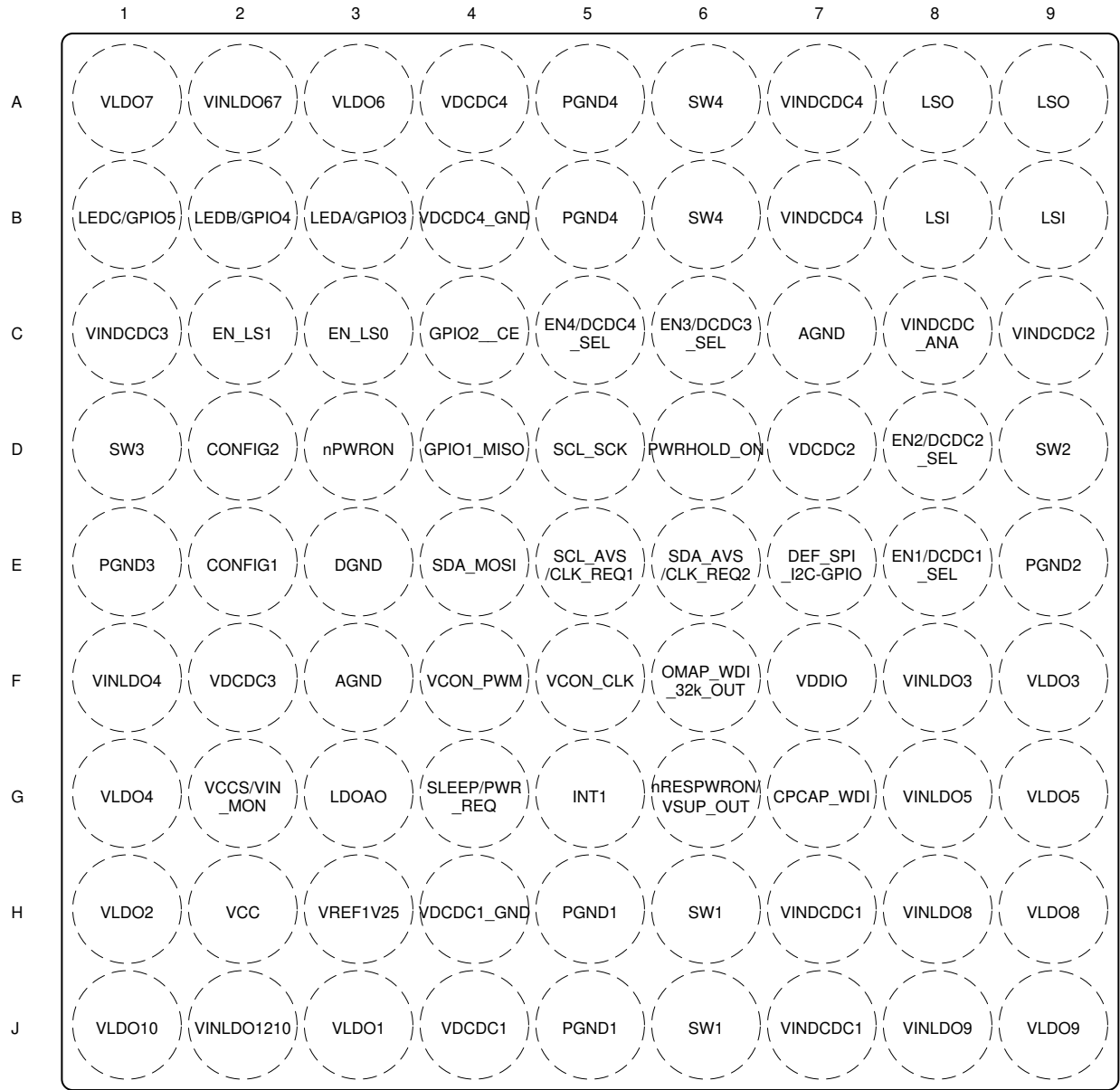
Figure 5-1. 81-Pin YFF DSBGA (Bottom View)
