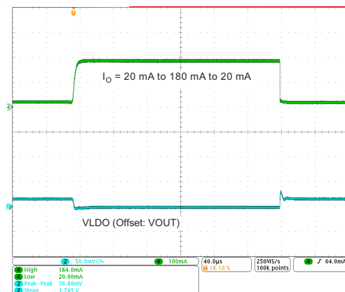
9-11. LDO1, LDO2, LDO3 Load Transient Response
