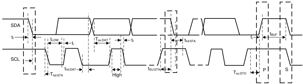
7-1. Serial Interface Timing Diagram for FS-Mode
