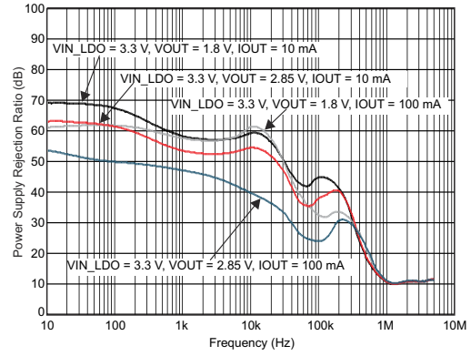
6-26. LDO6 and LDO8 PSRR vs Frequency
