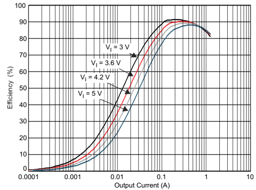
V_{OUT} = 1.8\text{ V} PWM Mode LQM2MPN-1R0 T_A = 25^\circ\text{C}
