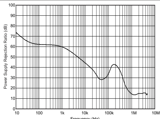
V_{IN} = 3.2\text{ V} V_{OUT} = 2.7\text{ V} I_{OUT} = 225\text{ mA} 6-24. LDO4 and LDO5 PSRR vs Frequency
