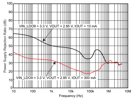
6-27. LDO9 PSRR vs Frequency
