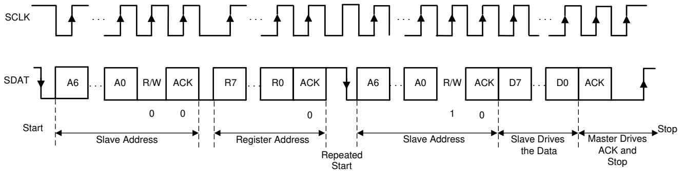
8-24. I 2 C Interface READ from TPS659128x; F/S Mode
