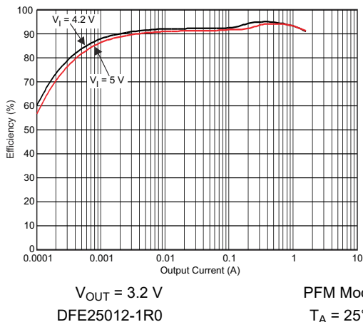
6-17. DCDC3 Efficiency vs Output Current
