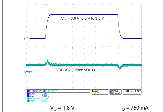
9-7. DCDC2 Line Transient Response
