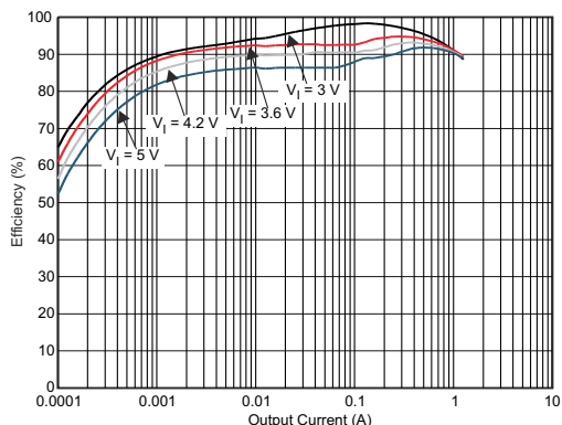
V_{OUT} = 2.95\text{ V} PFM Mode VLS201612-1R0 T_A = 25^\circ\text{C}
