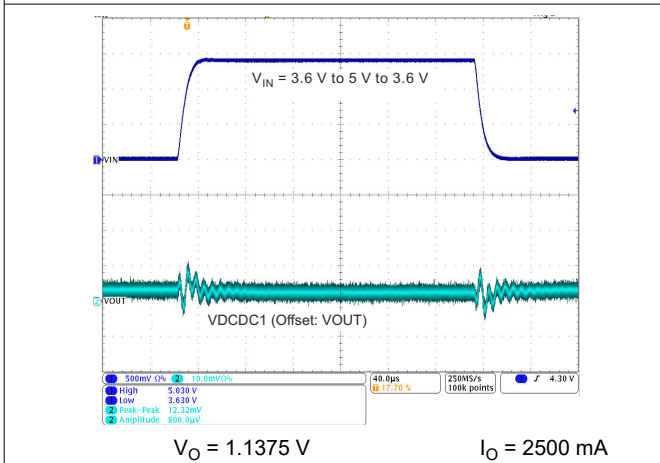
9-6. DCDC1 Line Transient Response
