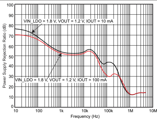
6-23. LDO1, LDO2, LDO3 PSRR vs Frequency
