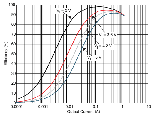
V_{OUT} = 2.95\text{ V} PWM Mode VLS201612-1R0 T_A = 25^\circ\text{C}
