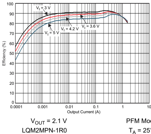
6-15. DCDC3 Efficiency vs Output Current
