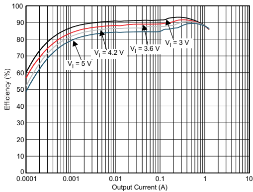
V_{OUT} = 2.25\text{ V} PFM Mode VLS201612-1R0 T_A = 25^\circ\text{C}
