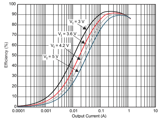
V_{OUT} = 2.25\text{ V} PWM Mode VLS201612-1R0 T_A = 25^\circ\text{C}
