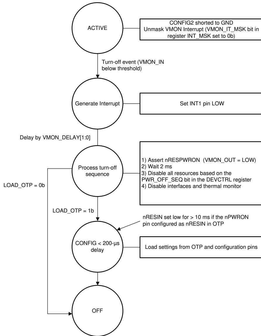
8-8. SHUTDOWN Flow for CONFIG2 Pin Shorted to GND
