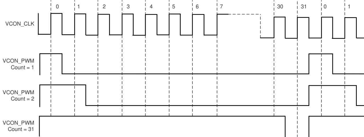
8-12. VCON Voltage Scaling Architecture
