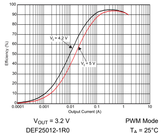
6-18. DCDC3 Efficiency vs Output Current
