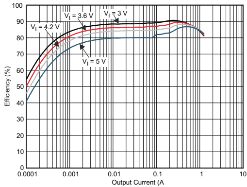
V_{OUT} = 1.8\text{ V} PFM Mode LQM2MPN-1R0 T_A = 25^\circ\text{C}
