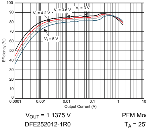
6-13. DCDC3 Efficiency vs Output Current
