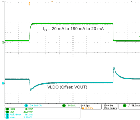
9-21. LDO7 Load Transient Response
