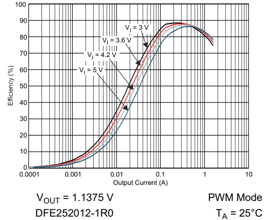
6-14. DCDC3 Efficiency vs Output Current
