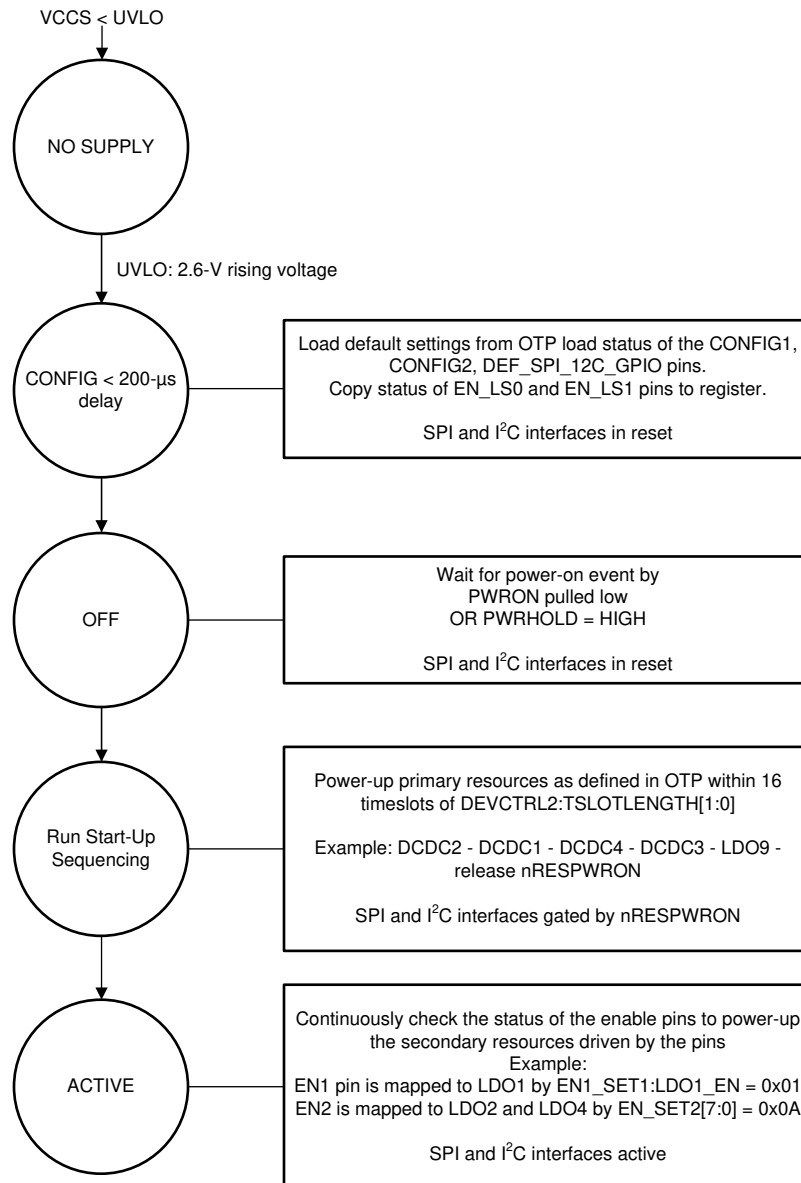
8-4. STARTUP Flow for CONFIG2 Pin Shorted to LDOAO
