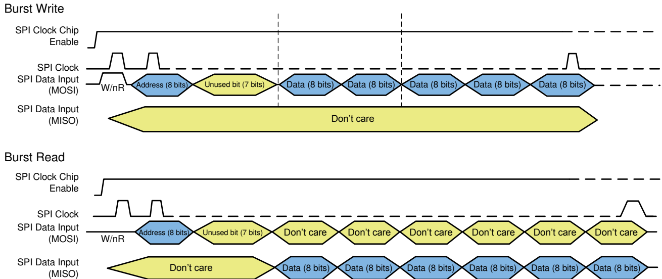
8-18. SPI BURST READ and BURST WRITE Protocol
