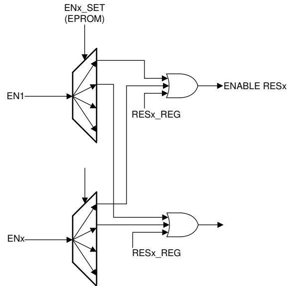
8-10. ENx Architecture
