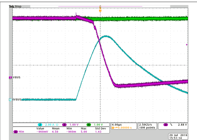
9-4. Px_VBUS Short with TVS2200 and Schottky Diode
