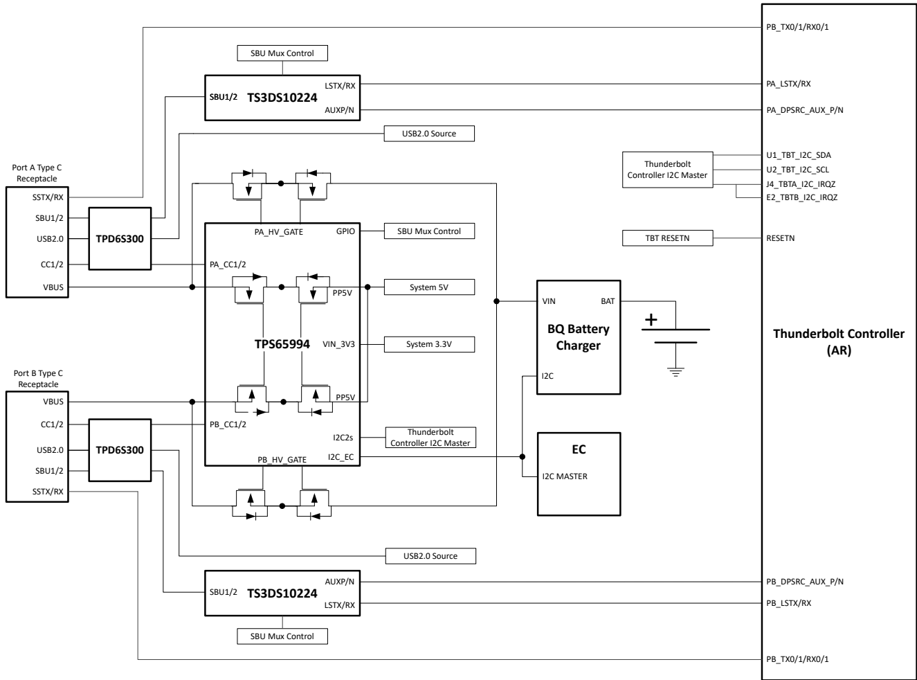
图 9-6. Thunderbolt Architecture
