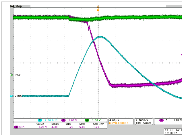
9-3. Px_VBUS Short with TVS2200, but Without Schottky Diode
