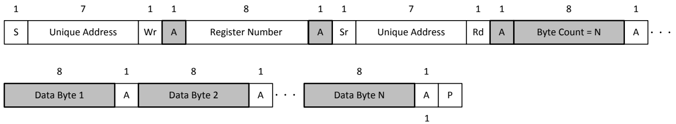
8-26. I²C Unique Address Read Register Protocol
