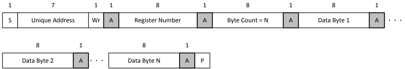
8-25. I²C Unique Address Write Register Protocol
