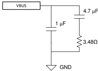
9-2. VBUS Snubber
