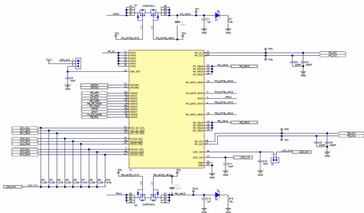
11-1. Example Schematic
