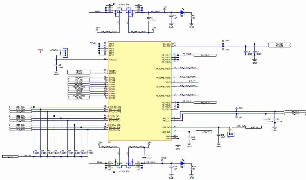
11-1. Example Schematic
