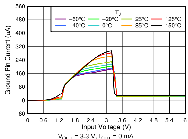
FIG 10. I_Q vs V_{IN}
