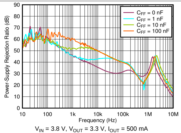
FIG 38. PSRR vs Frequency and C_{FF}
