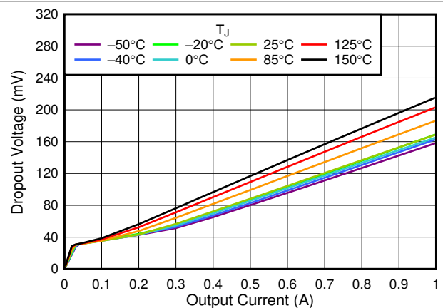
6-4. 3.3-V Dropout Voltage vs I_{OUT}
