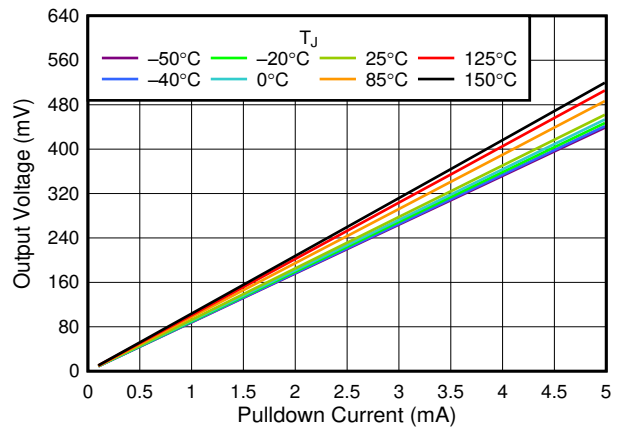
6-14. V_{OUT} vs I_{OUT} Pulldown Resistor
