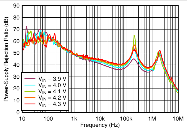
6-32. PSRR vs Frequency and V_{IN}
