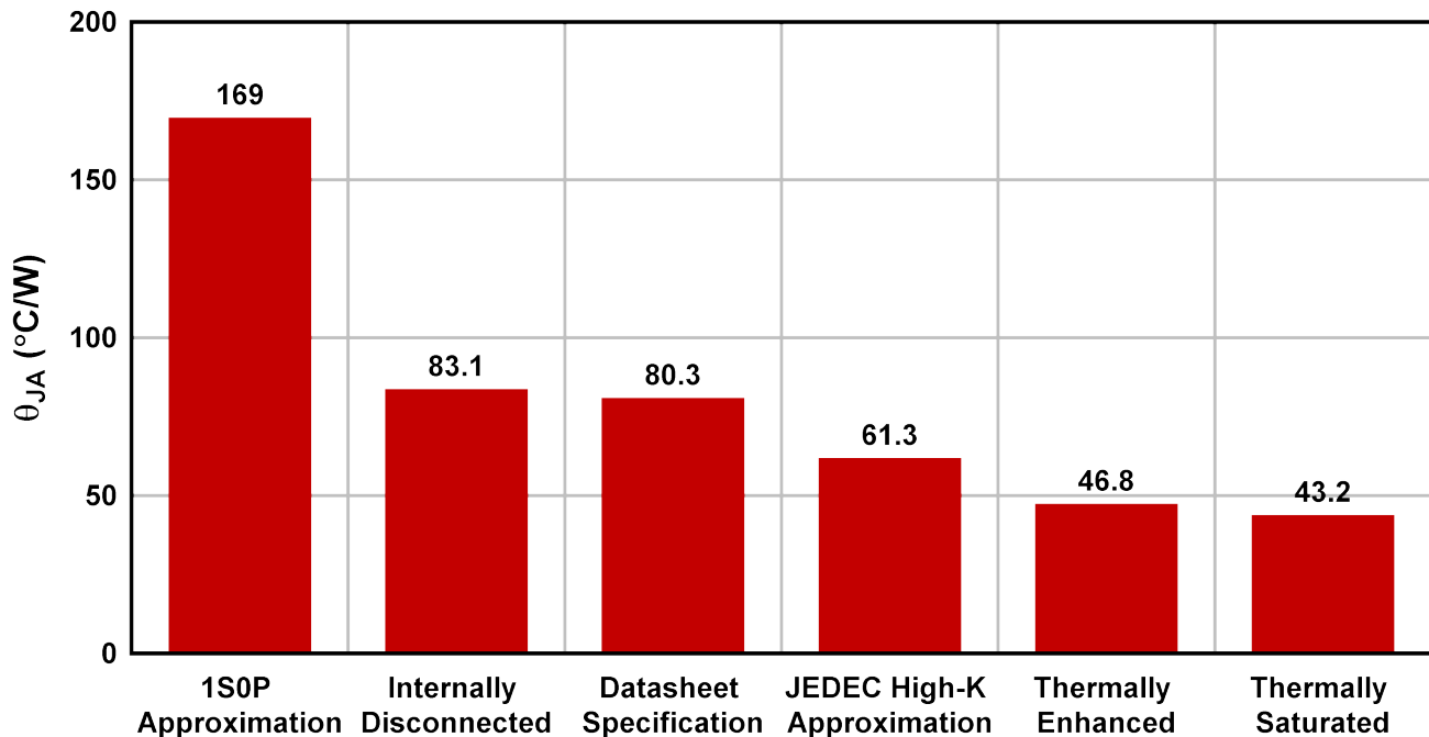
Figure 8-8. TPS746-Q1 (WSON) R_{\theta JA} vs Board Layout
