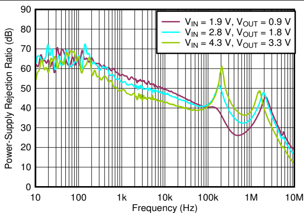
6-33. PSRR vs Frequency and V_{IN}
