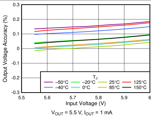
6-3. 5.5-V Line Regulation vs V_{IN}
