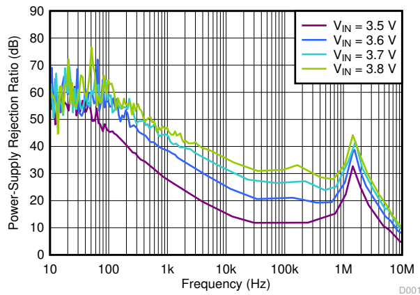
6-31. PSRR vs Frequency and V_{IN}
