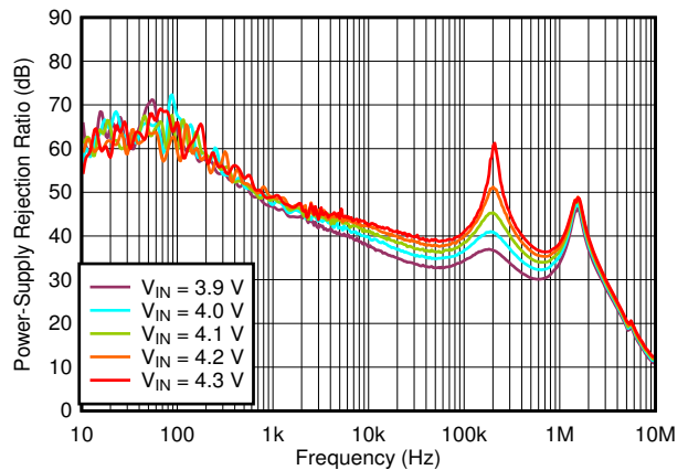
6-32. PSRR vs Frequency and V_{IN}
