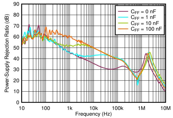
6-38. PSRR vs Frequency and C_{FF}
