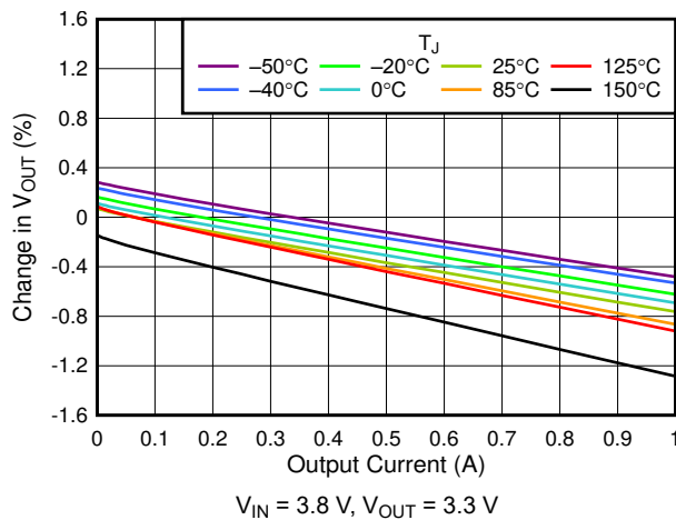
6-11. 3.3-V Load Regulation vs I_{OUT}
