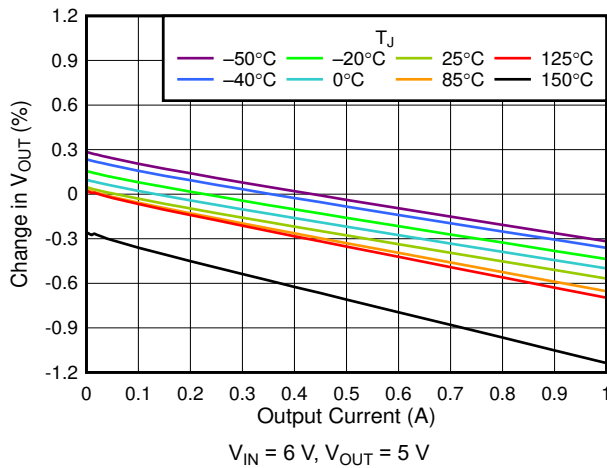
6-13. 5-V Load Regulation vs I_{OUT}
