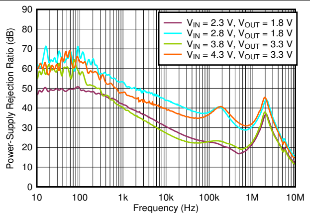
6-34. PSRR vs Frequency and V_{IN}
