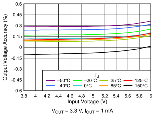
6-1. 3.3-V Line Regulation vs V_{IN}
