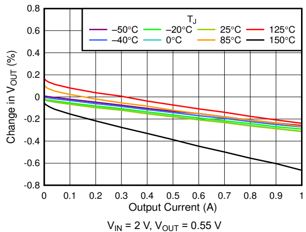
6-12. 0.55-V Load Regulation vs I_{OUT}
