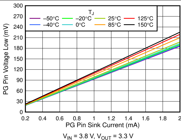
6-17. V_{OL(PG)} vs PG Pin Sink Current
