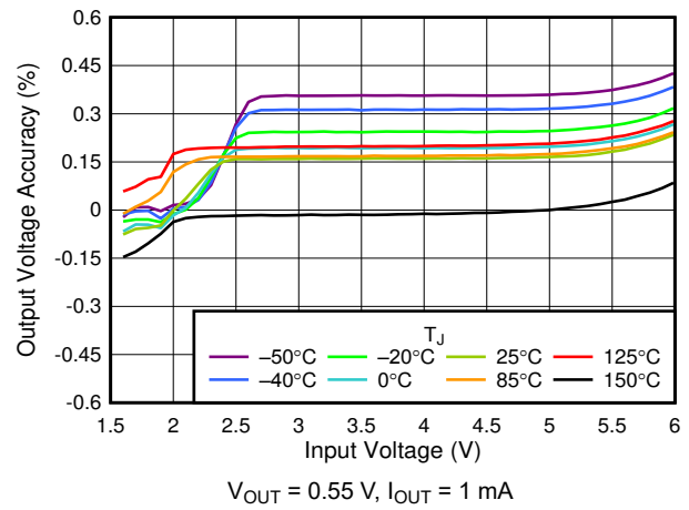
6-2. 0.55-V Line Regulation vs V_{IN}
