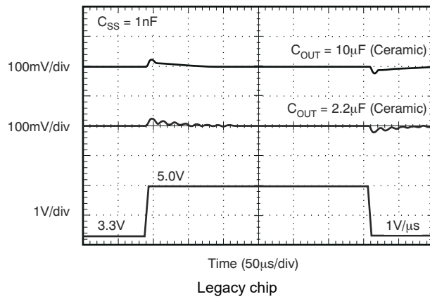
Figure 5-32. V_{BIAS} Line Transient
