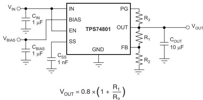
図 7-1. Typical Application Circuit for the TPS74801-Q1 (Adjustable)
