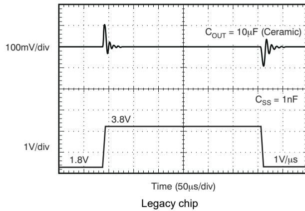
Figure 5-34. V_{IN} Line Transient
