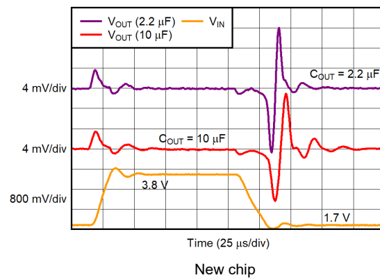
Figure 5-35. V_{IN} Line Transient
