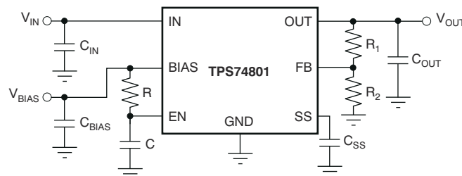
図 6-3. Soft-Start Delay Using an RC Circuit to Enable the Device
