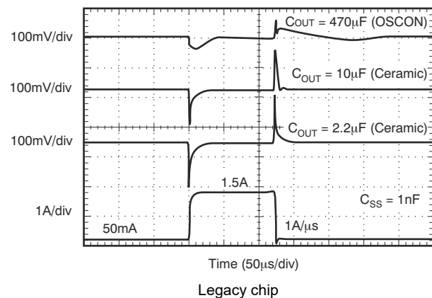
Figure 5-36. Output Load Transient Response
