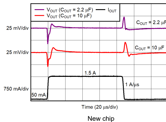
Figure 5-37. Output Load Transient Response
