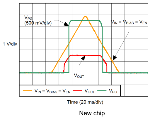
Figure 5-41. Power-Up, Power-Down
