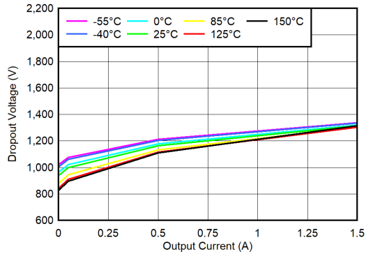
5-13. V_{BIAS} Dropout Voltage vs I_{OUT} and Temperature ( T_J )
