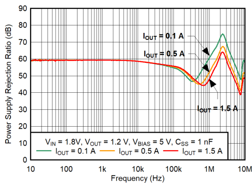
5-15. V_{BIAS} PSRR vs Frequency
