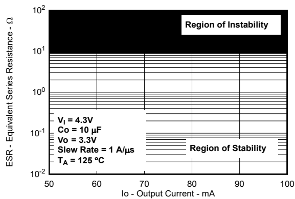
5-58. Typical Region of Stability ESR vs Output Current (New Chip)
