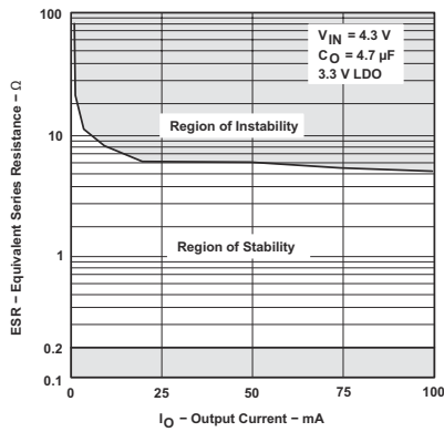
5-46. TPS76933-Q1 Typical Regions of Stability ESR vs Output Current (Legacy Chip)
