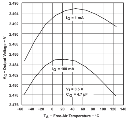
図 5-7. TPS76925-Q1 Output Voltage vs Free-Air Temperature (Legacy Chip)
