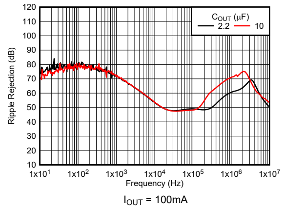
図 5-32. TPS76933-Q1 Ripple Rejection vs Output Capacitor (New Chip)
