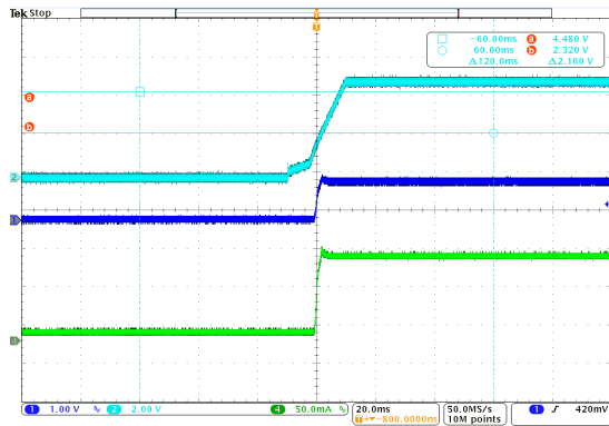
7-4. Power-Up Waveform (Legacy Chip)
