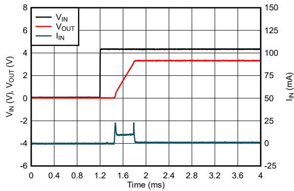
7-4. Power-Up Waveform (Legacy Chip)
