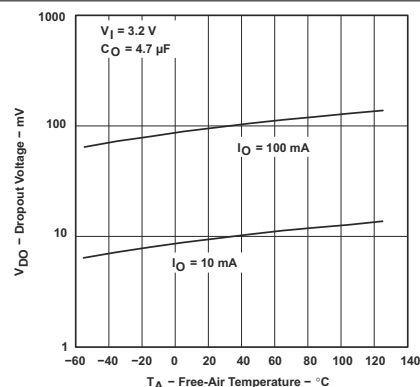
図 5-26. TPS76933-Q1 Dropout Voltage vs Free-Air Temperature (Legacy Chip)
