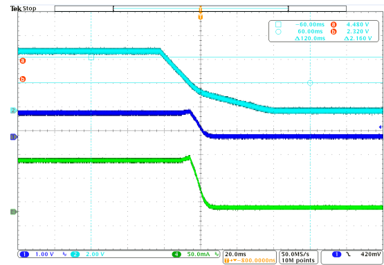
7-5. Power-Down Waveform (Legacy Chip)
