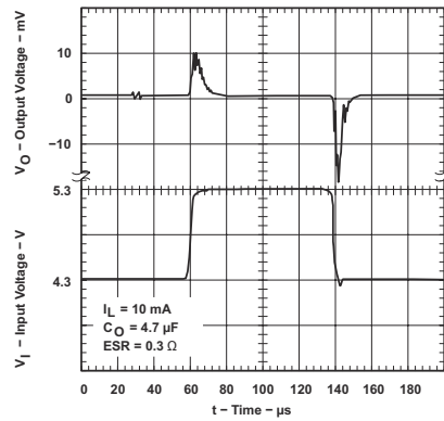
図 5-37. TPS76915-Q1 Line Transient Response (Legacy Chip)
