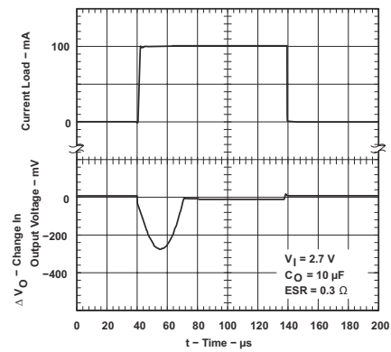
7-9. TPS76915-Q1 Load Transient Response (Legacy Chip)
