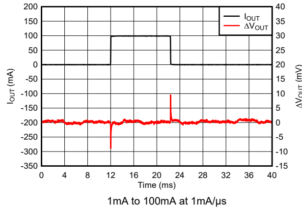
図 7-16. TPS76933-Q1 Load Transient Response (New Chip)
