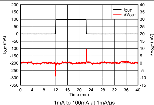
図 5-45. TPS76933-Q1 Load Transient Response (New Chip)
