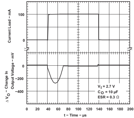
図 5-38. TPS76915-Q1 Load Transient Response (Legacy Chip)
