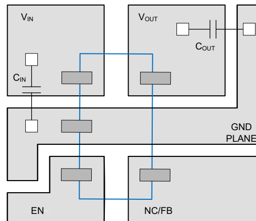
図 7-17. Layout Recommendation
