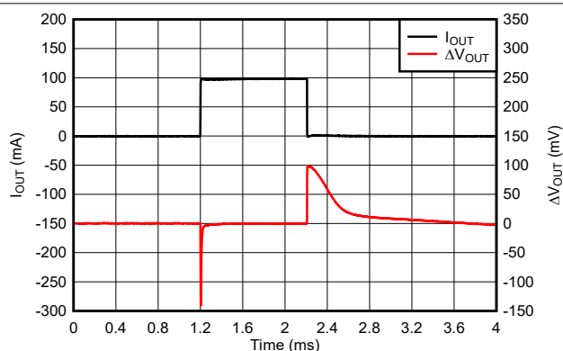
図 5-44. TPS76933-Q1 Load Transient Response (New Chip)
