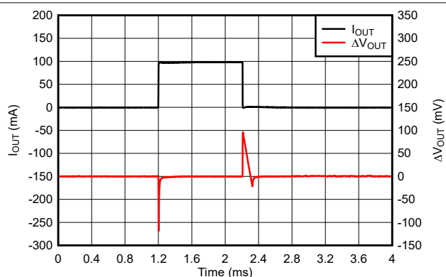
図 5-43. TPS76933-Q1 Load Transient Response (New Chip)
