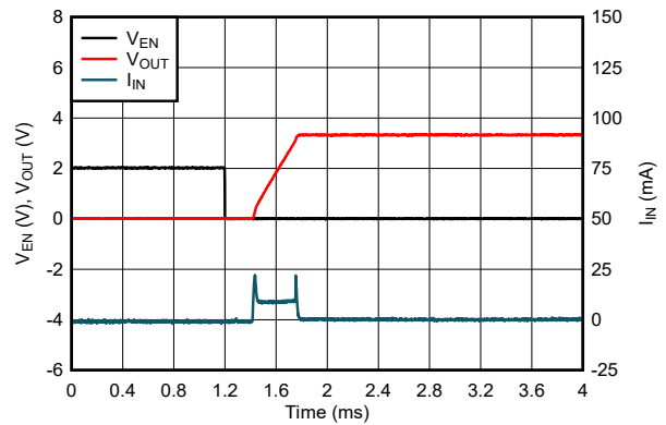
図 5-36. LDO Start-Up Time With EN (New Chip)
