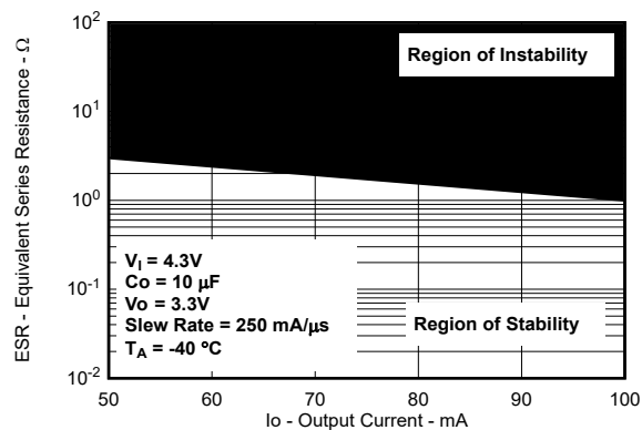
5-65. Typical Region of Stability ESR vs Output Current (New Chip)
