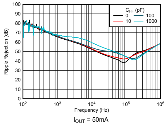
図 5-33. TPS76901-Q1 Ripple Rejection vs Feed-Forward Capacitor (New Chip)
