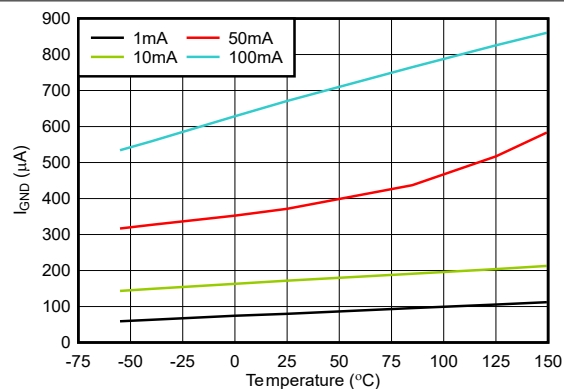
図 5-13. TPS76933-Q1 Ground Current vs Free-Air Temperature (New Chip)
