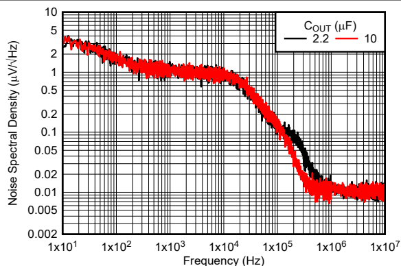
図 5-21. TPS76933-Q1 Output Spectral Noise Density vs Frequency (Legacy Chip)
