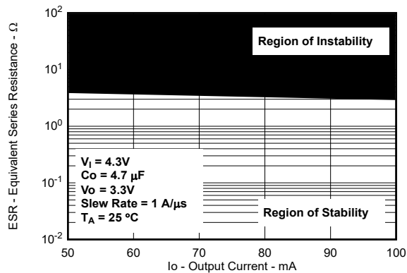
5-48. TPS76933-Q1 Typical Regions of Stability ESR vs Output Current (Legacy Chip)
