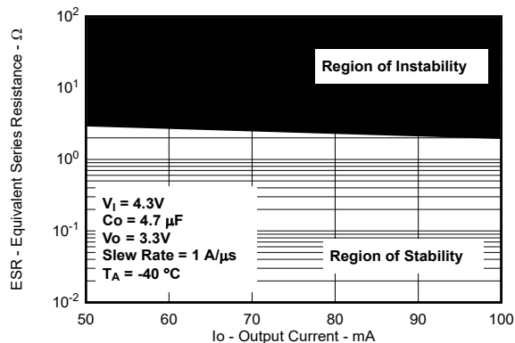
5-60. Typical Region of Stability ESR vs Output Current (New Chip)
