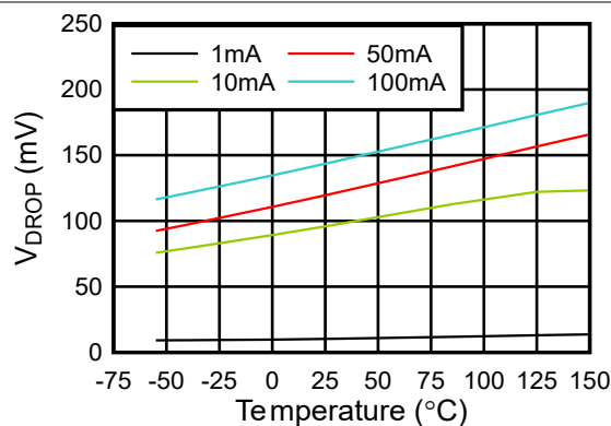
図 5-27. TPS76933-Q1 Dropout Voltage vs Free-Air Temperature (New Chip)
