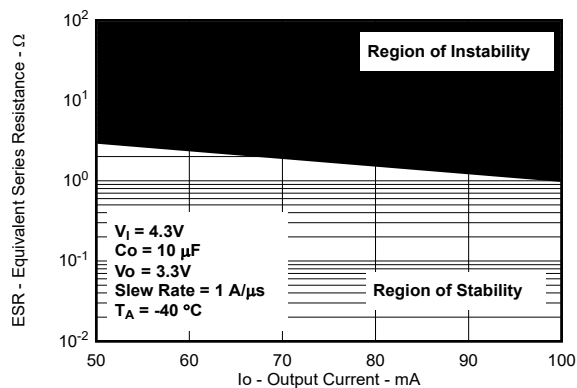
5-64. Typical Region of Stability ESR vs Output Current (New Chip)
