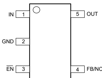
図 4-1. DBV Package, 5-Pin SOT-23 (Top View)
