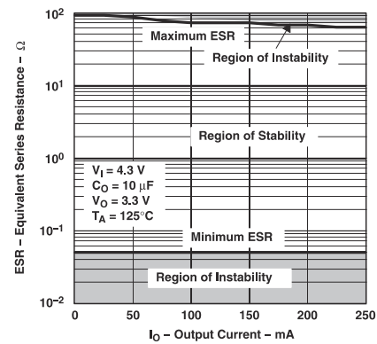
5-59. Typical Region of Stability ESR vs Output Current (Legacy Chip)
