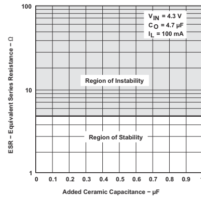
5-47. TPS76933-Q1 Typical Regions of Stability ESR vs Added Ceramic Capacitance (Legacy Chip)
