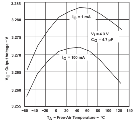
図 5-8. TPS76933-Q1 Output Voltage vs Free-Air Temperature (Legacy Chip)
