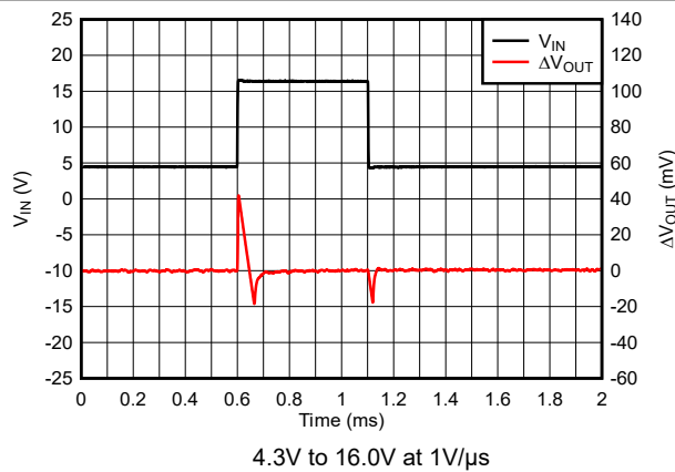
図 5-41. TPS76933-Q1 Line Transient Response (New Chip)
