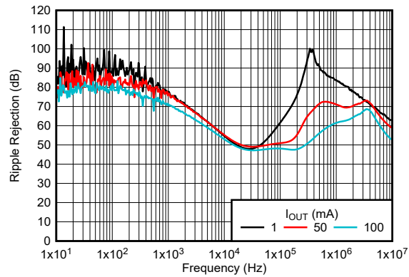
図 5-31. TPS76933-Q1 Ripple Rejection vs Output Current (New Chip)
