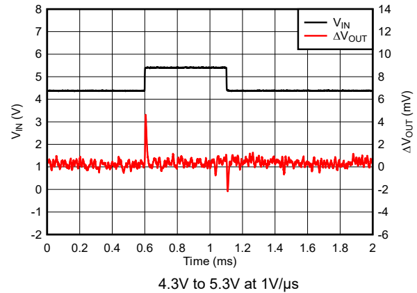
図 5-40. TPS76933-Q1 Line Transient Response (New Chip)
