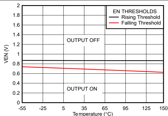
図 5-19. TPS76933-Q1 EN Threshold vs Free-Air Temperature (New Chip)
