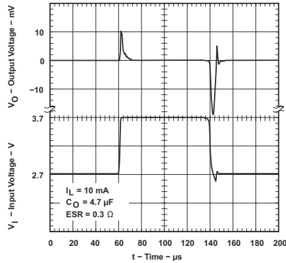
図 5-37. TPS76915-Q1 Line Transient Response (Legacy Chip)
