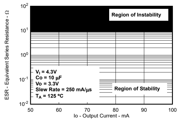
5-59. Typical Region of Stability ESR vs Output Current (Legacy Chip)
