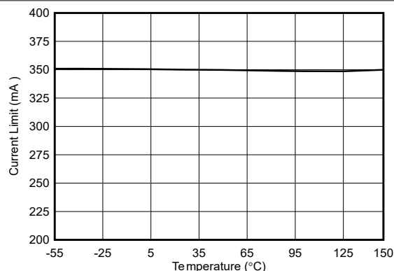
図 5-20. TPS76933-Q1 Current Limit vs Free-Air Temperature (New Chip)
