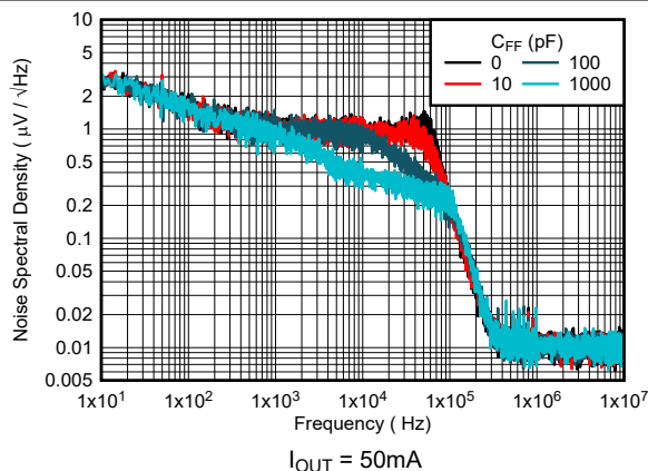
図 5-24. TPS76901-Q1 Output Spectral Noise Density vs Feed-Forward Capacitor (New Chip)
