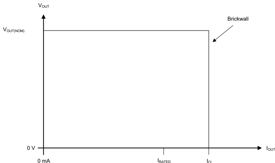
☒ 6-5. Current Limit
