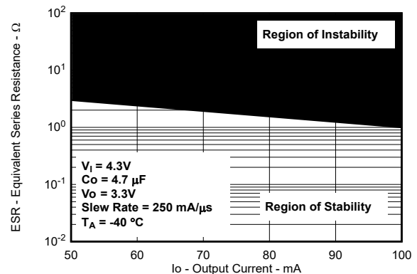
5-61. Typical Region of Stability ESR vs Output Current (New Chip)
