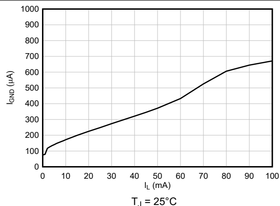
図 5-14. TPS76933-Q1 Ground Current vs Output Current (New Chip)
