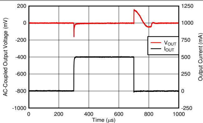
FIG 6-23. I_{OUT} Transient
