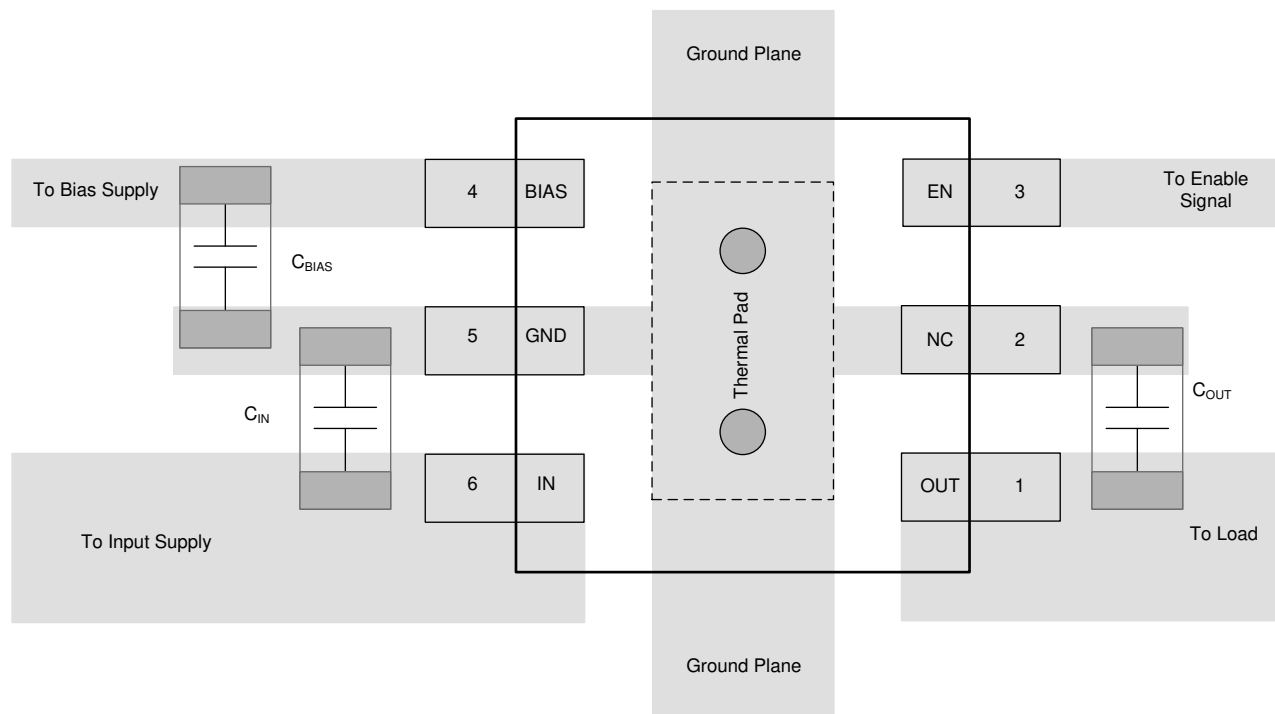
10-2. Recommended Layout for DRV Package
