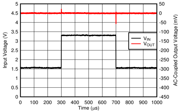
FIG 6-19. V_{IN} Transient
