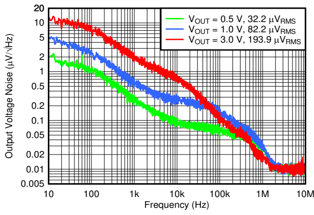
6-29. Output Noise vs Frequency and V_{OUT}
