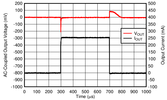
FIG 6-20. I_{OUT} Transient
