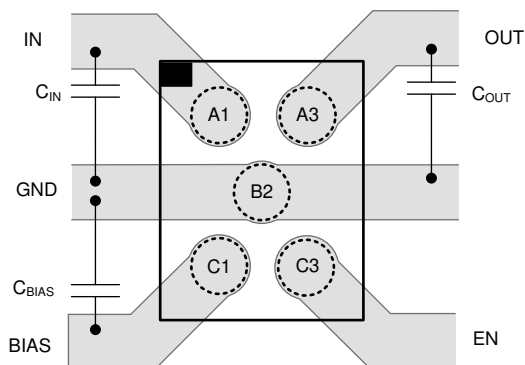
10-1. Recommended Layout for YKA Package
