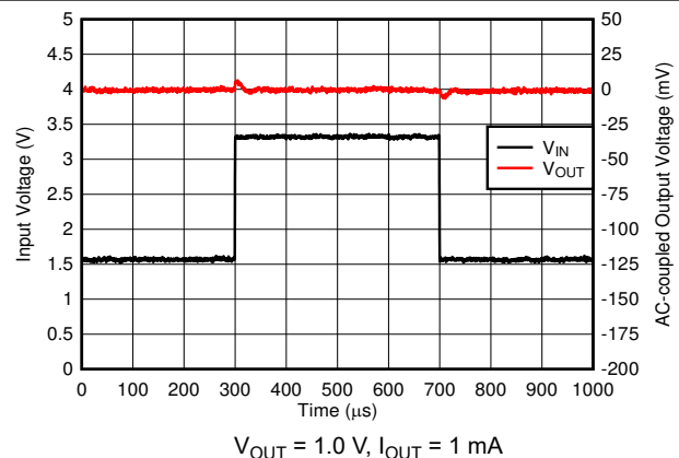
Figure 6-18. V_{IN} Transient
