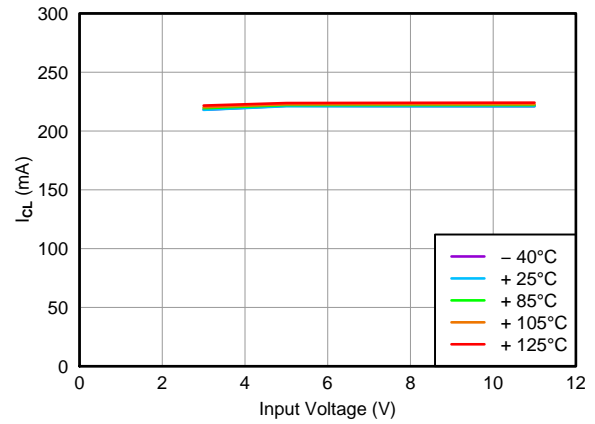
8. Current Limit vs Input Voltage
