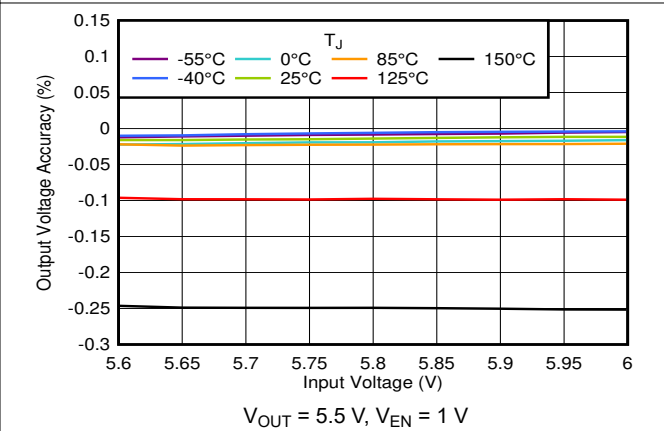
图 5-12. Output Voltage Accuracy vs V_{IN}
