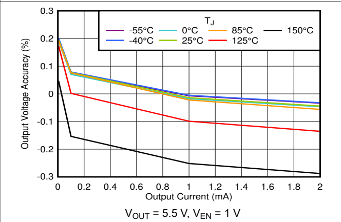
图 5-10. Output Voltage Accuracy vs I_{OUT}
