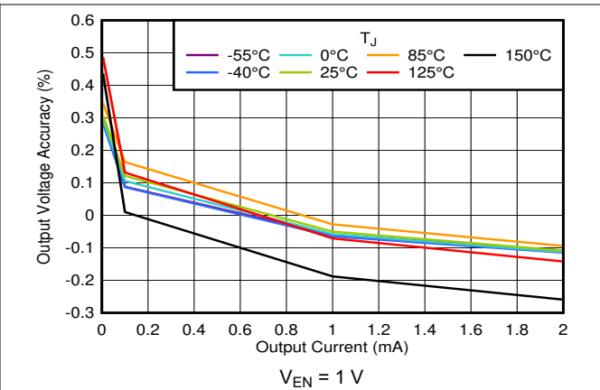
图 5-8. Output Voltage Accuracy vs I_{OUT}
