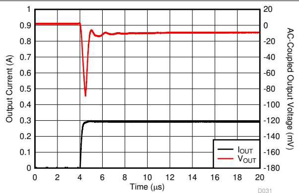
5-36. Load Transient
