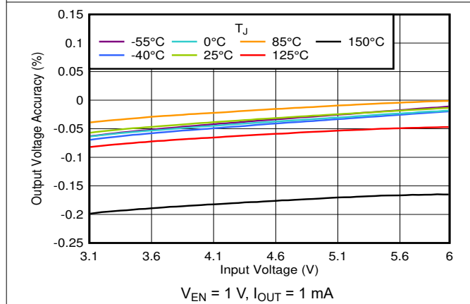
图 5-11. Output Voltage Accuracy vs V_{IN}
