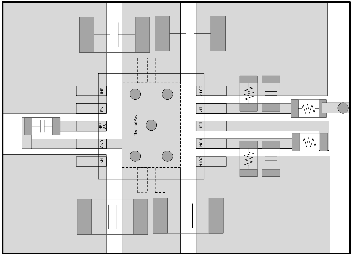
☒ 81. Layout Example for Adjustable Option
