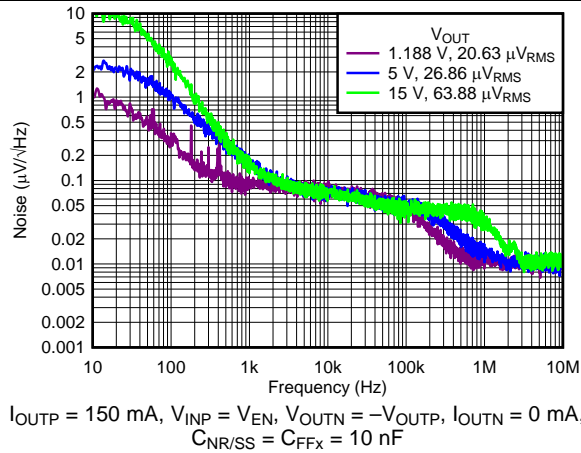
Fig 14. Positive Spectral Noise Density vs Frequency and V_{OUTP}
