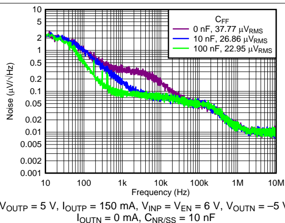
Fig 18. Positive Spectral Noise Density vs Frequency and C_{FFP}
