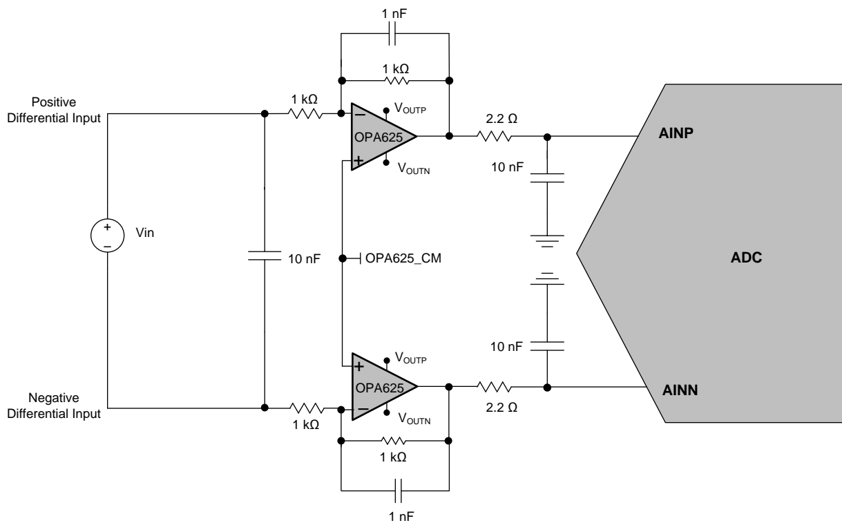
☒ 78. Creating Power Rails for an Analog Front-End of an ADC
