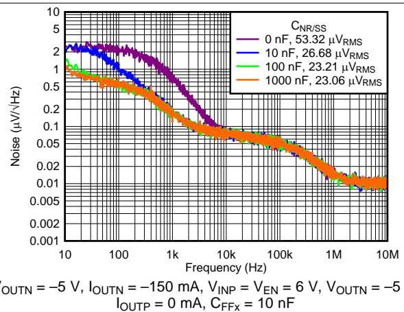
Fig 17. Negative Spectral Noise Density vs Frequency and C_{NR/SS}
