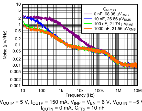
Fig 16. Positive Spectral Noise Density vs Frequency and C_{NR/SS}
