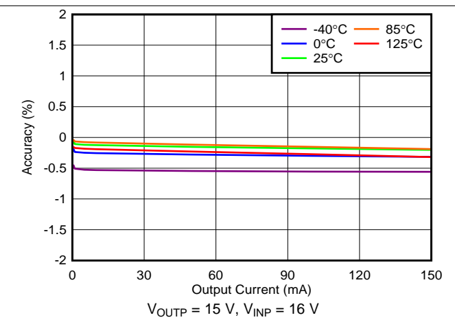
图 41. Positive Load Regulation
