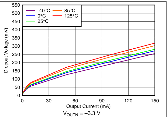
图 51. Negative Regulator Dropout Voltage vs Output Current
