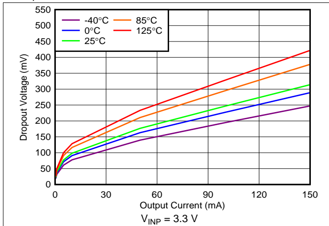
图 50. Positive Regulator Dropout Voltage vs Output Current
