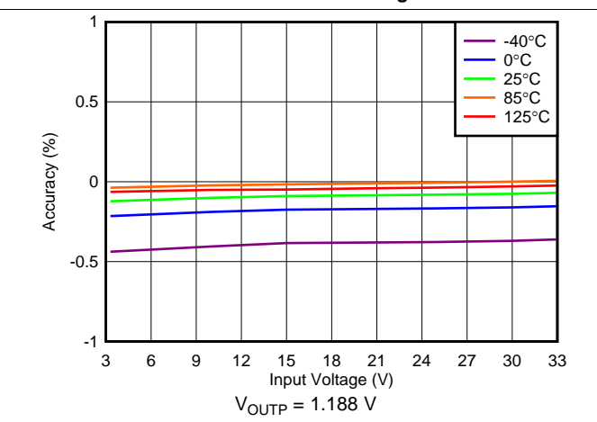
图 43. Positive Line Regulation
