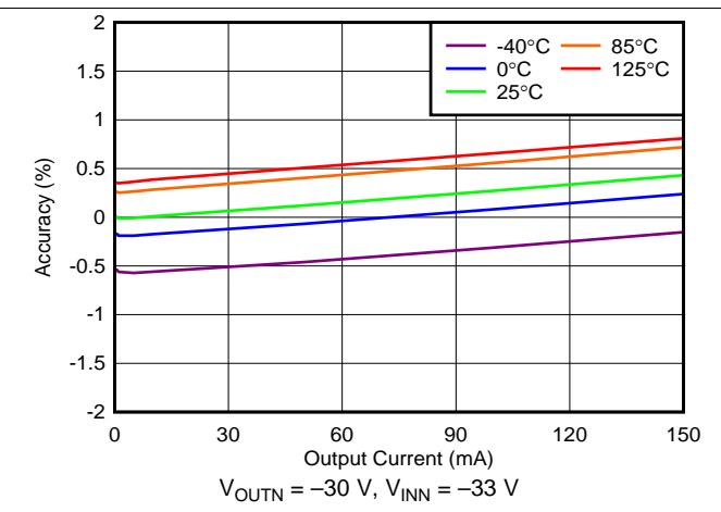
图 39. Negative Load Regulation
