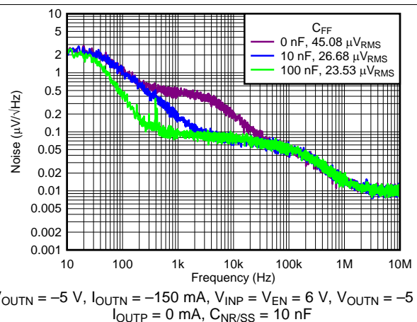
Fig 19. Negative Spectral Noise Density vs Frequency and C_{FFN}
