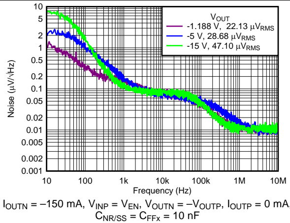
Fig 15. Negative Spectral Noise Density vs Frequency and V_{OUTN}
