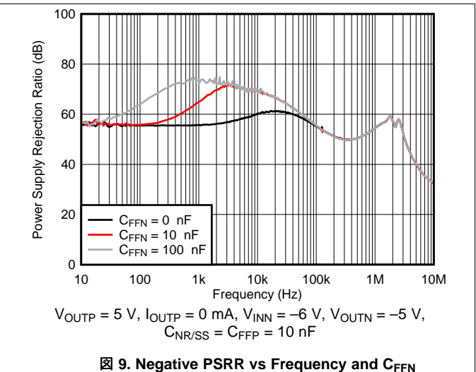
9. Negative PSRR vs Frequency and C_{FFN}
