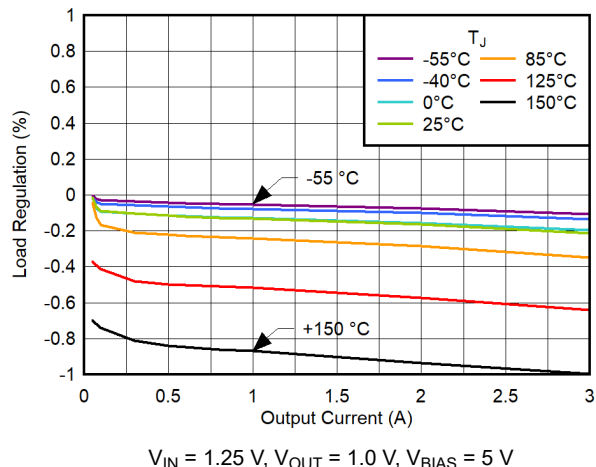
6-22. Load Regulation vs \geq 50\text{-mA} Output Current
