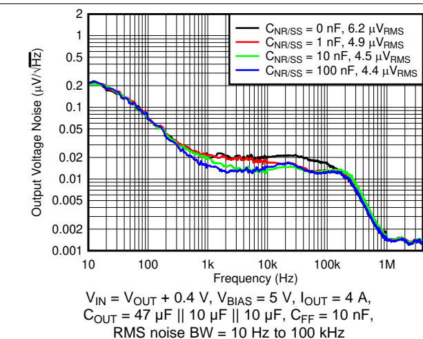
图 12. Output Noise vs Frequency and C_{NR/SS}
