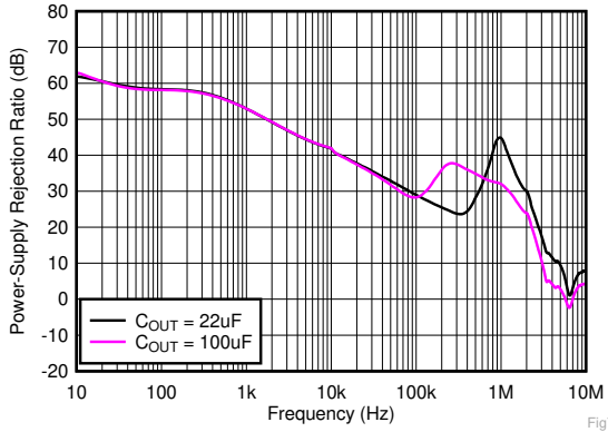
7-7. PSRR vs Frequency and C_{OUT}
