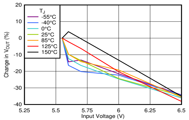
7-54. Line Regulation vs V_{IN}
