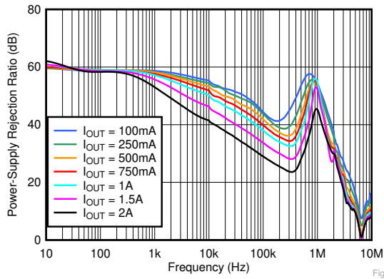
Fig 7-1. PSRR vs Frequency and I_{OUT}
