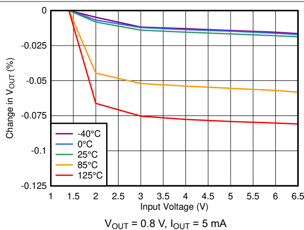
7-29. Line Regulation
