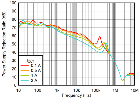
7-43. PSRR vs Frequency and I_{OUT}
