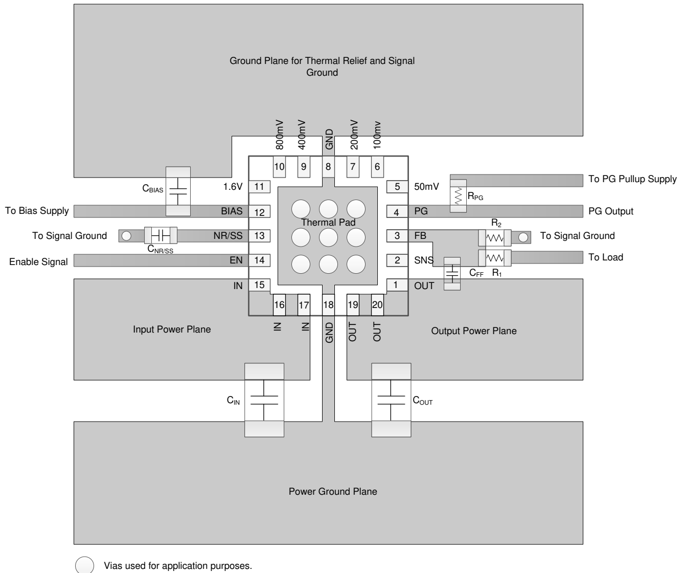
Figure 11-1. Example Layout
