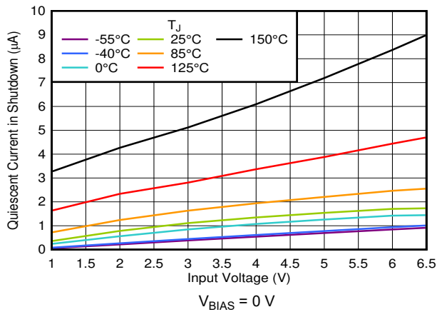
7-59. Shutdown Current vs Input Voltage
