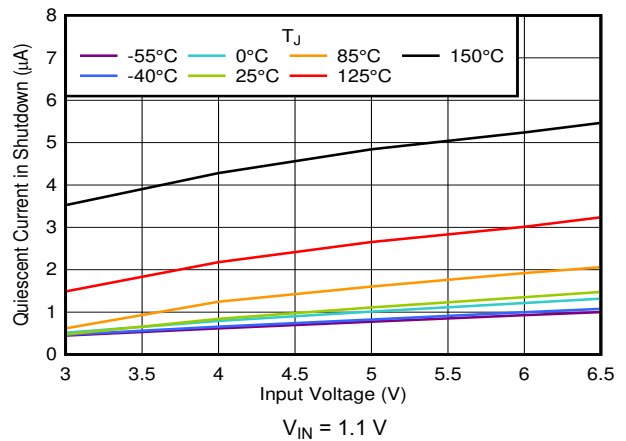
7-60. Shutdown Current vs Bias Voltage
