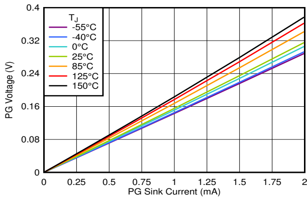
7-65. PG Voltage vs PG Current Sink
