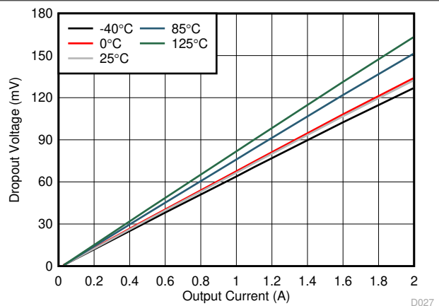
7-22. Dropout Voltage vs Output Current Without BIAS
