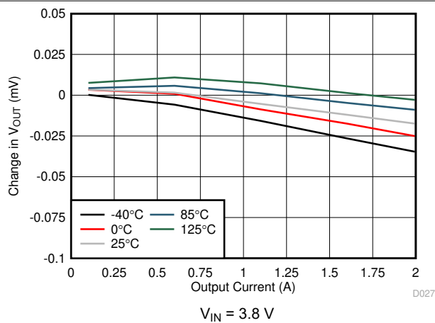
7-27. Load Regulation (3.3-V Output)
