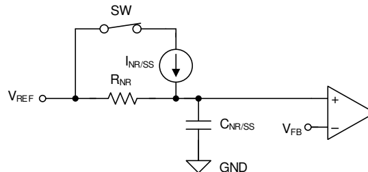
☒ 8-2. Simplified Soft-Start Circuit
