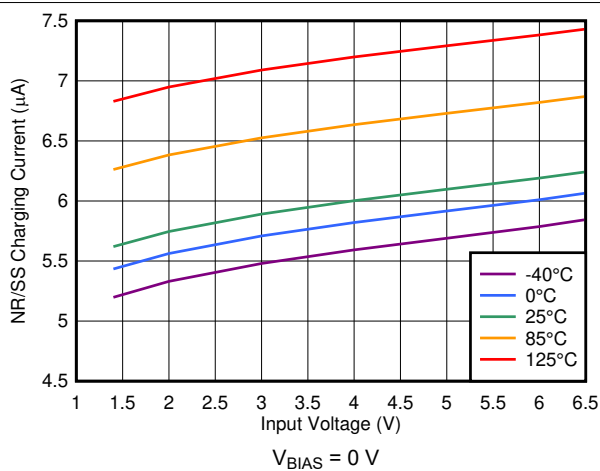
7-36. I_{NR/SS} Current vs Input Voltage
