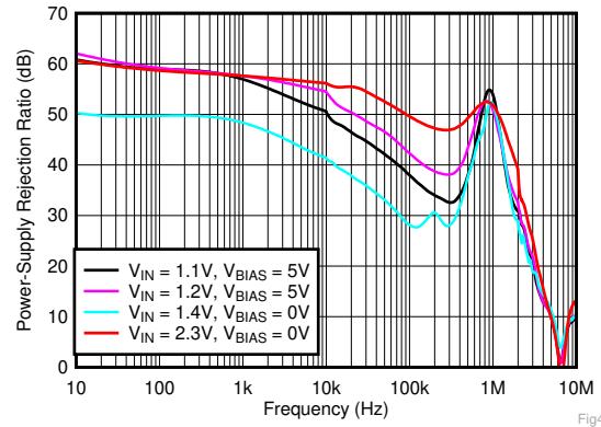
Fig 7-2. PSRR vs Frequency and V_{IN} With BIAS
