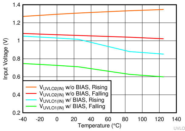
7-37. V_{IN} UVLO vs Temperature
