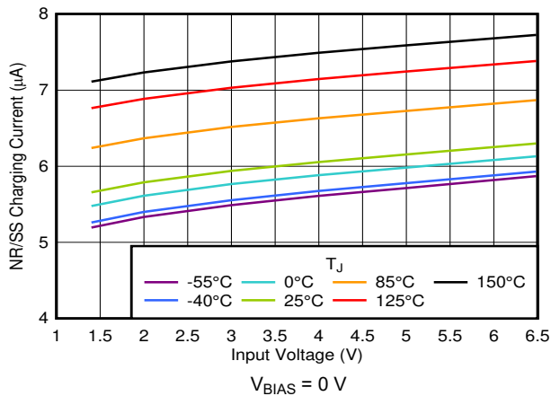
7-61. I_{NR/SS} Current vs Input Voltage
