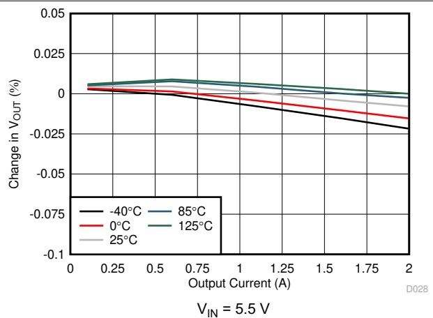
7-28. Load Regulation (5-V Output)
