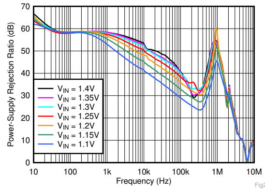
Fig 7-2. PSRR vs Frequency and V_{IN} With BIAS
