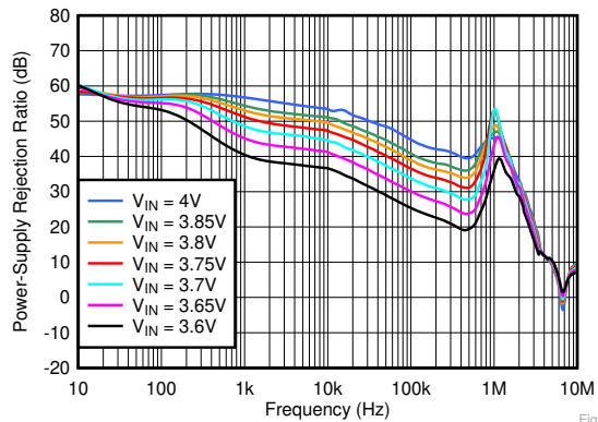
Fig 7-4. PSRR vs Frequency and V_{IN}
