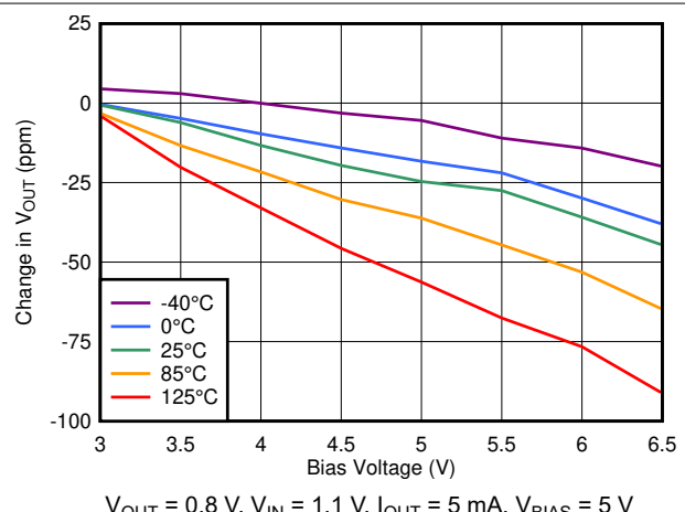
7-30. Line Regulation With BIAS
