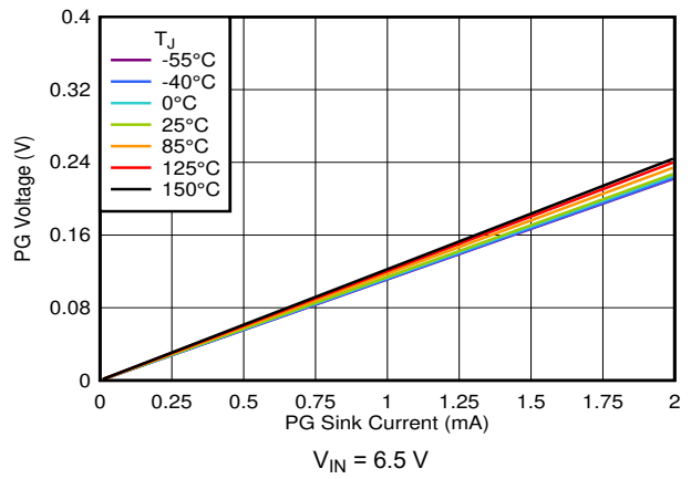
7-66. PG Voltage vs PG Current Sink
