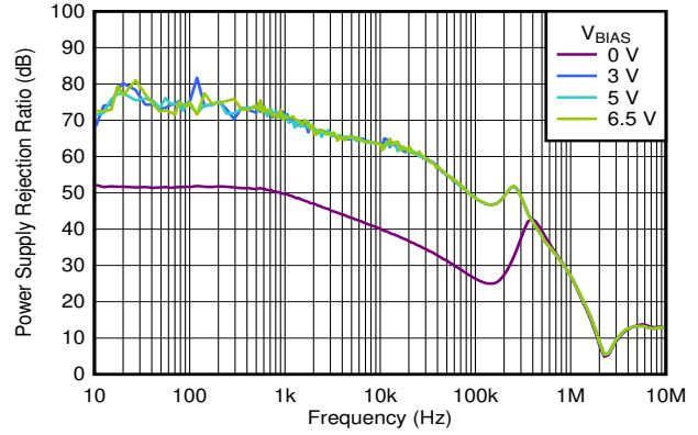
7-44. PSRR vs Frequency and V_{BIAS}
