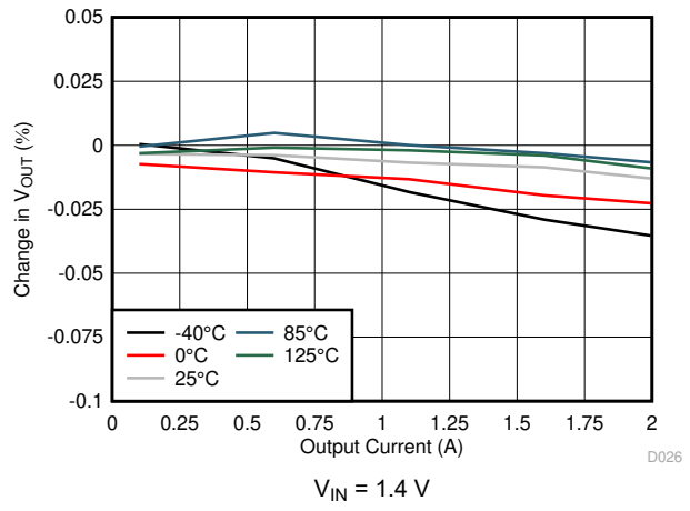
7-26. Load Regulation
