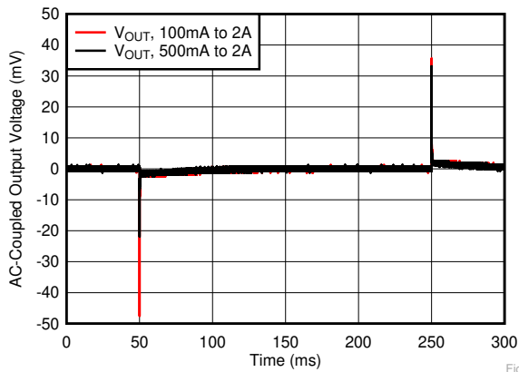
7-19. Load Transient vs Time and DC Load
